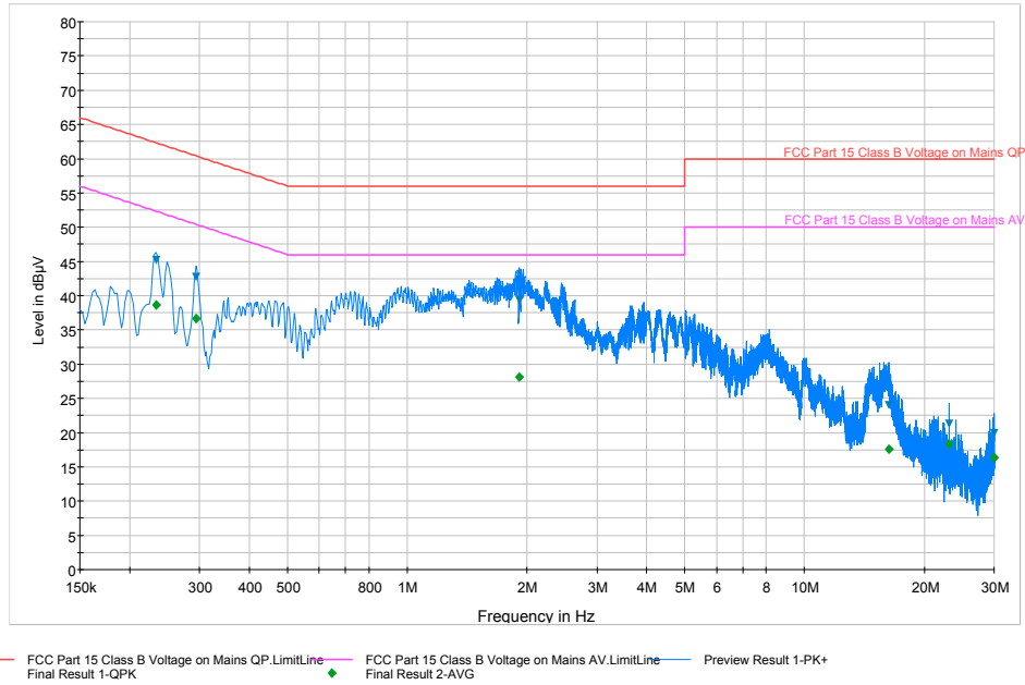
Plot 6-18. Line Conducted Plot with Bluetooth LE (L1)
