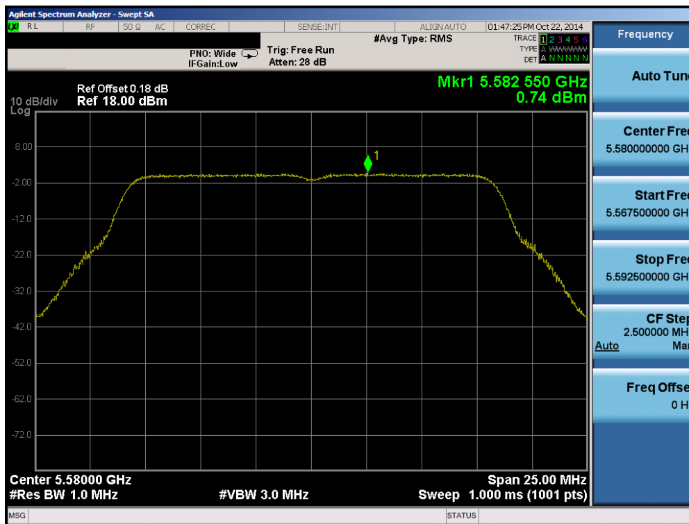
Plot 6-58. Peak Power Spectral Density Plot (802.11a (UNII Band 2C) – Ch. 116)
