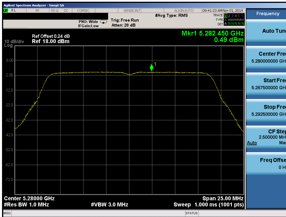
Plot 6-52. Peak Power Spectral Density Plot (20MHz BW 802.11n (UNII Band 2A) – Ch. 56)
