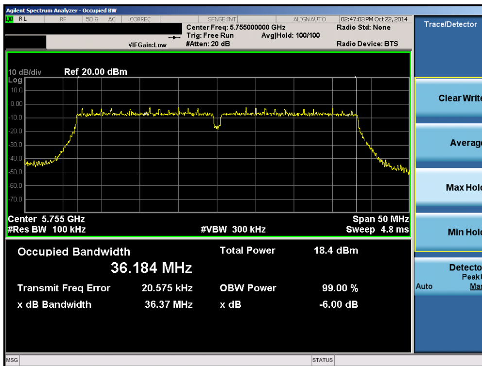
Plot 6-36. 6dB Bandwidth Plot (40MHz BW 802.11n (UNII Band 3) – Ch. 151)
