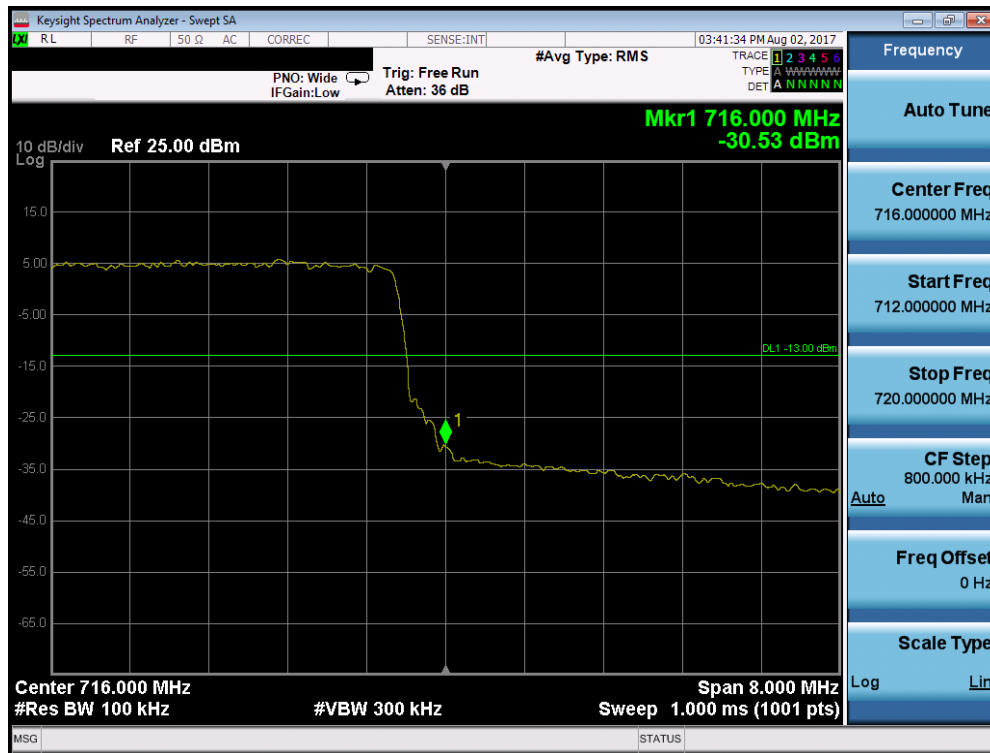
Plot 7-103. Upper Band Edge Plot (Band 12 – 10.0MHz QPSK – RB Size 50)
