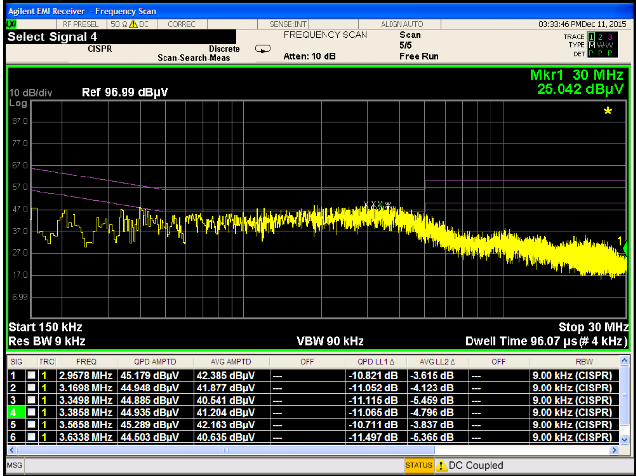
Plot 7-22. Line Conducted Plot with Bluetooth LE (L1) – Travel Adapter S/N EAY64329102
