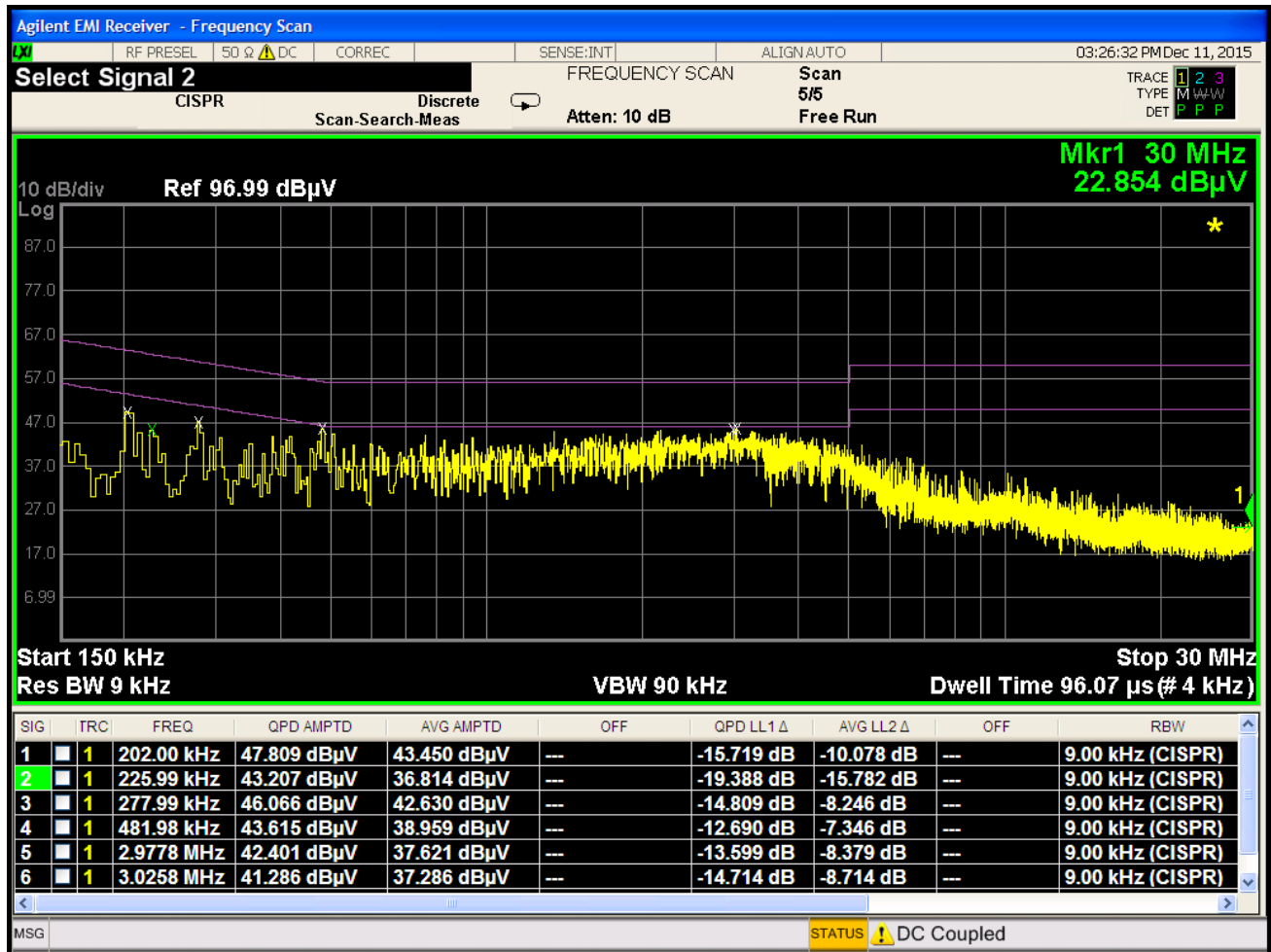
Plot 7-23. Line Conducted Plot with Bluetooth LE (N) – Travel Adapter S/N EAY64329102
