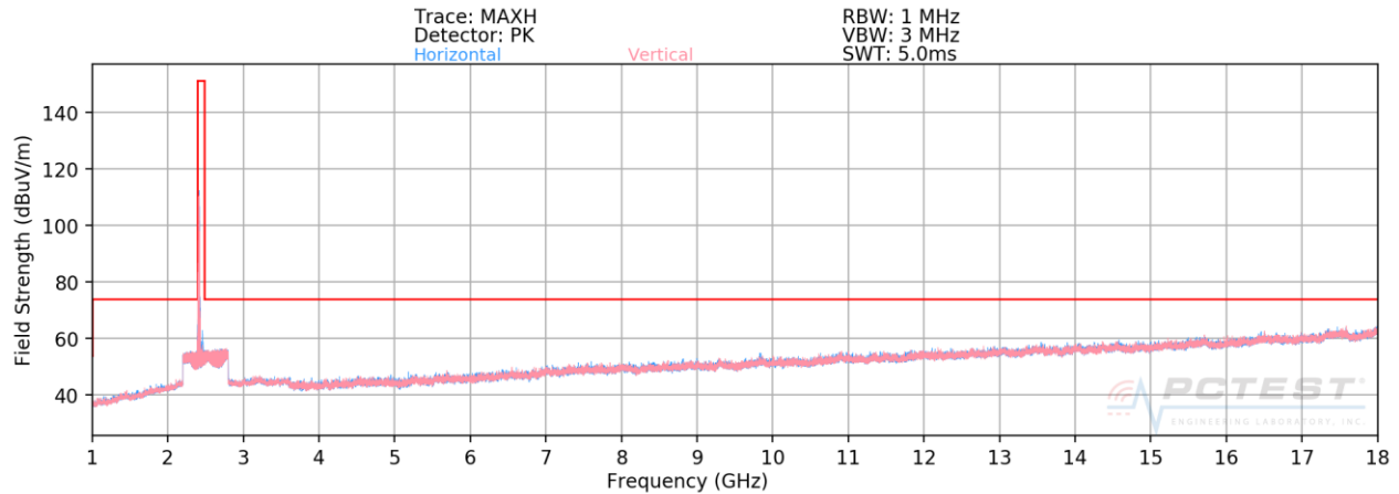
Plot 7-31. Radiated Spurious Plot above 1GHz ANT1 (802.11b – Ch. 1)
