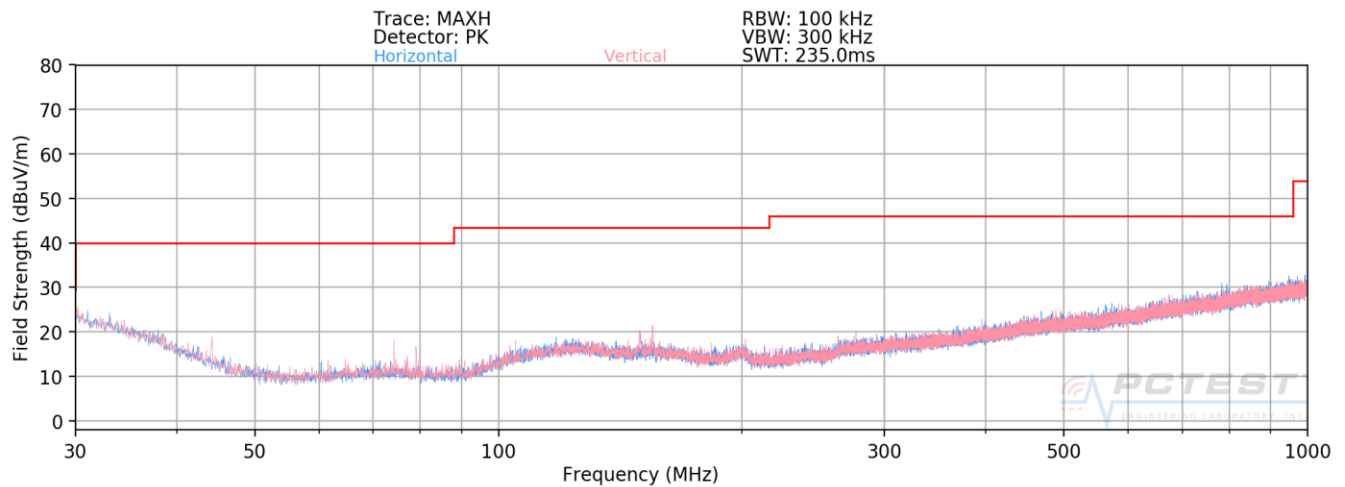
Plot 7-39. Radiated Spurious Plot below 1GHz
