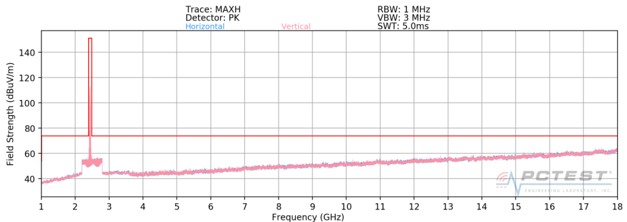
Plot 7-32. Radiated Spurious Plot above 1GHz ANT1 (802.11b – Ch. 6)
