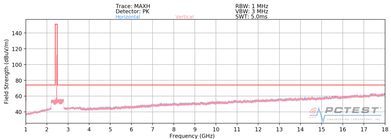
Plot 7-33. Radiated Spurious Plot above 1GHz ANT1 (802.11b – Ch. 11)
