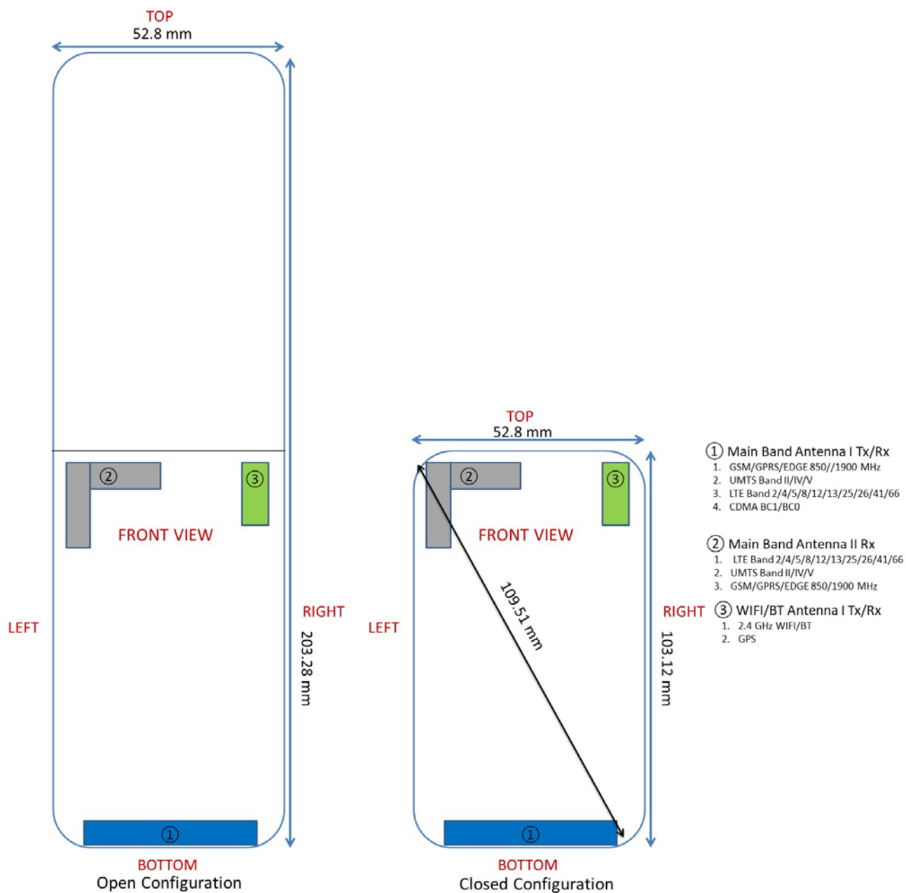
Figure E-1 DUT Antenna Locations
