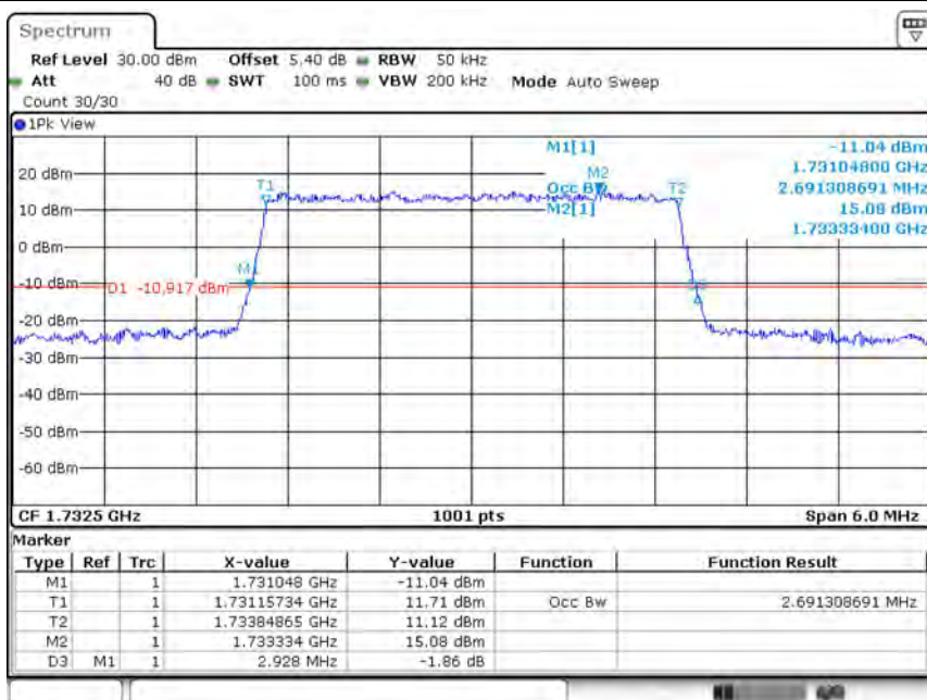
Band4-3MHz-QPSK-20175-15RB#0-2.691
