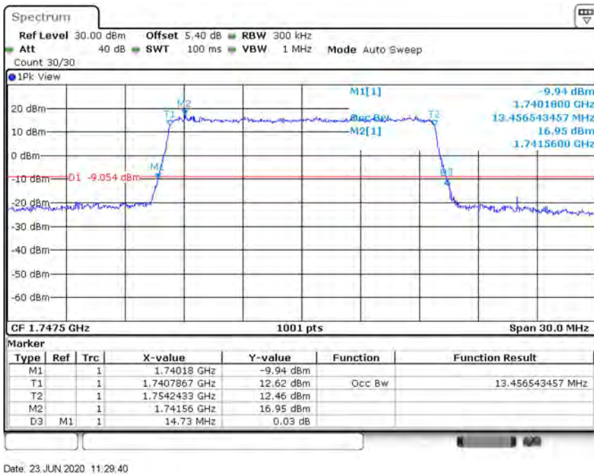
Band4-15MHz-64QAM-20025-75RB#0-13.457
