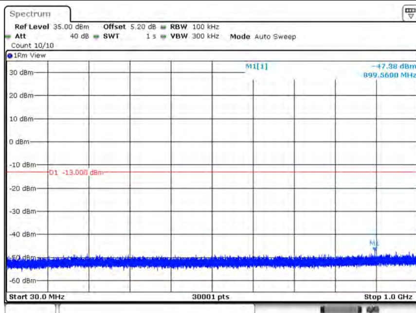
Band4-20MHz-16QAM-20175-1RB#0-Range1:30~1000MHz
