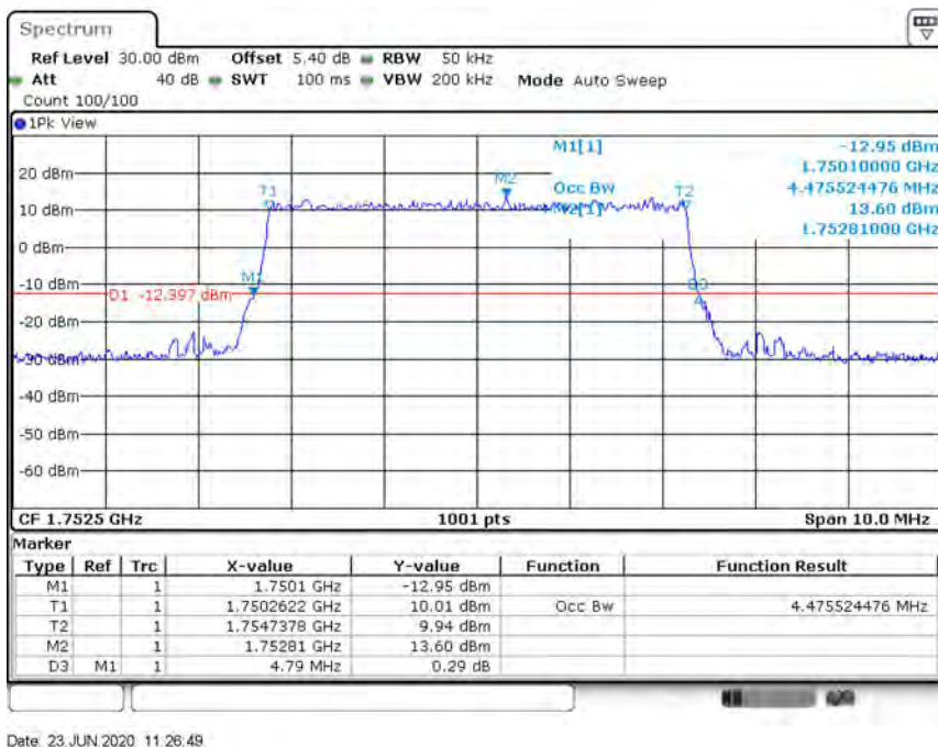
Band4-5MHz-64QAM-19975-25RB#0-4.466
