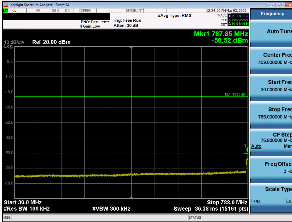
Plot 7-5. Conducted Spurious Plot (LTE Band 14 – 10 MHz QPSK - RB Size 1, RB Offset 0 - Mid Channel)
