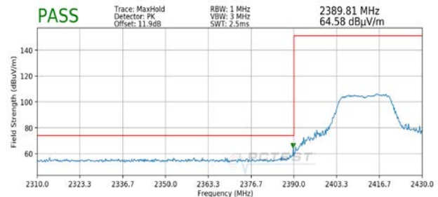
Plot 7-40. Radiated Restricted Lower Band Edge Measurement (Peak)
