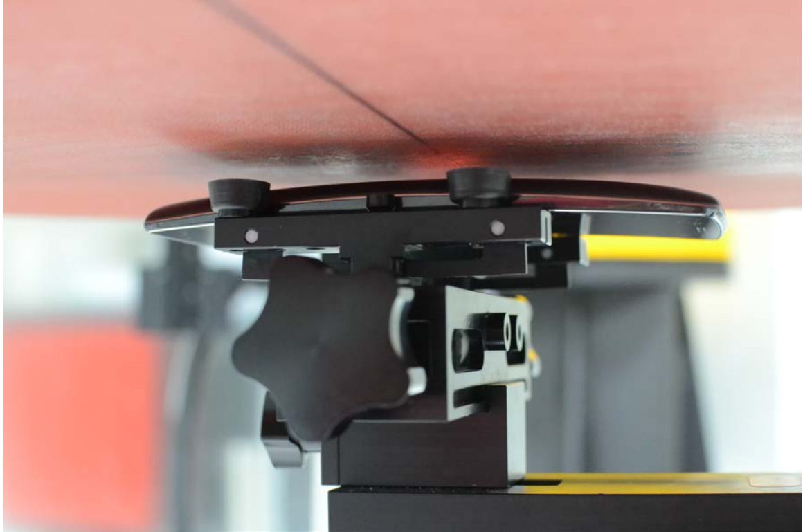
SAR Test Setup Photo 5: Back at 0.8 cm
