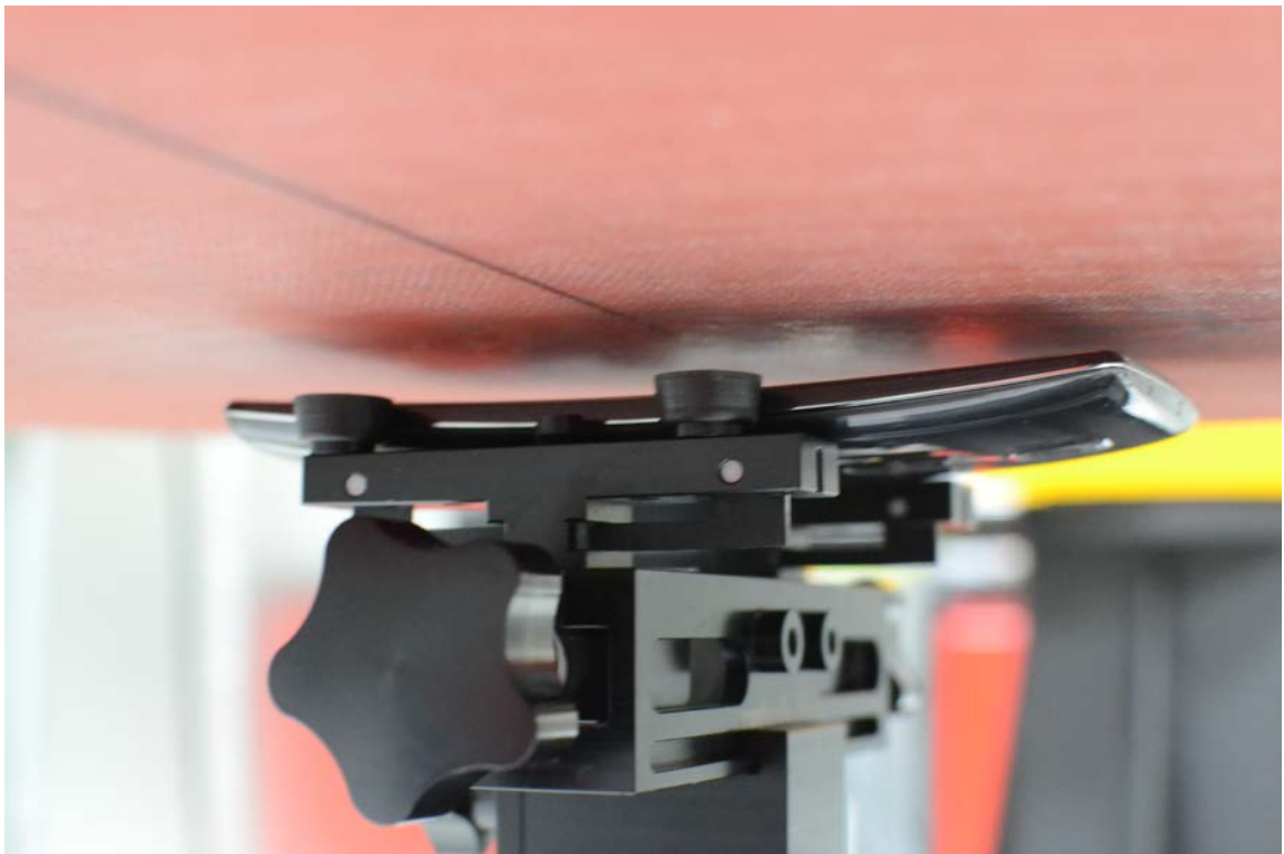
SAR Test Setup Photo 6: Front at 0.8 cm
