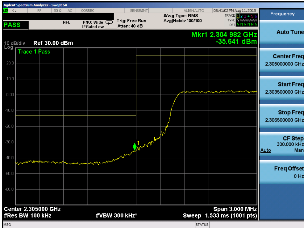
Plot 6-161. Lower Band Edge Plot (Band 30 – 10.0MHz QPSK – RB Size 50)
