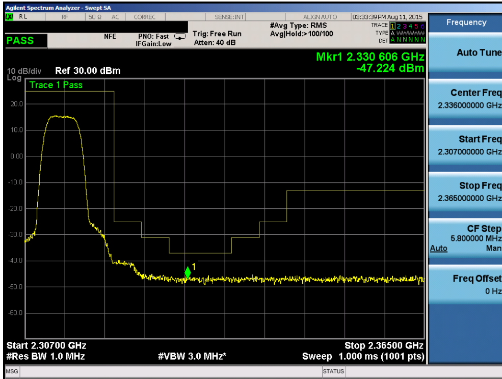
Plot 6-160. Upper Extended Band Edge Plot (Band 30 – 5.0MHz QPSK – RB Size 25)
