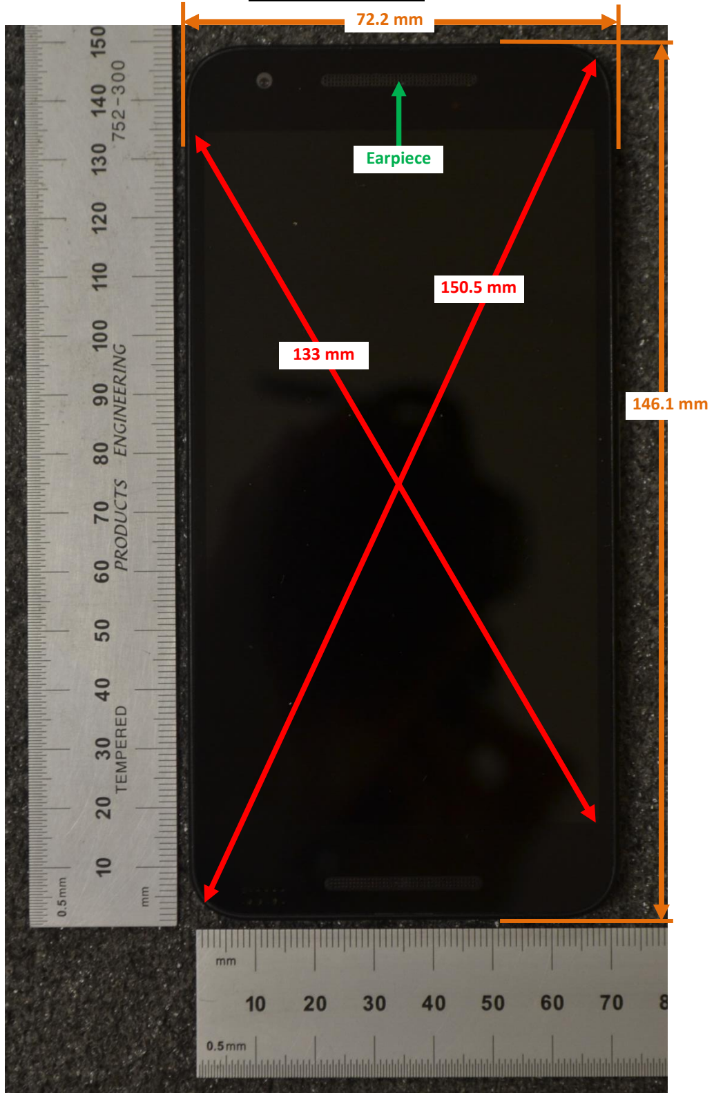
Overall Dimensions
