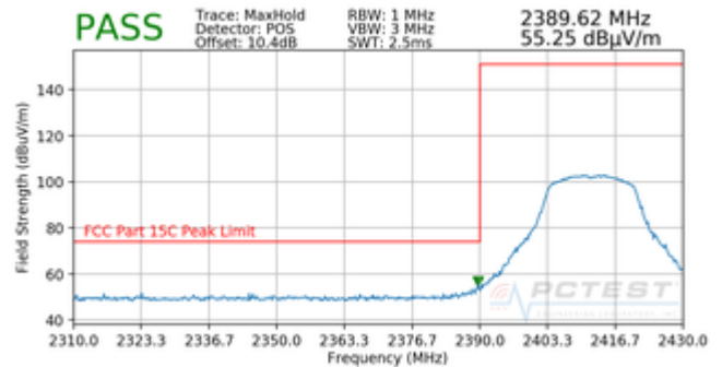
Plot 7-16. Radiated Restricted Lower Band Edge Measurement SISO ANT2 (Peak)
