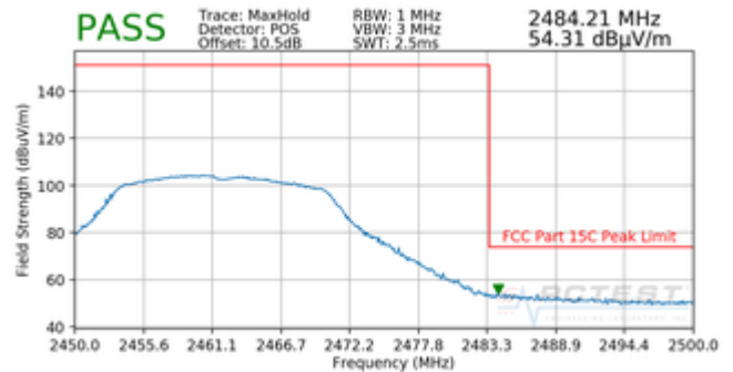
Plot 7-18. Radiated Restricted Upper Band Edge Measurement SISO ANT2 (Peak)
