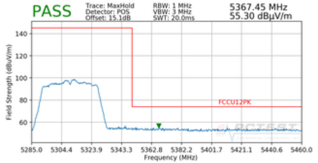
Plot 7-60. Radiated Band Edge Plot (Peak – WCP)
