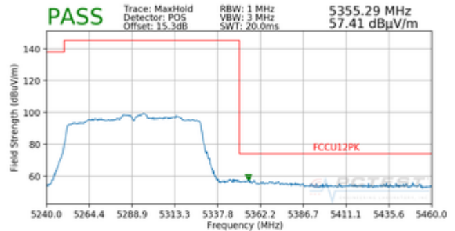
Plot 7-64. Radiated Upper Band Edge Plot (Peak – UNII Band 2A)
