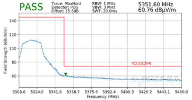
Plot 7-87. Radiated Band Edge Plot (Peak – WCP)
