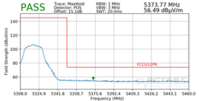
Plot 7-19. Radiated Upper Band Edge Plot (Peak – UNII Band 2A)
