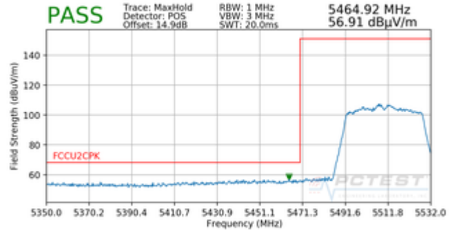
Plot 7-93. Radiated Lower Band Edge Plot (Peak – UNII Band 2C)
