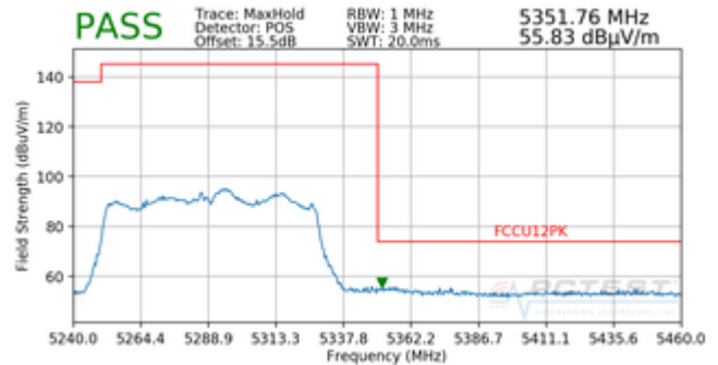
Plot 7-37. Radiated Upper Band Edge Plot (Peak – UNII Band 2A)
