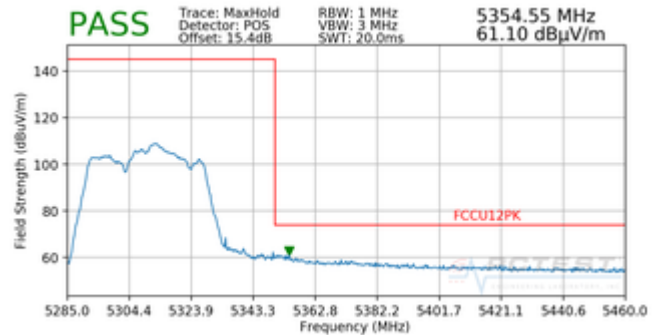
Plot 7-91. Radiated Upper Band Edge Plot (Peak – UNII Band 2A)
