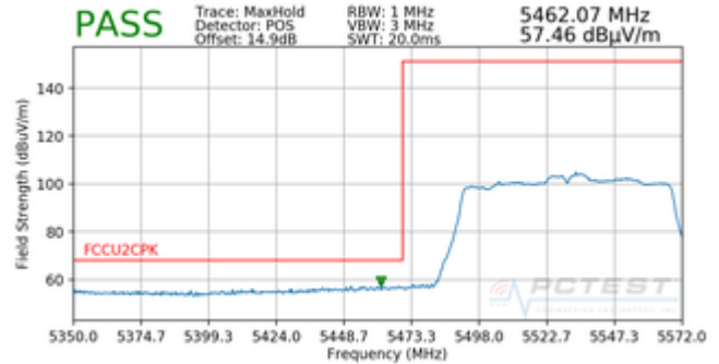
Plot 7-66. Radiated Lower Band Edge Plot (Peak – UNII Band 2C)
