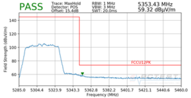
Plot 7-96. Radiated Band Edge Plot (Peak – WCP)
