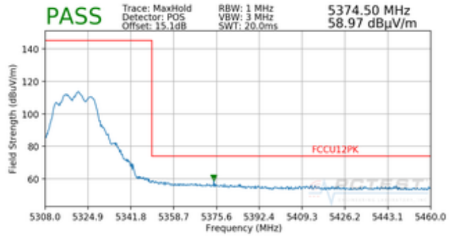
Plot 7-78. Radiated Band Edge Plot (Peak – WCP)
