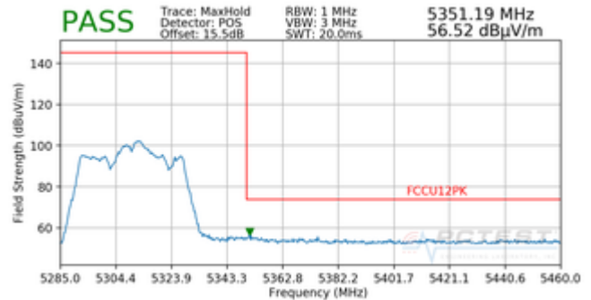
Plot 7-28. Radiated Upper Band Edge Plot (Peak – UNII Band 2A)
