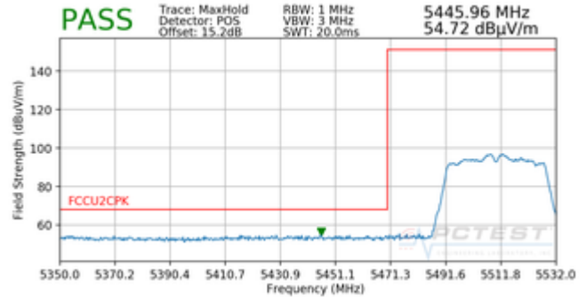
Plot 7-30. Radiated Lower Band Edge Plot (Peak – UNII Band 2C)
