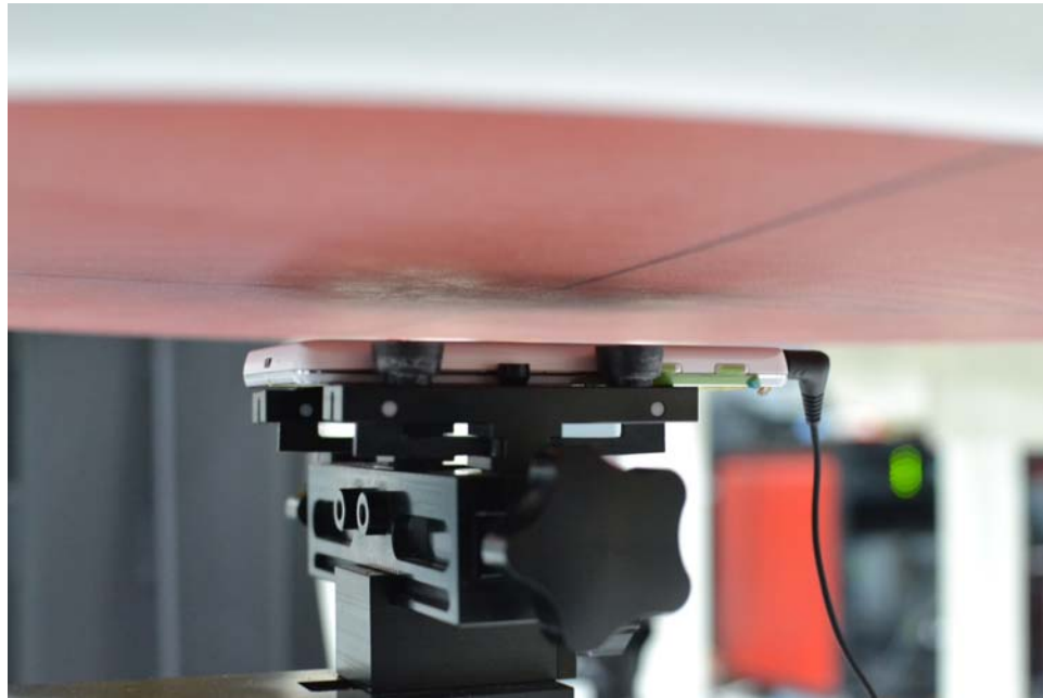
SAR Test Setup Photo 11 - Body Worn with Headphones at 1.0 cm
