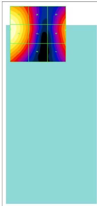
Figure 11-1 Sample E-field Scan Overlay (T-Coil Centered Scan pictured. See Test Setup Photographs Acoustic Scan Overlay and actual WD overlay)
