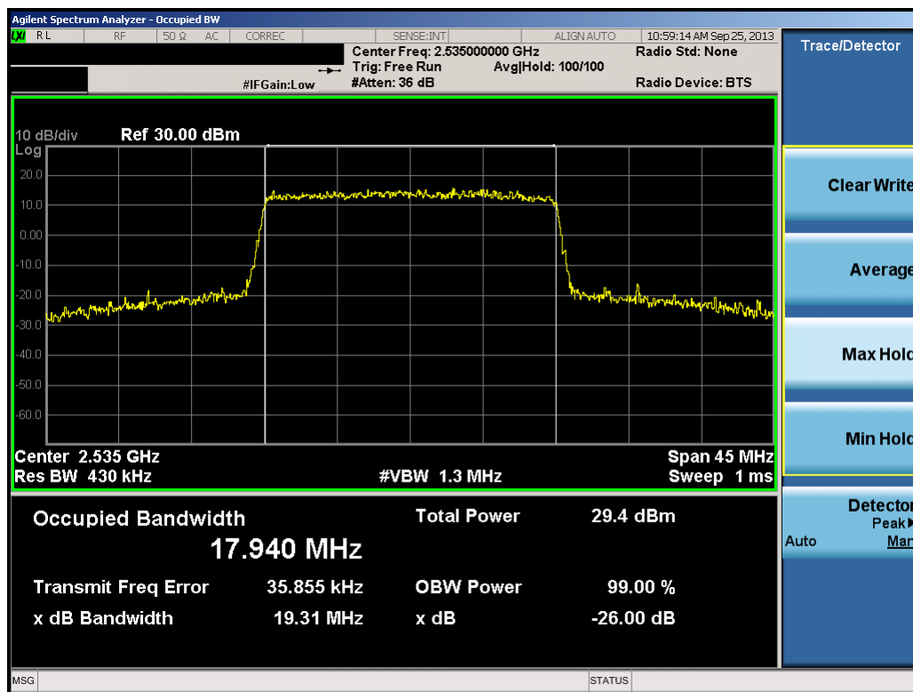
Plot 11-43. Occupied Bandwidth Plot (20.0MHz 16-QAM – RB Size 100)
