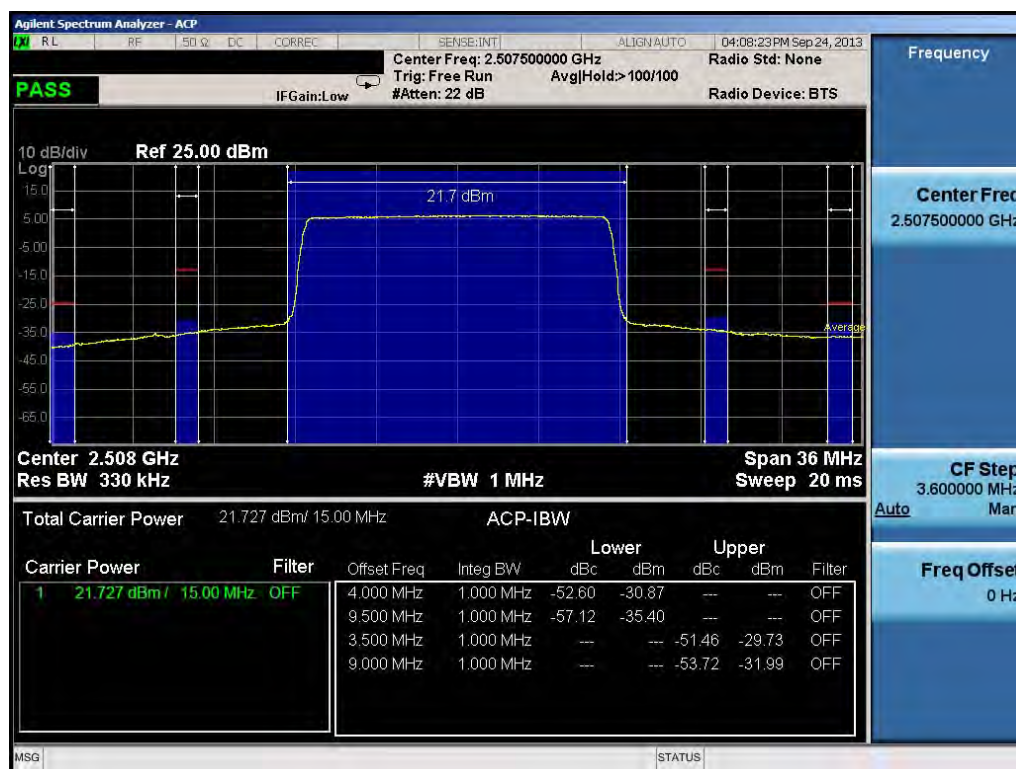
Plot 11-37. ACP Plot (15.0MHz QPSK – RB Size 75) – Low Channel
