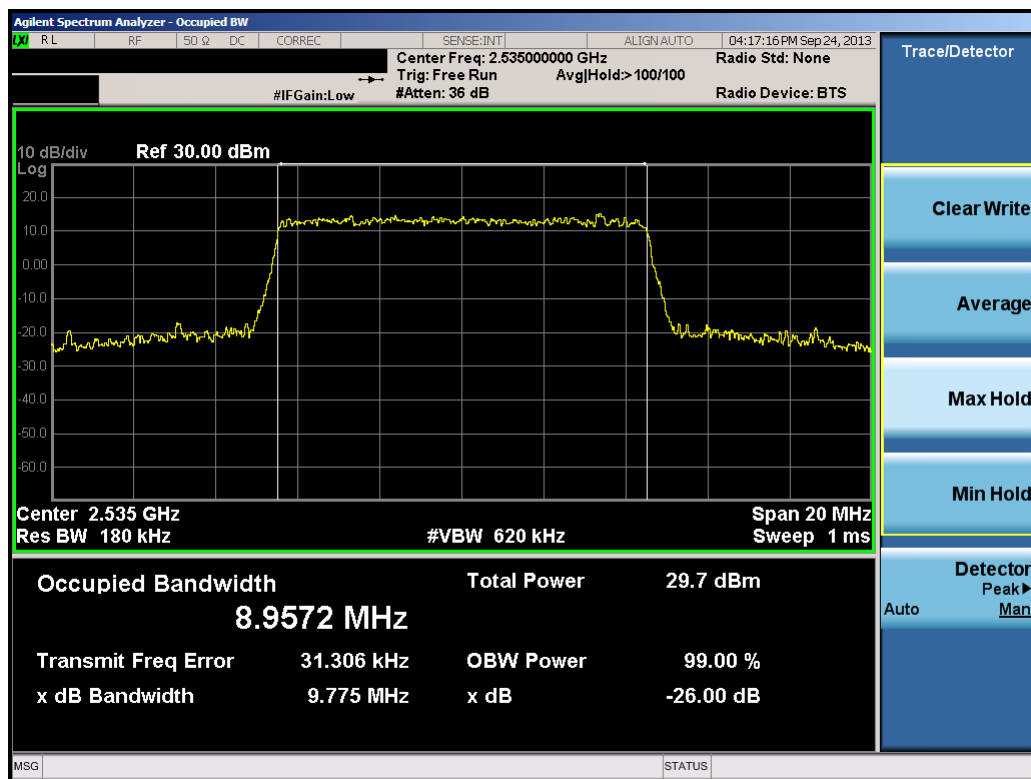
Plot 11-21. Occupied Bandwidth Plot (10.0MHz 16-QAM – RB Size 50)
