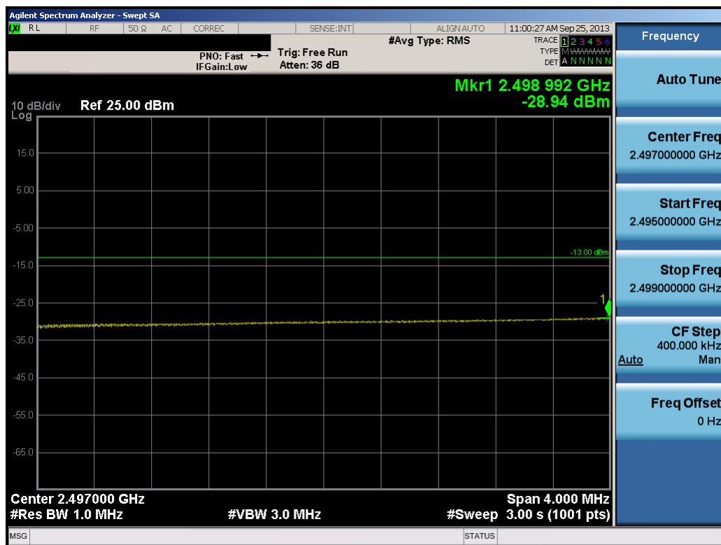
Plot 11-41. Lower Extended Band Edge Plot (20.0MHz QPSK – RB Size 100)
