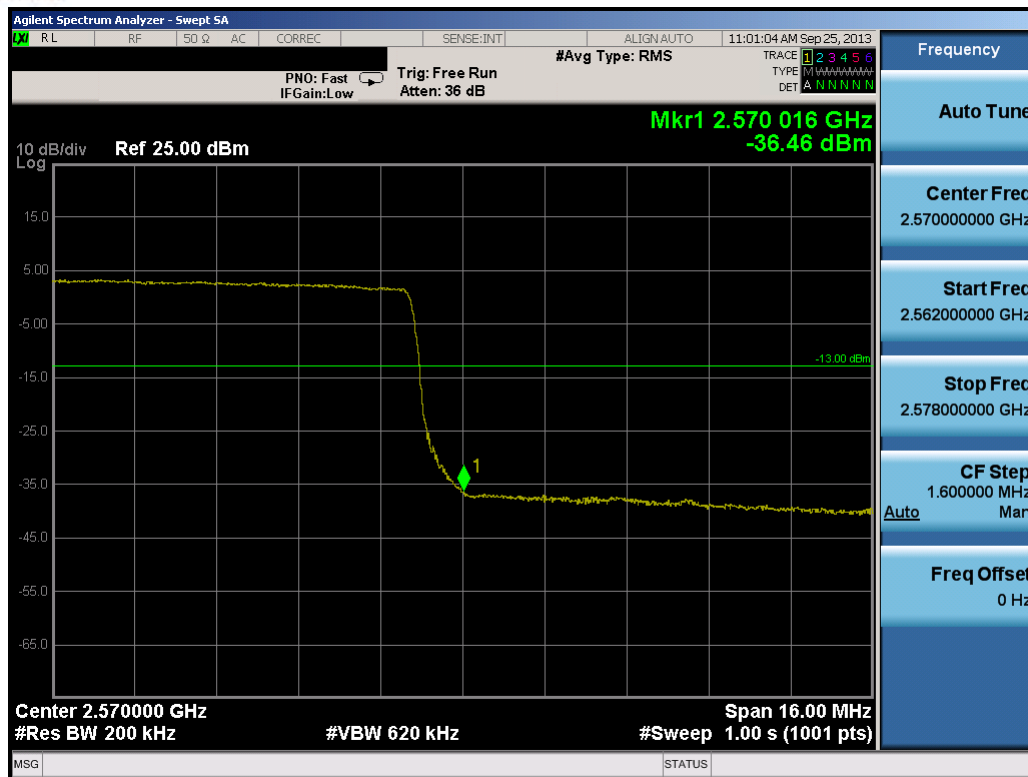
Plot 11-44. Upper Band Edge Plot (20.0MHz QPSK – RB Size 100)
