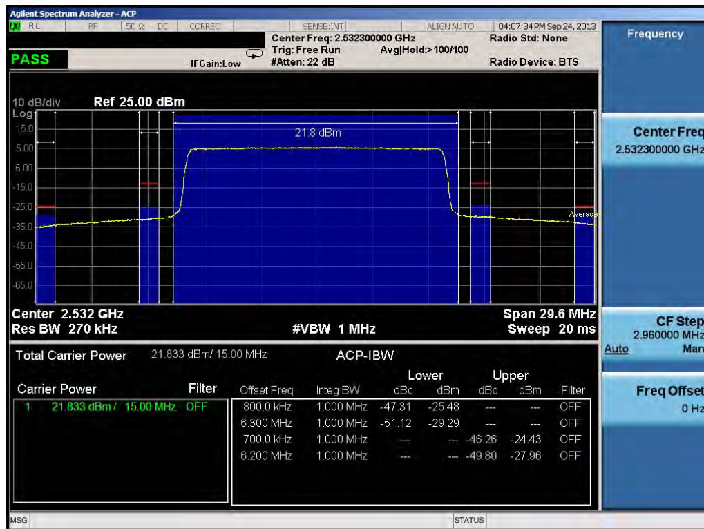
Plot 11-38. ACP Plot (15.0MHz QPSK – RB Size 75) – Mid Channel
