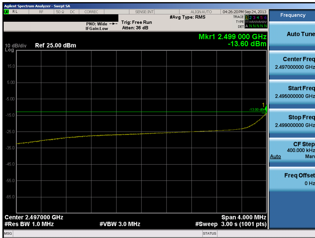
Plot 11-2. Lower Extended Band Edge Plot (5.0MHz QPSK – RB Size 25)
