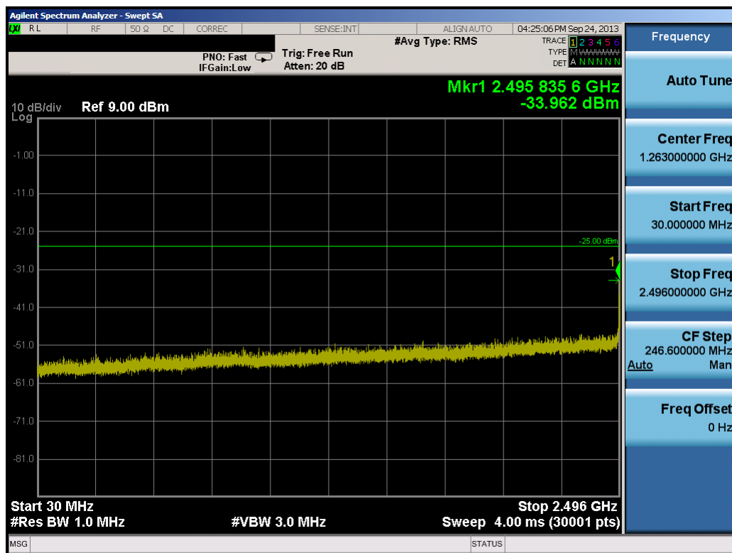
Plot 11-5. Conducted Spurious Plot (5.0MHz QPSK – RB Size 1, RB Offset 0 – Low Channel)
