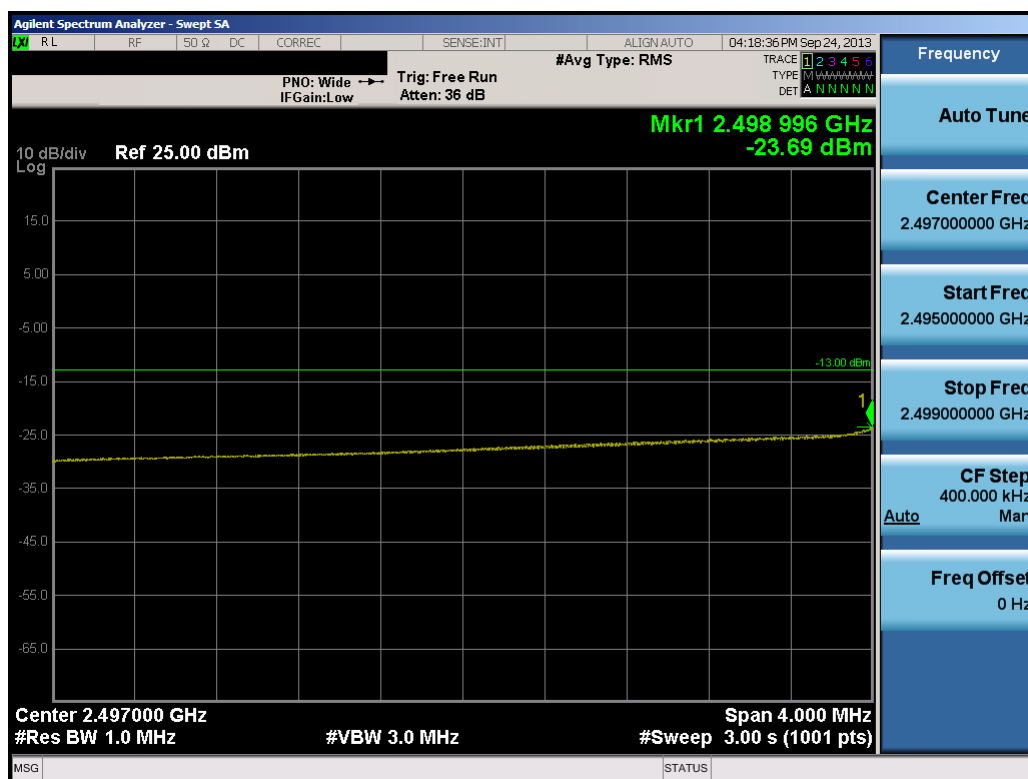
Plot 11-19. Lower Extended Band Edge Plot (10.0MHz QPSK – RB Size 50)
