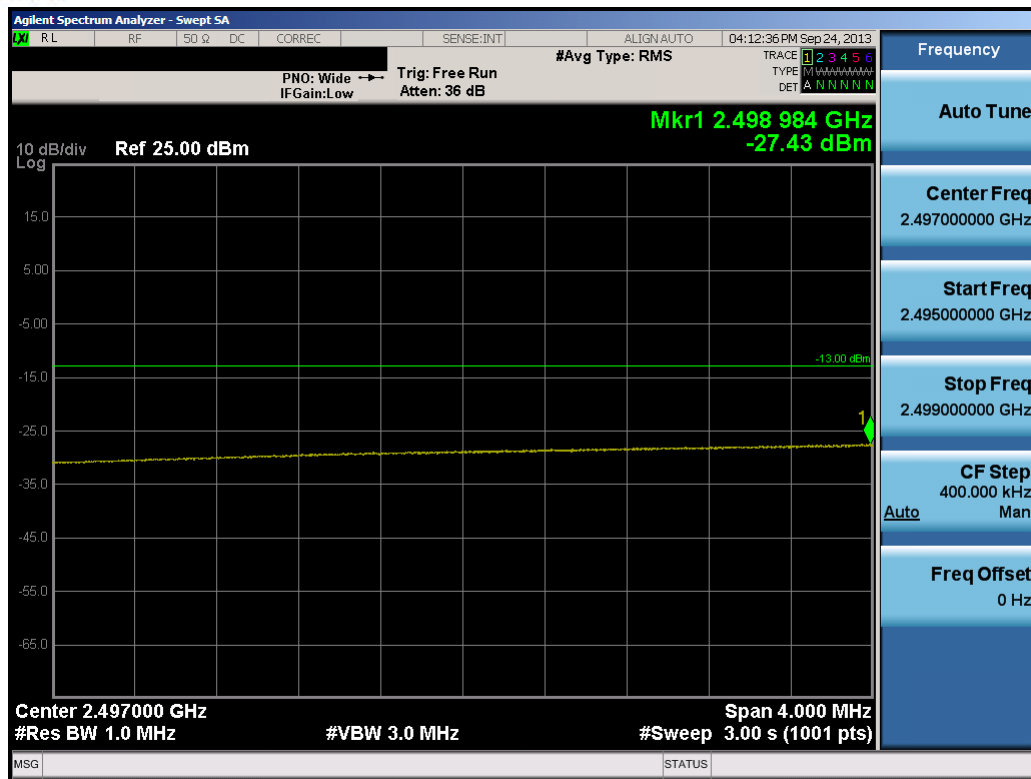
Plot 11-30. Lower Extended Band Edge Plot (15.0MHz QPSK – RB Size 75)
