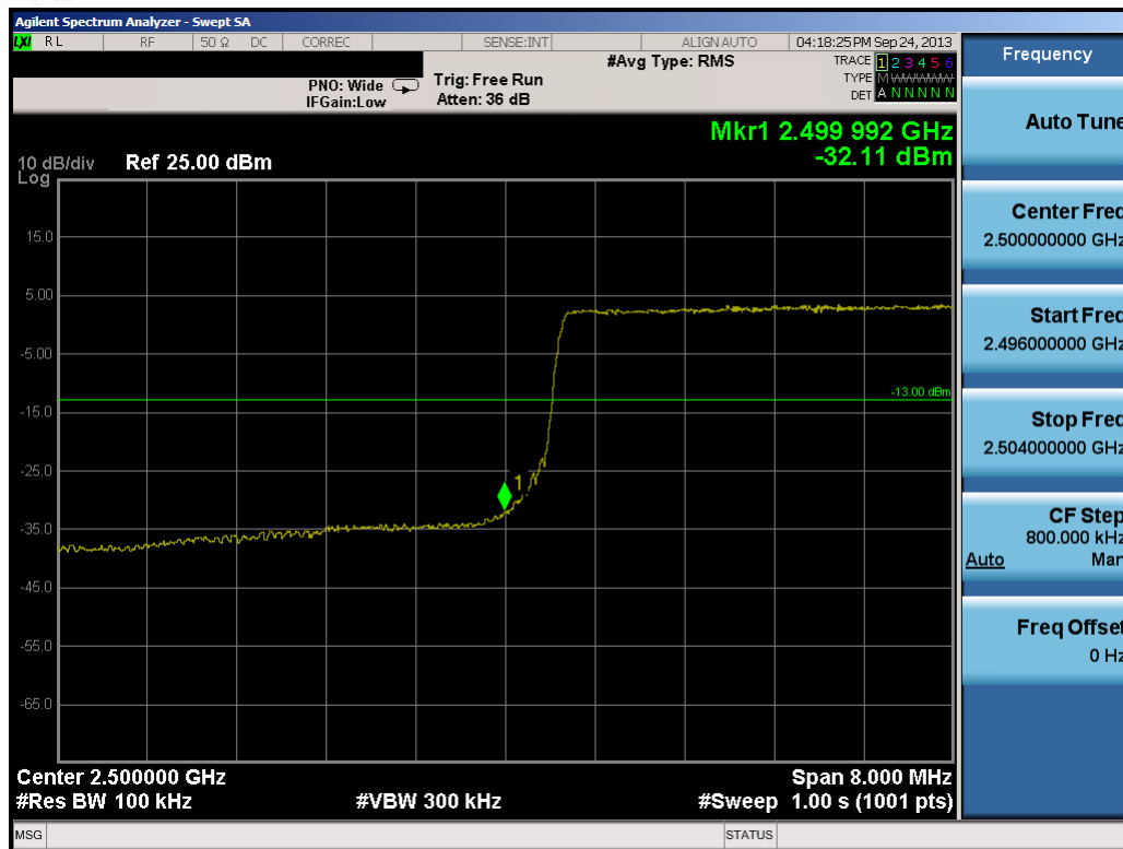
Plot 11-18. Lower Band Edge Plot (10.0MHz QPSK – RB Size 50)
