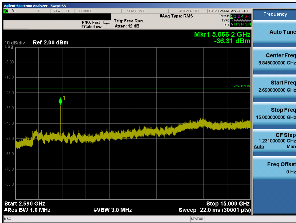
Plot 11-8. Conducted Spurious Plot (5.0MHz QPSK – RB Size 1, RB Offset 0 – Mid Channel)
