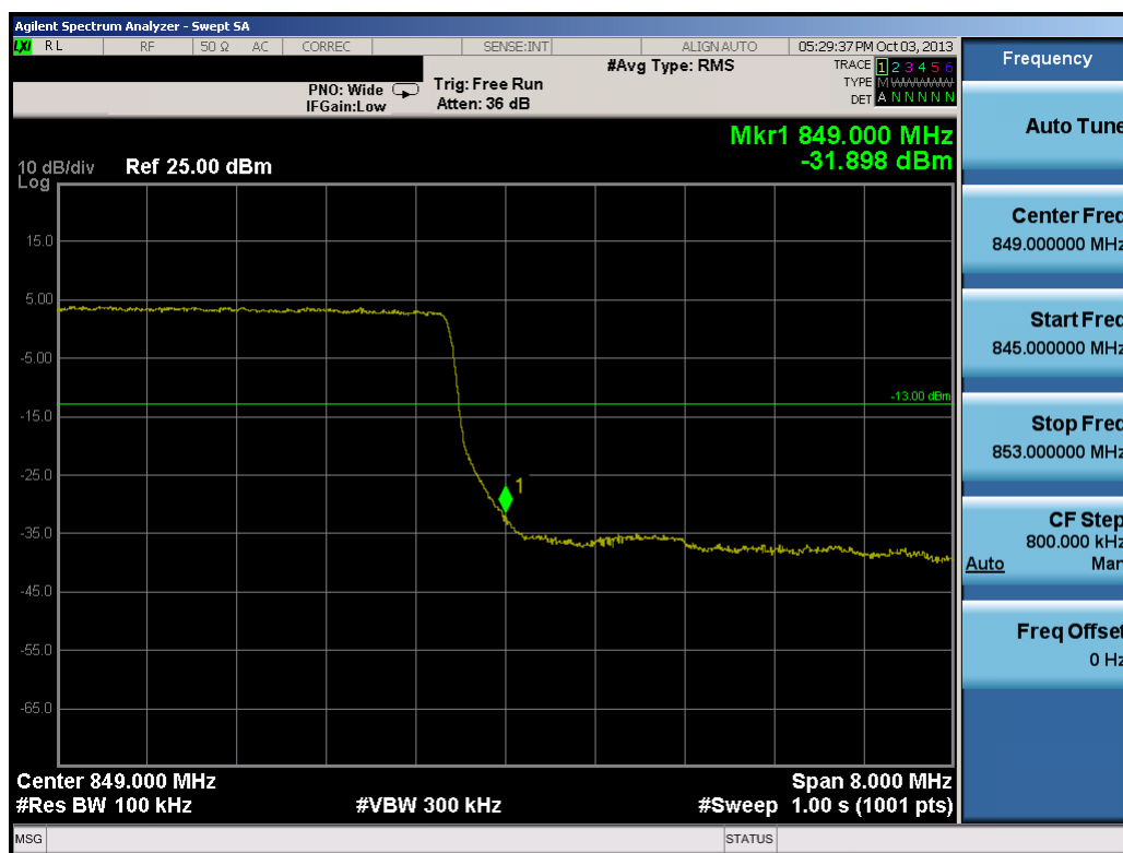
Plot 8-17. Upper Band Edge Plot (10.0MHz QPSK – RB Size 50)
