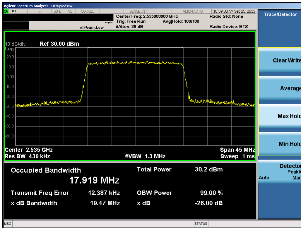
Plot 11-42. Occupied Bandwidth Plot (20.0MHz QPSK – RB Size 100)
