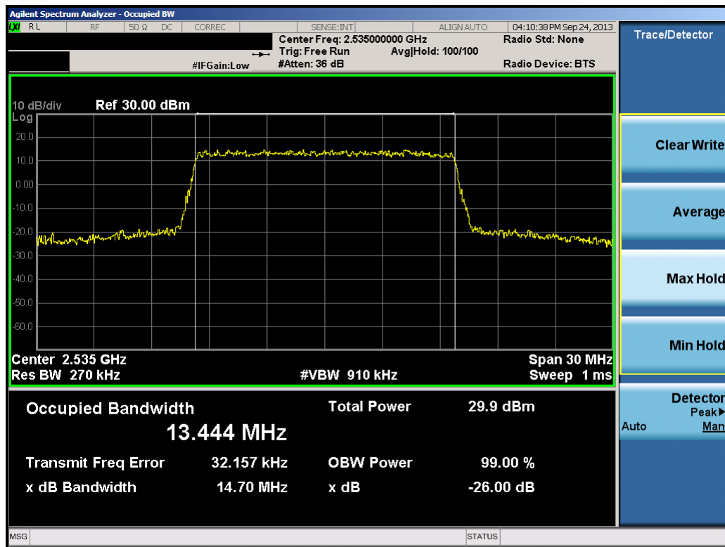
Plot 11-32. Occupied Bandwidth Plot (15.0MHz 16-QAM – RB Size 75)
