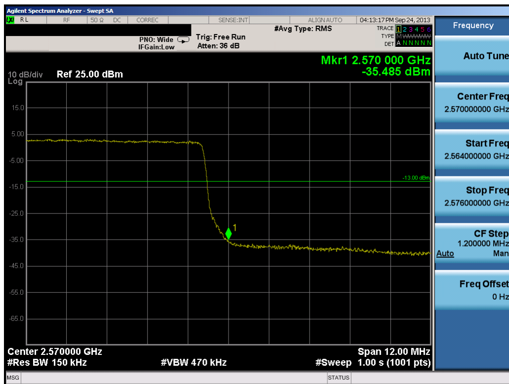
Plot 11-33. Upper Band Edge Plot (15.0MHz QPSK – RB Size 75)
