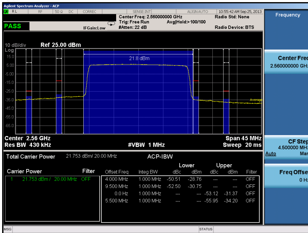
Plot 11-50. ACP Plot (20.0MHz QPSK – RB Size 100) – High Channel
