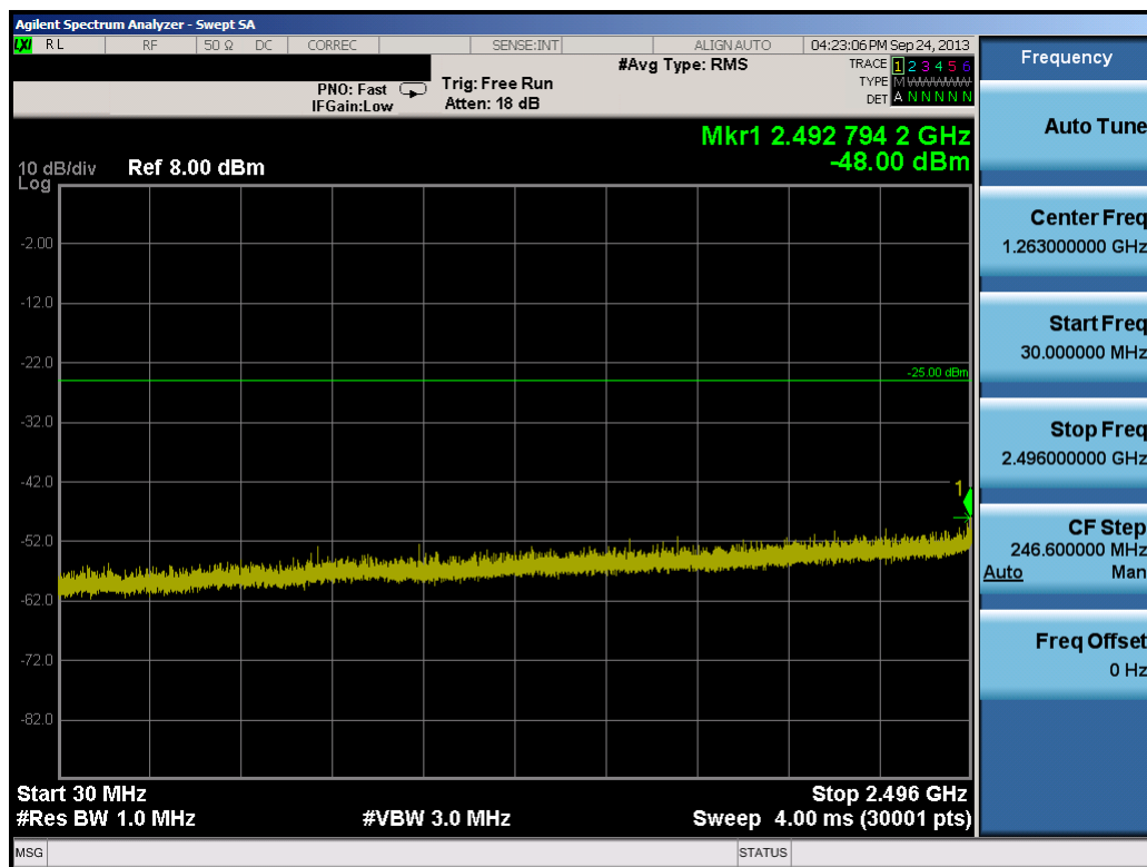
Plot 11-7. Conducted Spurious Plot (5.0MHz QPSK – RB Size 1, RB Offset 0 – Mid Channel)
