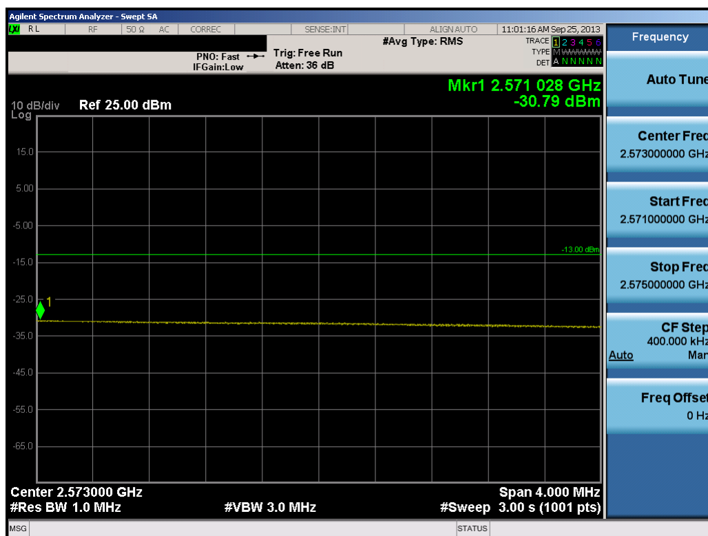
Plot 11-45. Upper Extended Band Edge Plot (20.0MHz QPSK – RB Size 100)
