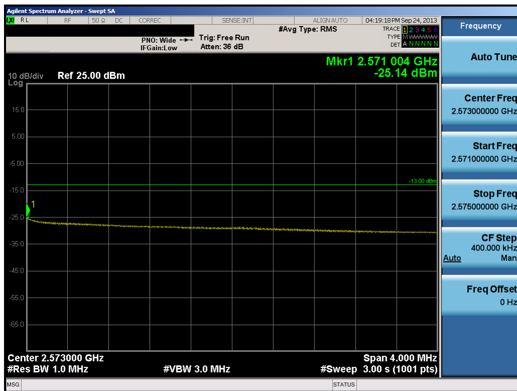
Plot 11-23. Upper Extended Band Edge Plot (10.0MHz QPSK – RB Size 50)
