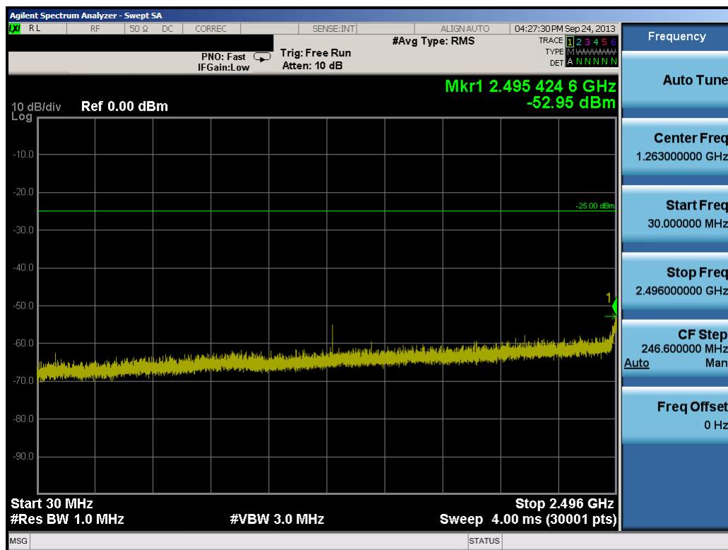
Plot 11-9. Conducted Spurious Plot (5.0MHz QPSK – RB Size 1, RB Offset 0 – High Channel)
