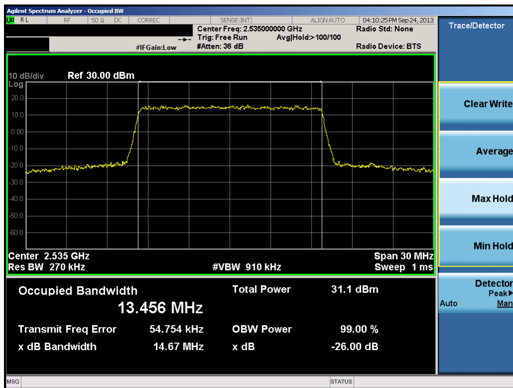
Plot 11-31. Occupied Bandwidth Plot (15.0MHz QPSK – RB Size 75)
