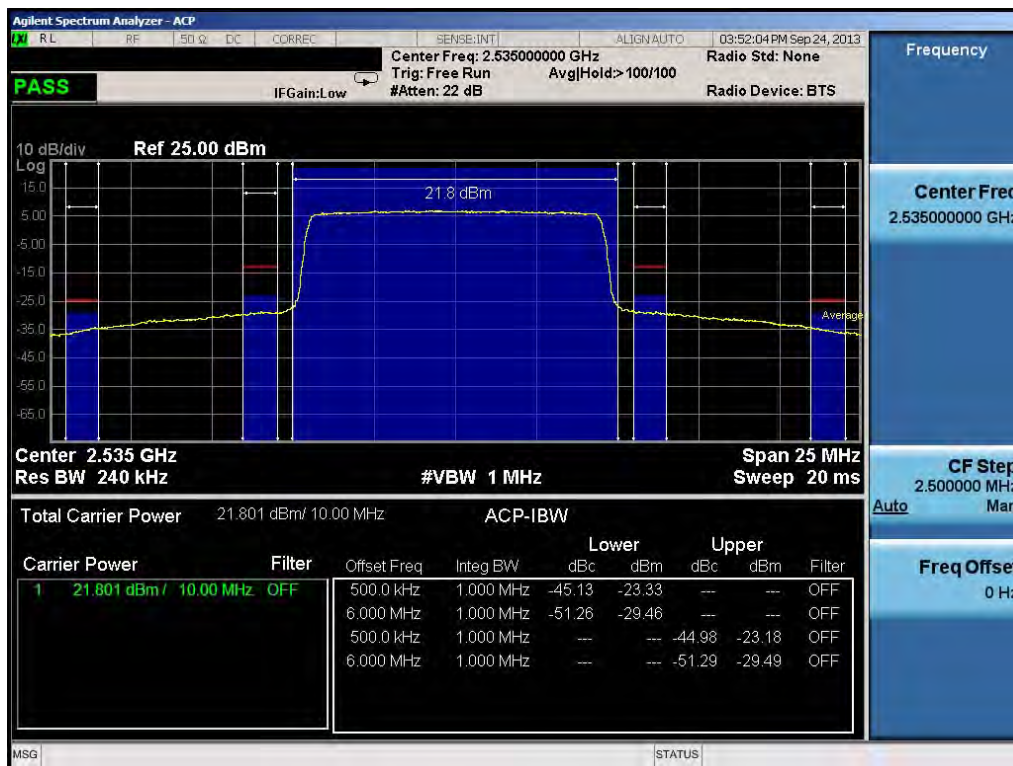
Plot 11-27. ACP Plot (10.0MHz QPSK – RB Size 50) – Mid Channel
