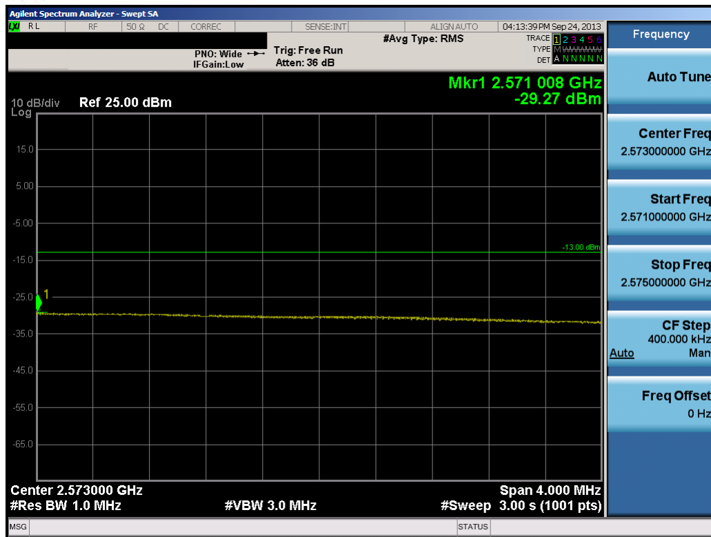
Plot 11-34. Upper Extended Band Edge Plot (15.0MHz QPSK – RB Size 75)
