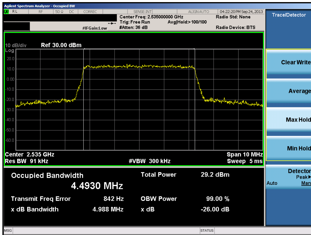
Plot 11-4. Occupied Bandwidth Plot (5.0MHz 16-QAM – RB Size 25)
