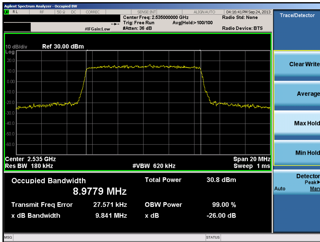
Plot 11-20. Occupied Bandwidth Plot (10.0MHz QPSK – RB Size 50)
