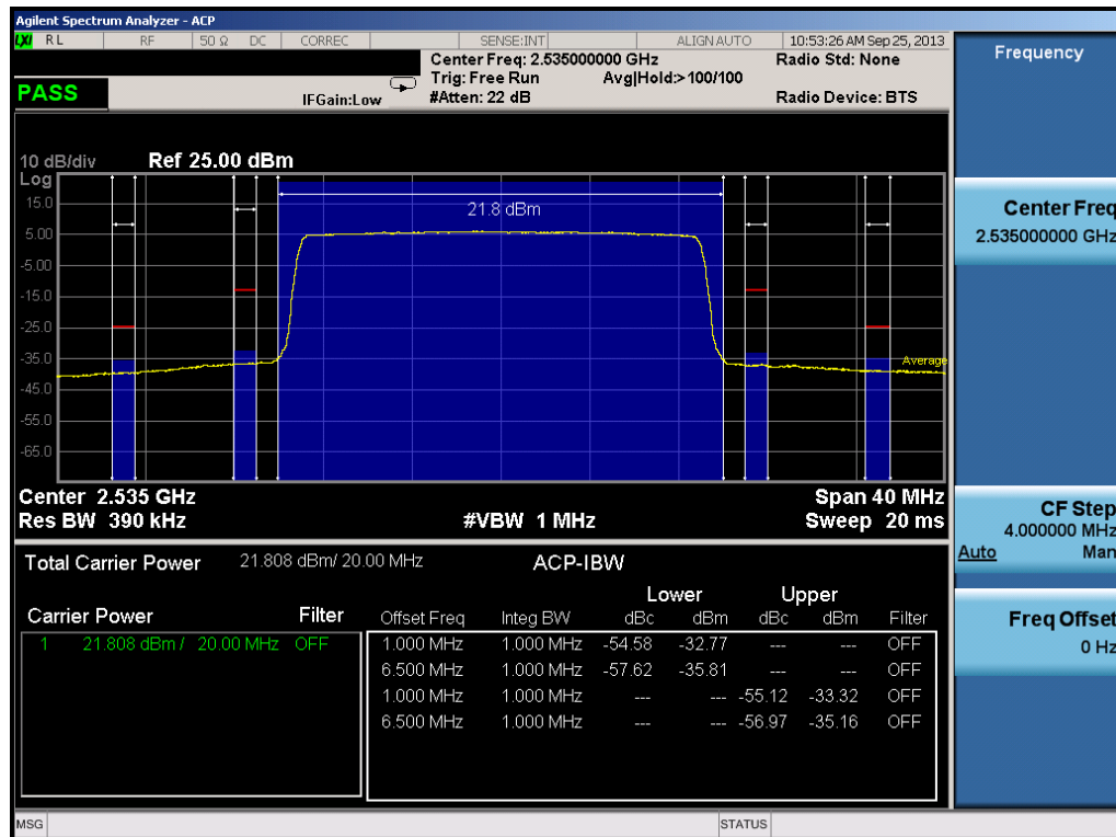
Plot 11-49. ACP Plot (20.0MHz QPSK – RB Size 100) – Mid Channel
