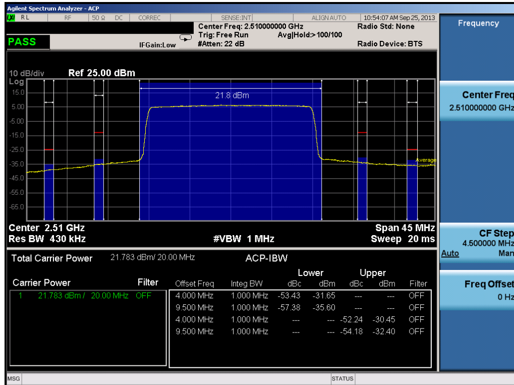
Plot 11-48. ACP Plot (20.0MHz QPSK – RB Size 100) – Low Channel
