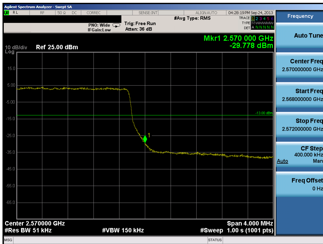
Plot 11-11. Upper Band Edge Plot (5.0MHz QPSK – RB Size 25)
