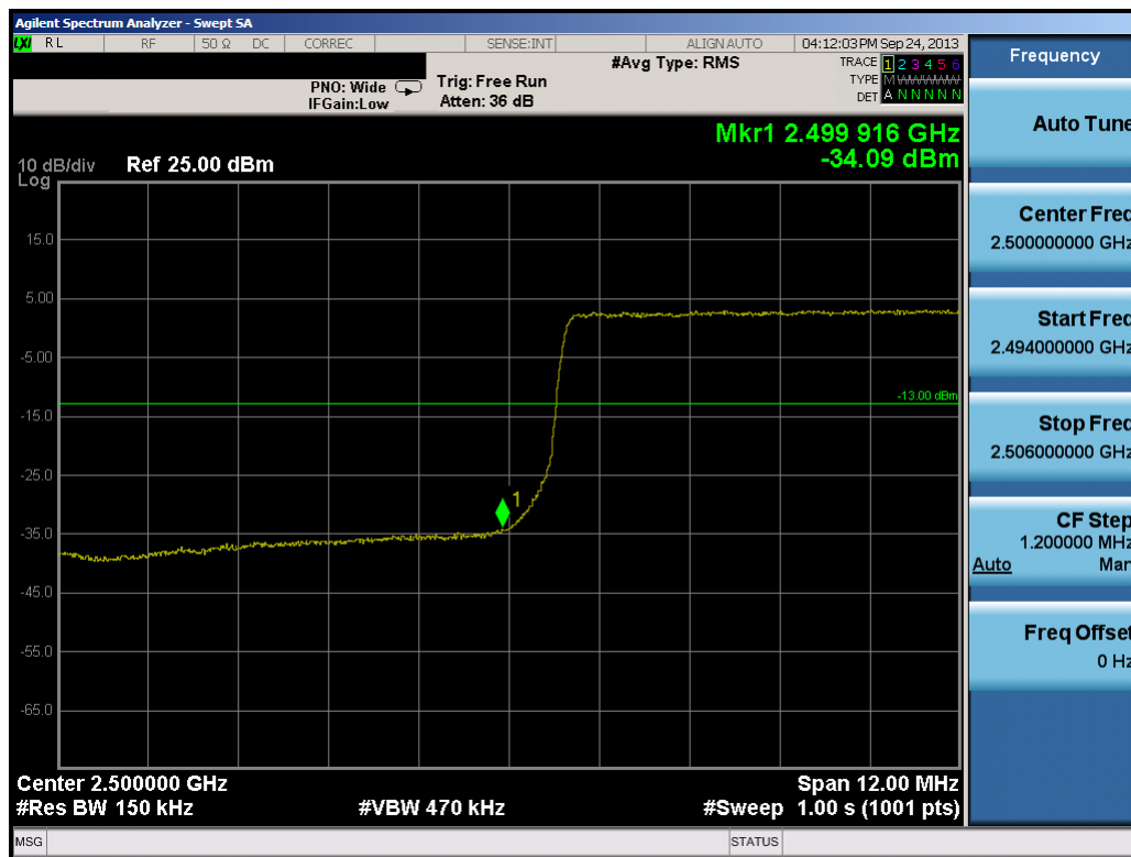
Plot 11-29. Lower Band Edge Plot (15.0MHz QPSK – RB Size 75)
