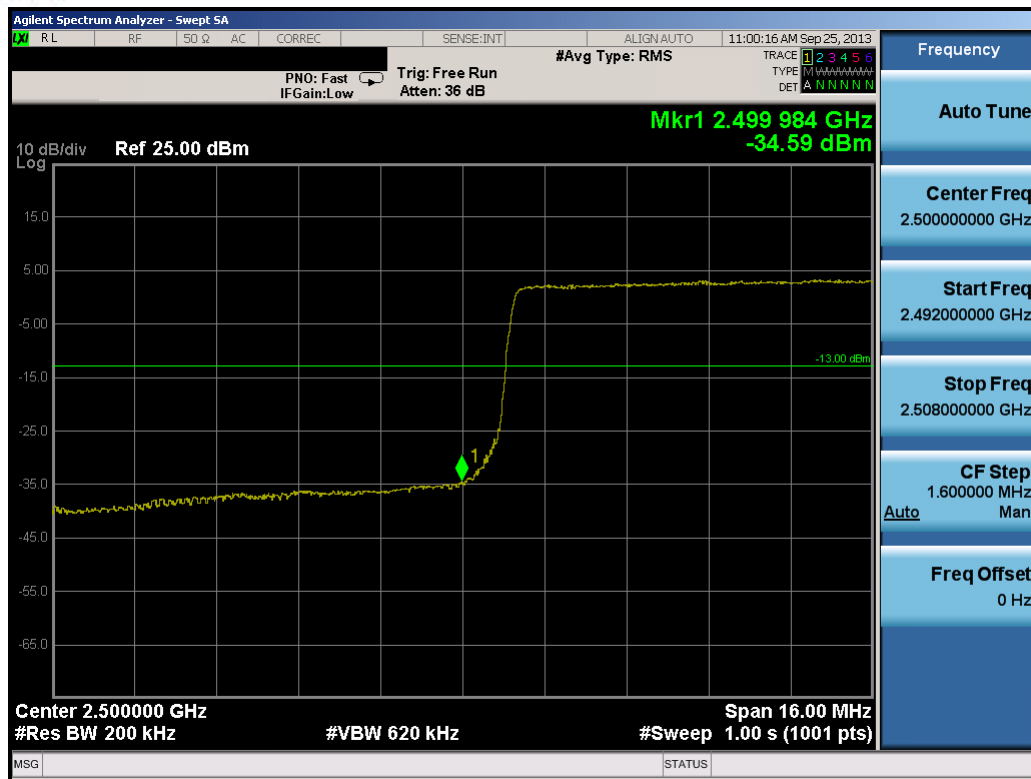
Plot 11-40. Lower Band Edge Plot (20.0MHz QPSK – RB Size 100)
