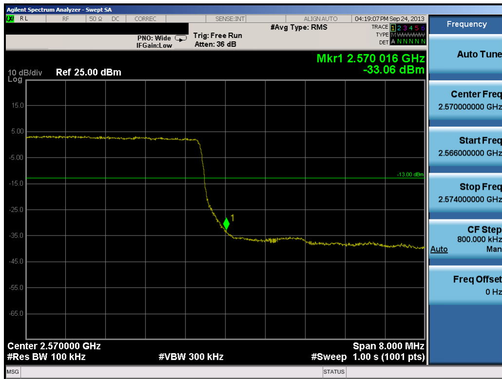
Plot 11-22. Upper Band Edge Plot (10.0MHz QPSK – RB Size 50)
