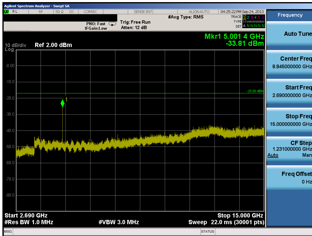
Plot 11-6. Conducted Spurious Plot (5.0MHz QPSK – RB Size 1, RB Offset 0 – Low Channel)
