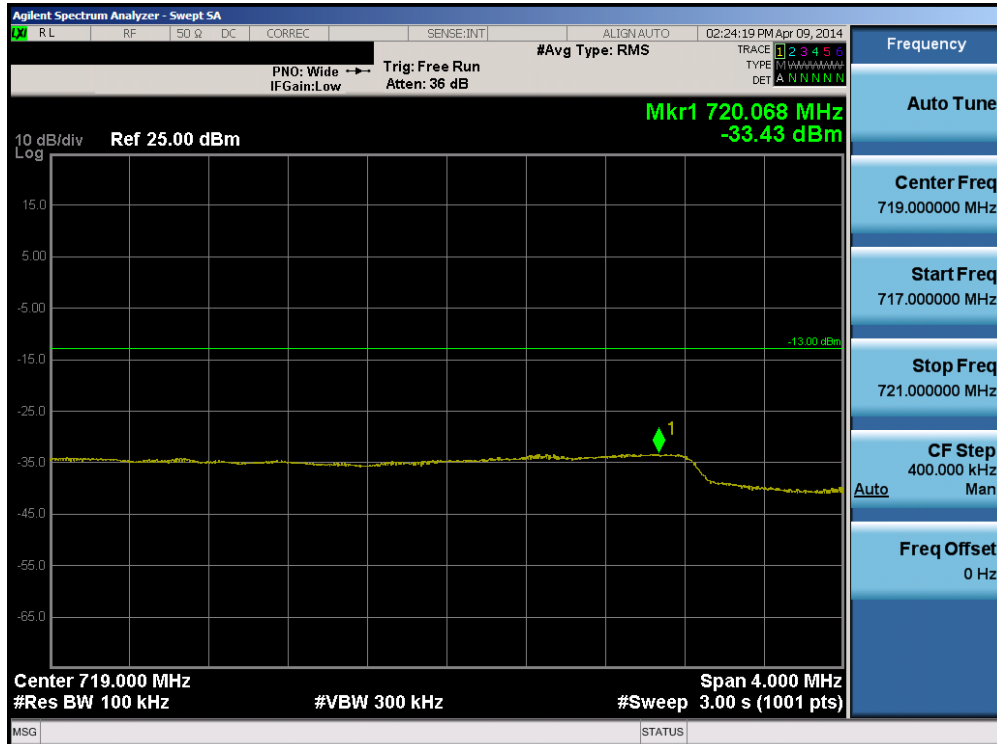
Plot 6-100. Upper Extended Band Edge Plot (Band 17 – 5.0MHz QPSK – RB Size 25)
