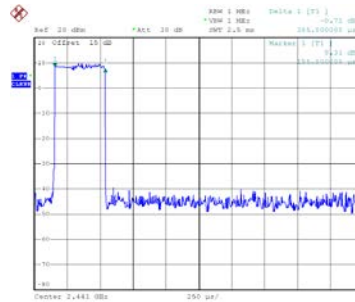
CH39-3DH1
