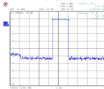
CH39-3DH3
