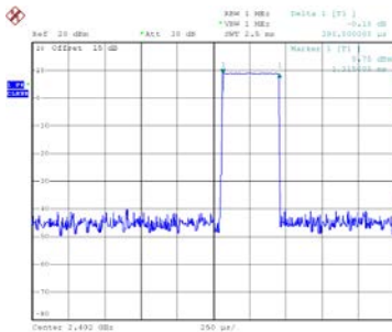
CH00-DH1
