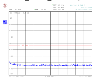
PCS1900_EDGE_CH661 Spectrum Plot
