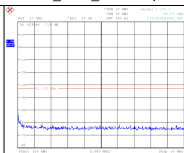
PCS1900_GSM_CH661 Spectrum Plot
