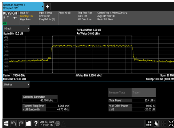
N66(45M)_CP-OFDM_256 QAM_Outer_Full_Mid_CH
