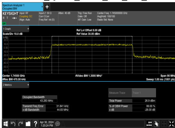
N66(45M)_CP- OFDM_QPSK_Outer_Full_Mid_CH
