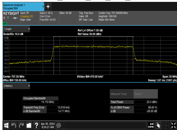
N12(15M)_CP-OFDM_256 QAM_Outer_Full_Mid_CH
