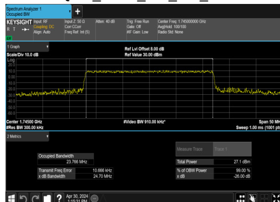
N66(25M)_CP-OFDM_16 QAM_Outer_Full_Mid_CH
