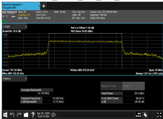
N12(15M)_CP-OFDM_64 QAM_Outer_Full_Mid_CH
