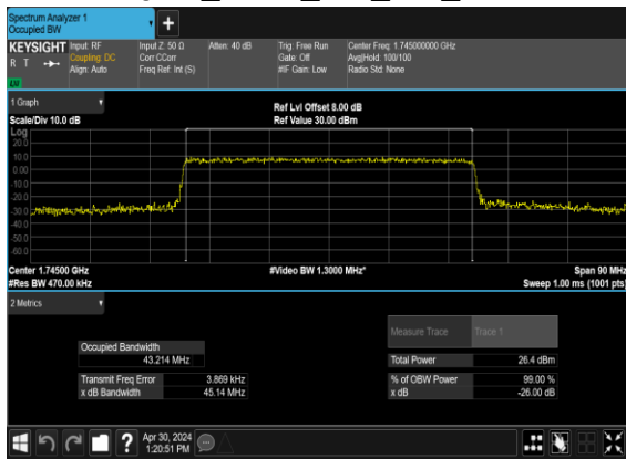
N66(45M)_CP-OFDM_64 QAM_Outer_Full_Mid_CH
