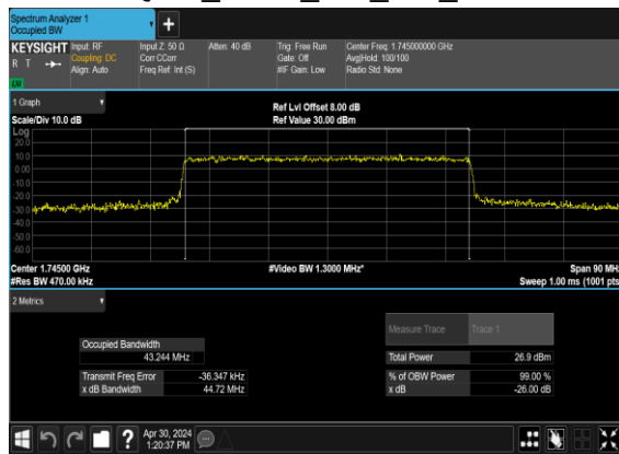
N66(45M)_CP-OFDM_16 QAM_Outer_Full_Mid_CH
