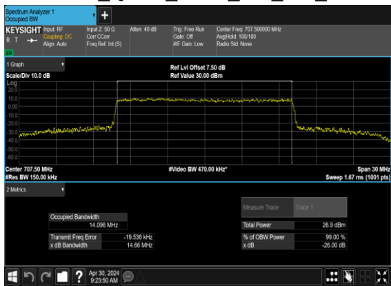
N12(15M)_CP- OFDM_QPSK_Outer_Full_Mid_CH
