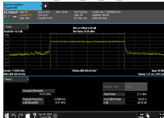
N66(20M)_CP-OFDM_16 QAM_Outer_Full_Mid_CH
