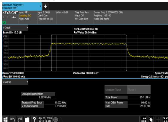
N7(10M)_CP-OFDM_64 QAM_Outer_Full_Mid_CH
