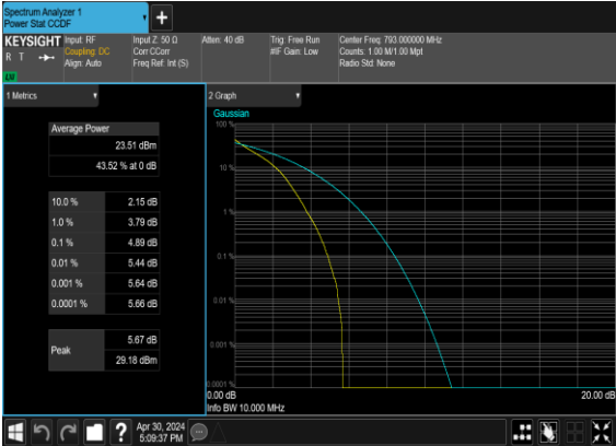
N14(10M)_DFT-s-OFDM_PI_2-BPSK_Outer_Full_Mid_CH
