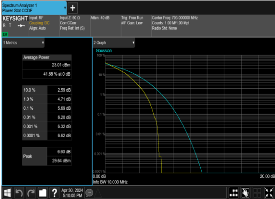
N14(10M)_DFT-s-OFDM_QPSK_Outer_Full_Mid_CH
