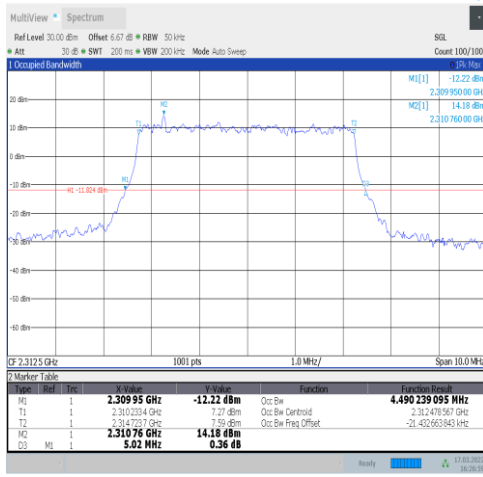
1-N30-15-5-H-1-DFT-QPSK-Outer_Full-25@0-Ant1-4.49-5.020-≤5-PASS
