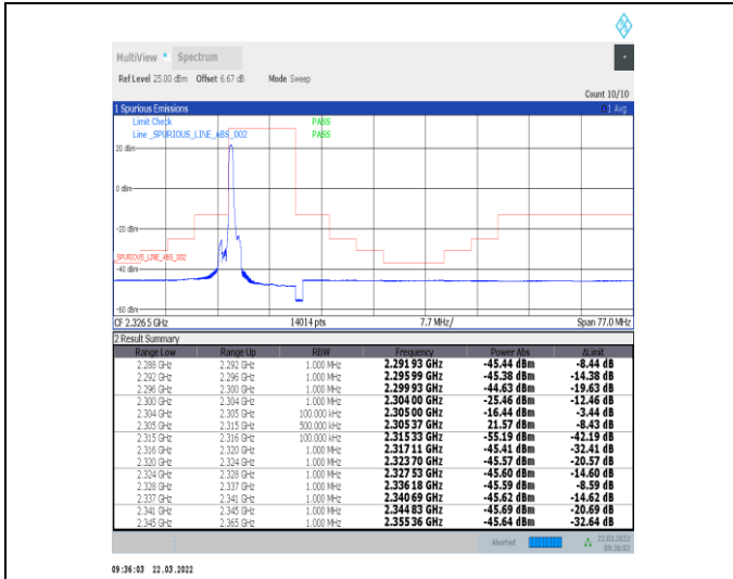
1-N30-15-10-M-1-DFT-PI2BPSK-Edge_1RB_Left-1@0-Ant1-PASS-see graph
