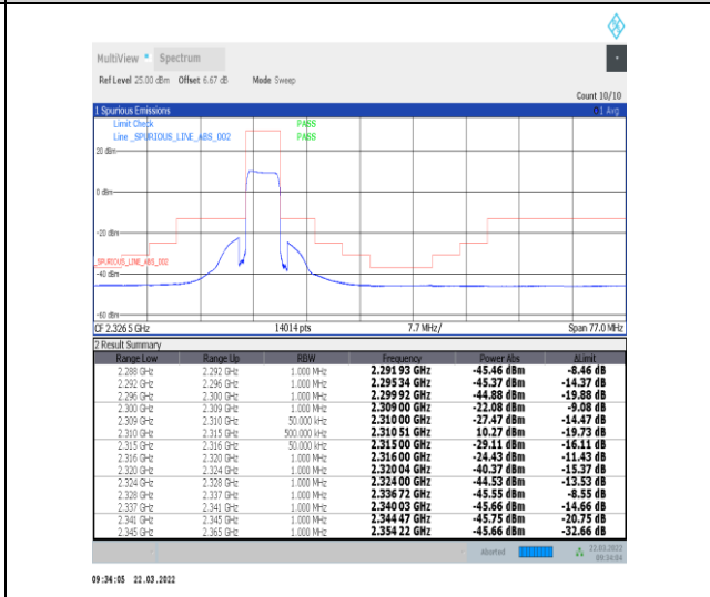
1-N30-15-5-H-6-CP-QPSK-Outer_Full-25@0-Ant1-PASS-see graph
