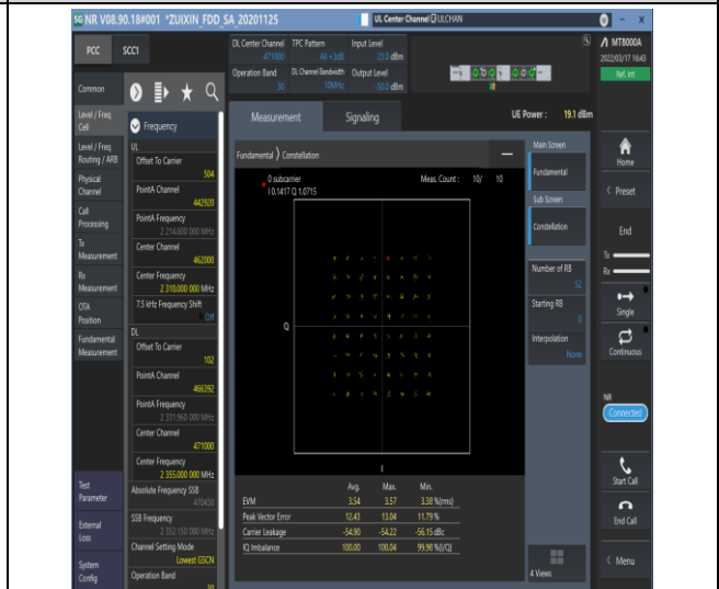
1-N30-15-10-M-8-CP-64QAM-Outer_Full-52@0-Ant1-see graph-PASS
