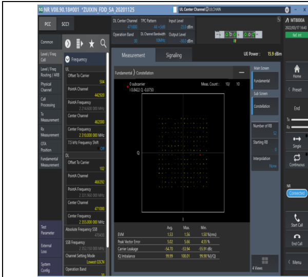
1-N30-15-10-M-9-CP-256QAM-Outer_Full-52@0-Ant 1-see graph-PASS
