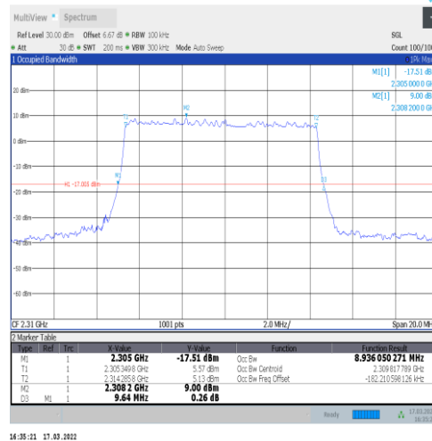
1-N30-15-10-M-5-DFT-256QAM-Outer_Full-50@0-A nt1-8.936-9.640-≤10-PASS
