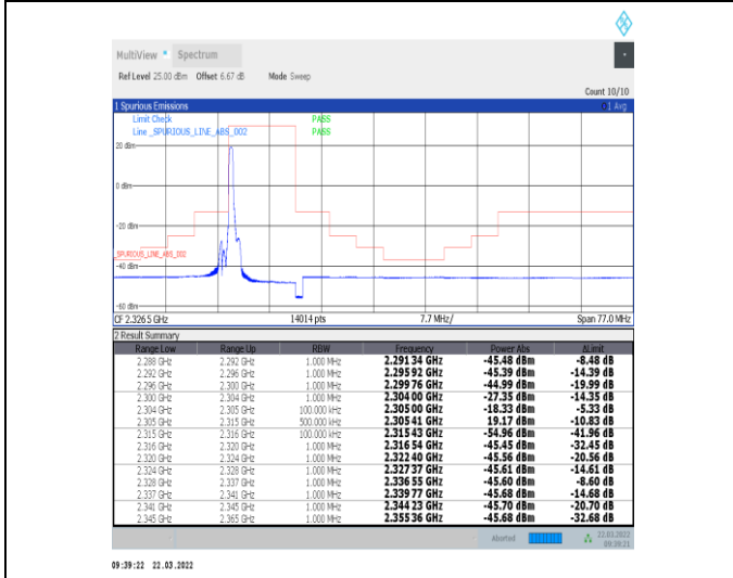
1-N30-15-10-M-4-CP-QPSK-Edge_1RB_Left-1@0-Ant1-PASS-see graph
