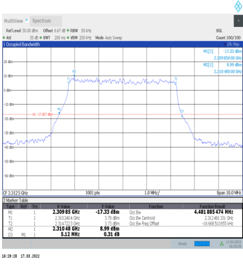
1-N30-15-5-H-5-DFT-256QAM-Outer_Full-25@0-Ant 1-4.482-5.120-≤5-PASS
