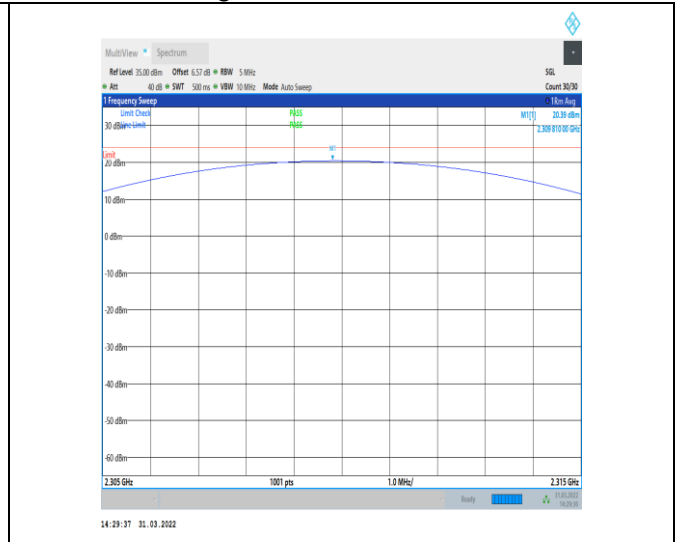
1-N30-PC3-15-5-M-3-DFT-PI2BPSK-Outer_Full-25@ 0-2305-2315-Ant1-20.39-23.98-PASS
