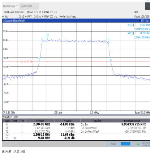
1-N30-15-10-M-4-DFT-64QAM-Outer_Full-50@0-Ant 1-8.935-9.680-≤10-PASS
