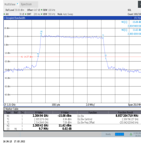
1-N30-15-10-M-3-DFT-16QAM-Outer_Full-50@0-Ant 1-8.937-9.700-≤10-PASS
