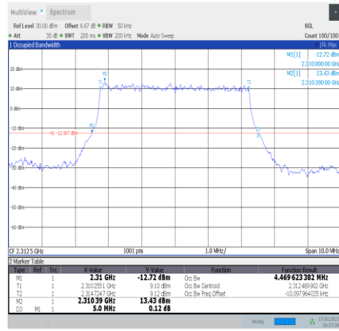
1-N30-15-5-H-2-DFT-PI2BPSK-Outer_Full-25@0-Ant1-4.47-5.000-≤5-PASS
