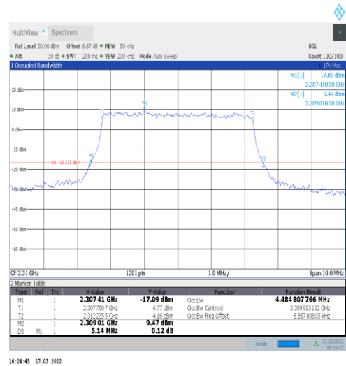
1-N30-15-5-M-7-CP-16QAM-Outer_Full-25@0-Ant1- 4.485-5.140-≤5-PASS
