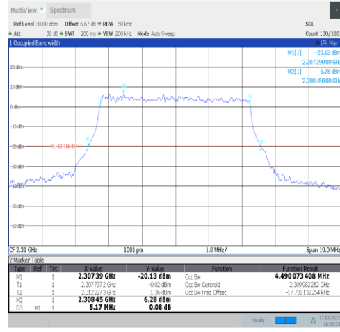
1-N30-15-5-M-9-CP-256QAM-Outer_Full-25@0-Ant1-4.49-5.170-≤5-PASS
