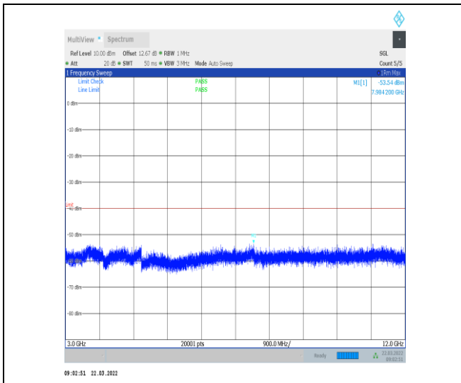
1-N30-15-10-M-1-DFT-PI2BPSK-Inner_1RB_Left-1 @ 1-3000-12000-Ant1--53.54--40-PASS
