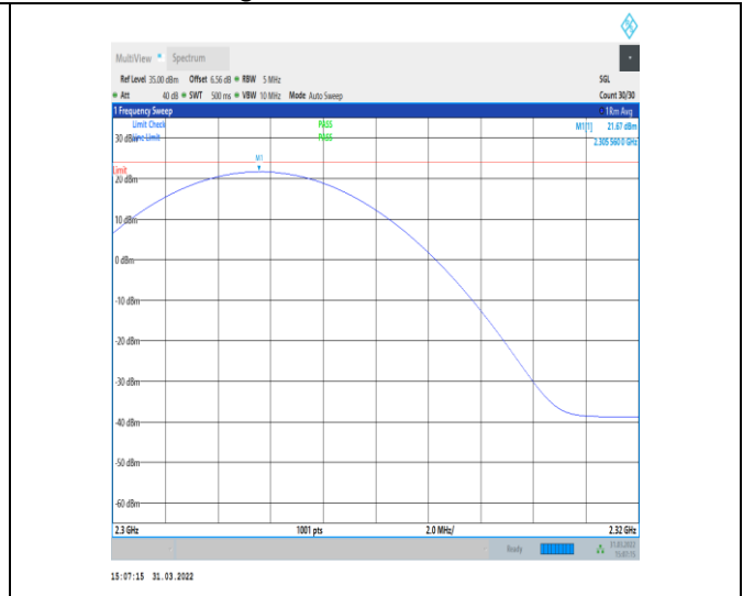
1-N30-PC3-15-10-M-1-DFT-PI2BPSK-Inner_1RB_Lef t-1 @1-2300-2320-Ant1-21.67-23.98-PASS
