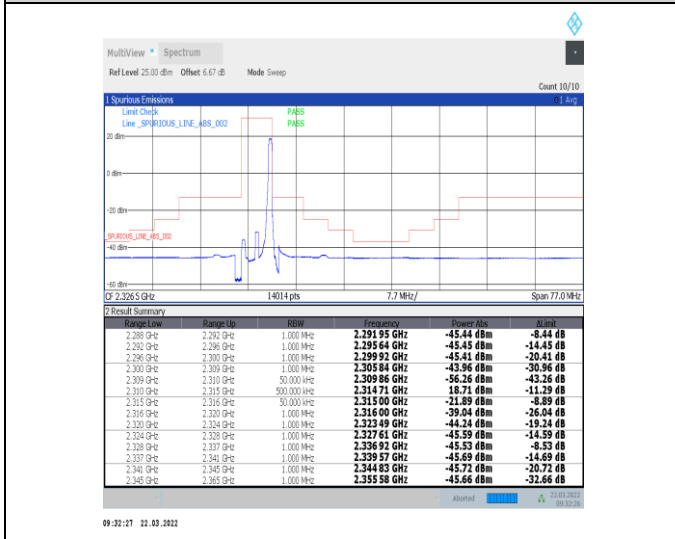
1-N30-15-5-H-5-CP-QPSK-Edge_1RB_Right-1@24-A nt1-PASS-see graph
