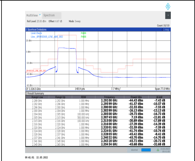
1-N30-15-10-M-6-CP-QPSK-Outer_Full-52@0-Ant1-PASS-see graph
