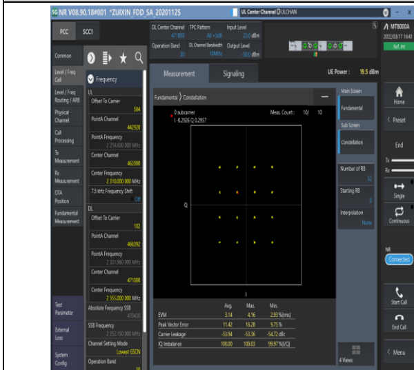
1-N30-15-10-M-7-CP-16QAM-Outer_Full-52@0-Ant1-see graph-PASS
