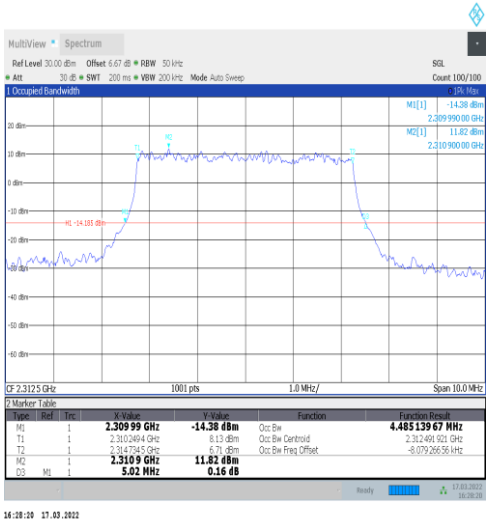
1-N30-15-5-H-3-DFT-16QAM-Outer_Full-25@0-Ant1 -4.485-5.020-≤5-PASS
