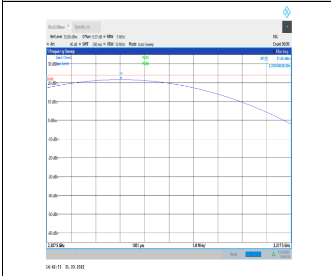
1-N30-PC3-15-5-H-1-DFT-PI2BPSK-Inner_1RB_Lef t-1@1-2307.5-2317.5-Ant1-21.62-23.98-PASS
