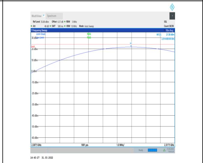
1-N30-PC3-15-5-H-2-DFT-PI2BPSK-Inner_1RB_Righ t-1@23-2307.5-2317.5-Ant1-21.58-23.98-PASS
