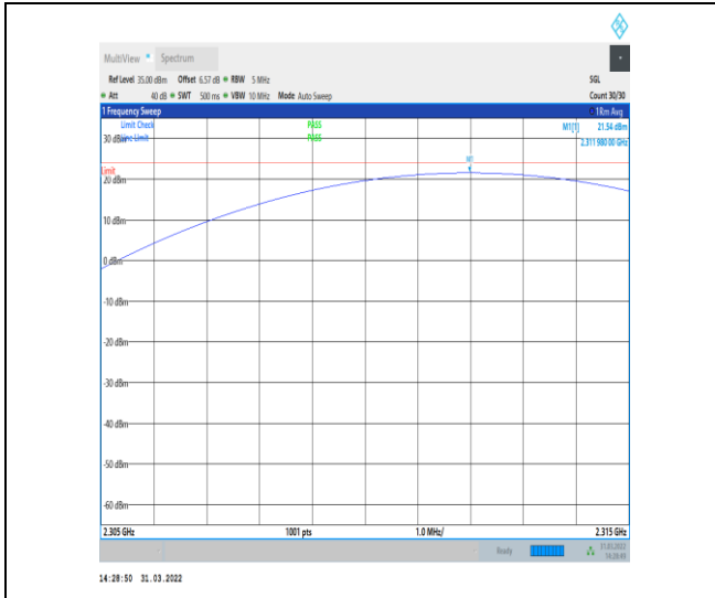
1-N30-PC3-15-5-M-2-DFT-PI2BPSK-Inner_1RB_Rig ht-1@23-2305-2315-Ant1-21.54-23.98-PASS
