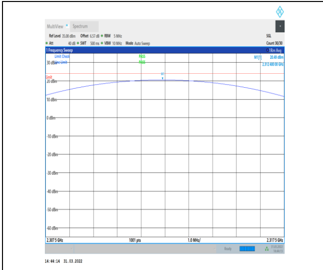
1-N30-PC3-15-5-H-3-DFT-PI2BPSK-Outter_Full-25 @0-2307.5-2317.5-Ant1-20.49-23.98-PASS
