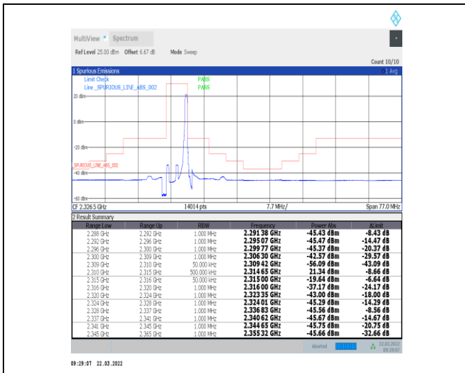
1-N30-15-5-H-2-DFT-PI2BPSK-Edge_1RB_Right-1@2 4-Ant1-PASS-see graph
