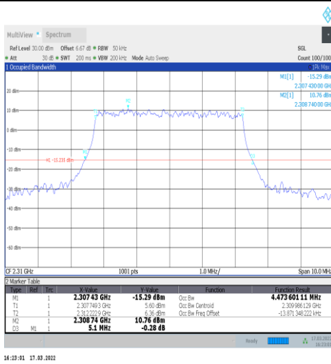
1-N30-15-5-M-4-DFT-64QAM-Outer_Full-25@0-Ant1 -4.474-5.100-≤5-PASS
