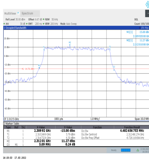
1-N30-15-5-H-4-DFT-64QAM-Outer_Full-25@0-Ant1 -4.483-5.090-≤5-PASS
