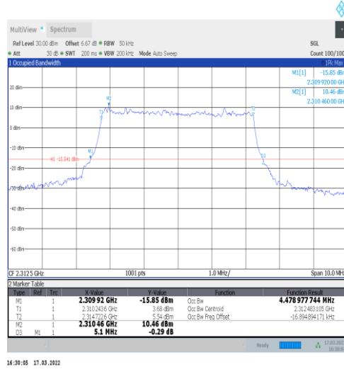
1-N30-15-5-H-6-CP-QPSK-Outer_Full-25@0-Ant1-4. 479-5.100-≤5-PASS
