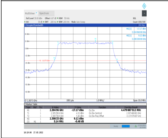
1-N30-15-5-L-7-CP-16QAM-Outer_Full-25@0-Ant1-4 .48-5.140-≤5-PASS
