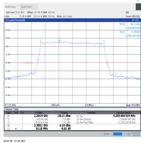
1-N30-15-10-M-9-CP-256QAM-Outer_Full-52@0-Ant1-9.293-10.180-≤10-PASS
