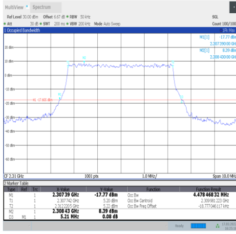
1-N30-15-5-M-8-CP-64QAM-Outer_Full-25@0-Ant1-4.478-5.210-≤5-PASS
