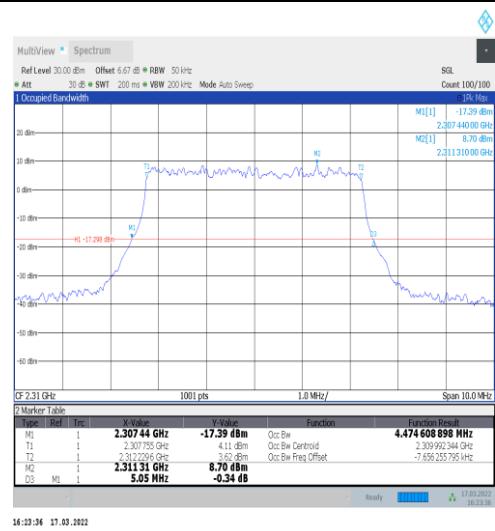
1-N30-15-5-M-5-DFT-256QAM-Outer_Full-25@0-Ant 1-4.475-5.050-≤5-PASS
