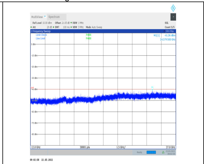
1-N30-15-10-M-1-DFT-PI2BPSK-Inner_1RB_Left-1@ 1-12000-27000-Ant1--41.36--40-PASS
