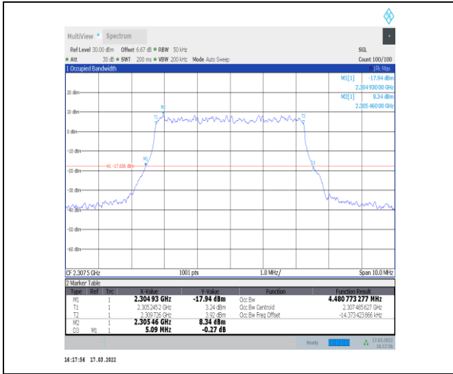
1-N30-15-5-L-5-DFT-256QAM-Outer_Full-25@0-Ant 1-4.481-5.090-≤5-PASS
