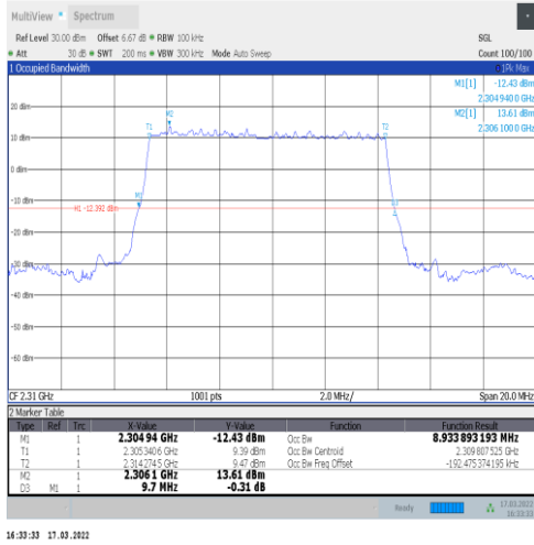
1-N30-15-10-M-2-DFT-PI2BPSK-Outer_Full-50@0-A nt1-8.934-9.700-≤10-PASS
