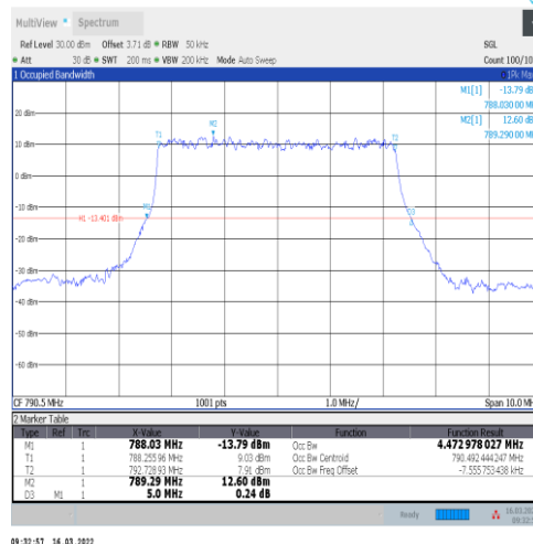
1-N14-15-5-L-2-DFT-PI2BPSK-Outer_Full-25@0-Ant 1-4.473-5.000-≤5-PASS
