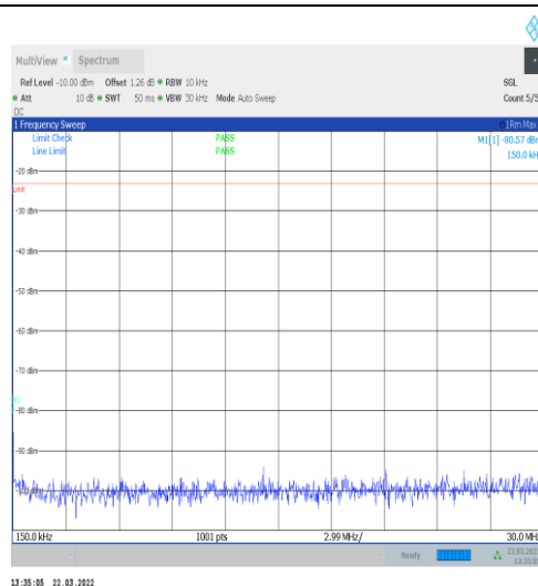
1-N14-15-10-M-1-DFT-PI2BPSK-Inner_1RB_Left-1 @1-0.15-30-Ant1--80.57--23-PASS
