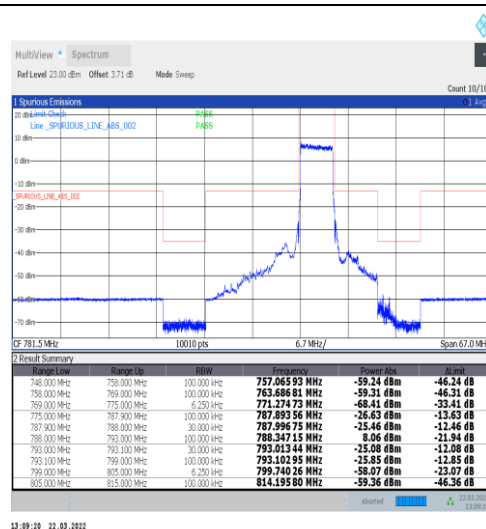
1-N14-15-5-L-3-DFT-PI2BPSK-Outer_Full-25@0-Ant1-PASS-see graph
