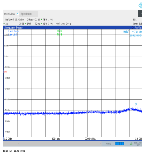
1-N14-15-10-M-1-DFT-PI2BPSK-Inner_1RB_Left-1 @1-1000-3000-Ant1--47.19--13-PASS
