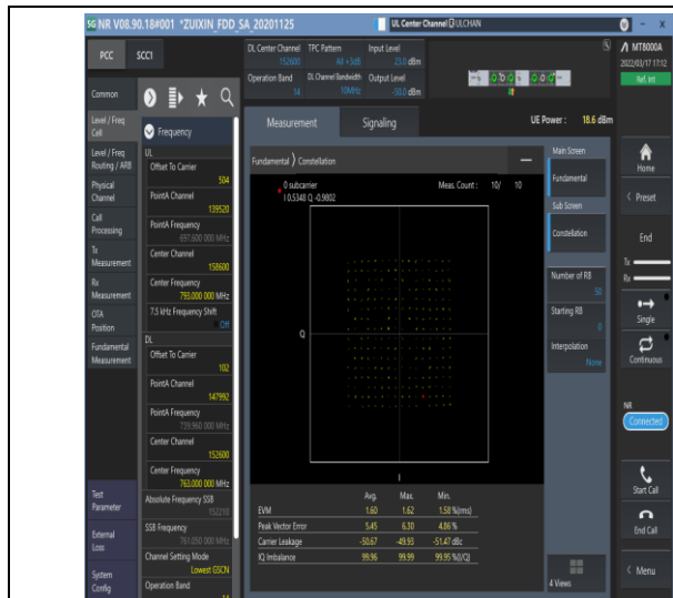
1-N14-15-10-M-5-DFT-256QAM-Outer_Full-50@0-Ant1-see graph-PASS
