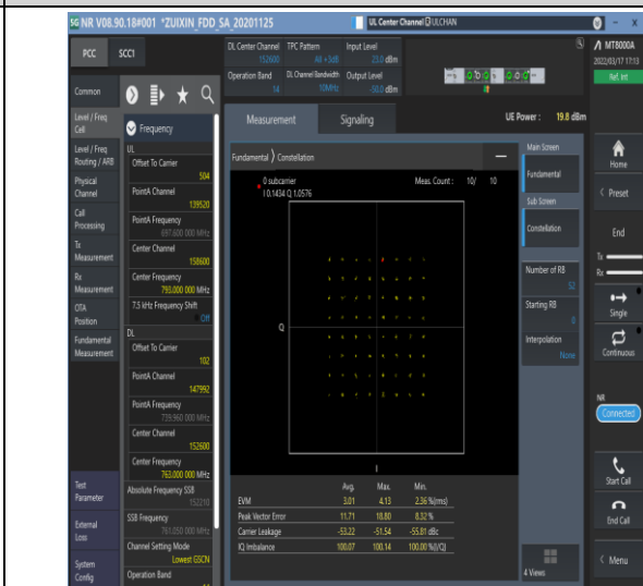
1-N14-15-10-M-8-CP-64QAM-Outer_Full-52@0-Ant1-see graph-PASS
