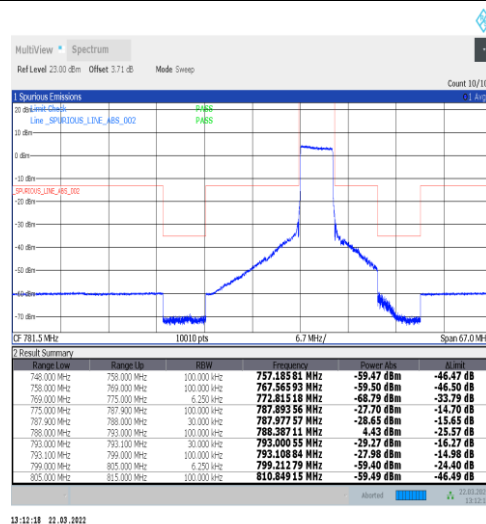
1-N14-15-5-L-6-CP-QPSK-Outer_Full-25@0-Ant1-PASS-see graph
