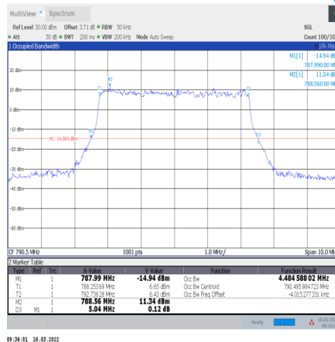
1-N14-15-5-L-4-DFT-64QAM-Outer_Full-25@0-Ant1 -4.485-5.040-≤5-PASS
