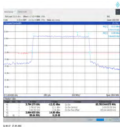
1-N77-3700-3980-30-90-M-4-DFT-64QAM-Outer_Full-240@0-Ant1-85.786-89.640-≤90-PASS
