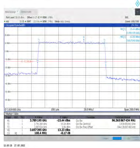
1-N77-3700-3980-30-100-M-5-DFT-256QAM-Outer_Full-270@0-Ant1-96.366-100.400-≤100-PASS
