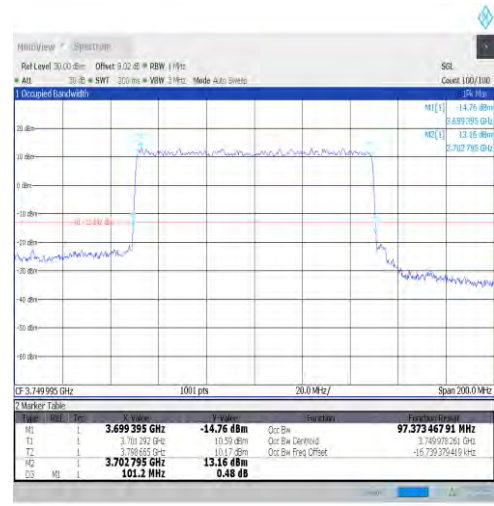
1-N77-3700-3980-30-100-L-6-CP-QPSK-Outer_Full- 273@0-Ant1-97.373-101.200-≤100-PASS
