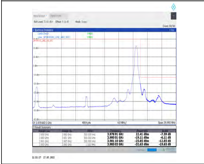
1-N77-3700-3980-30-30-H-5-CP-QPSK-Edge_1RB_Right-1@77-Ant1-PASS-see graph
