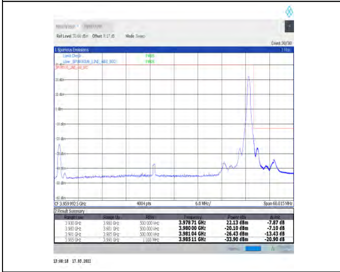
1-N77-3700-3980-30-50-H-5-CP-QPSK-Edge_1RB_Right-1@132-Ant1-PASS-see graph
