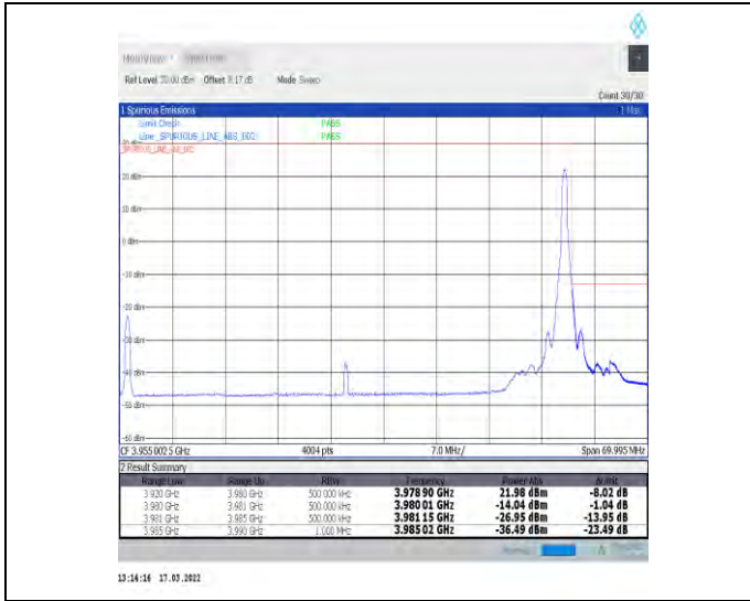
1-N77-3700-3980-30-60-H-2-DFT-PI2BPSK-Edge_1R_B_Right-1@161-Ant1-PASS-see graph
