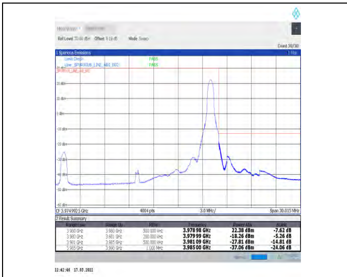
1-N77-3700-3980-30-20-H-2-DFT-PI2BPSK-Edge_1R_B_Right-1@50-Ant1-PASS-see graph
