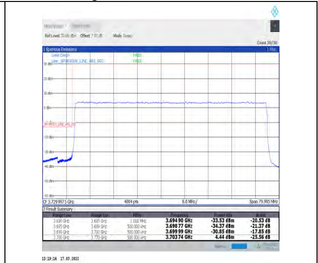
1-N77-3700-3980-30-70-L-3-DFT-PI2BPSK-Outer_Full-180@0-Ant1-PASS-see graph
