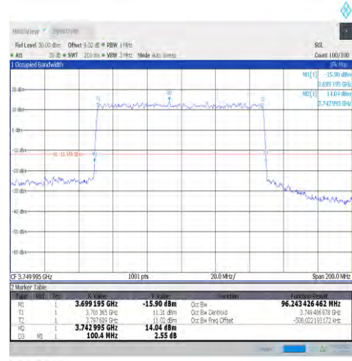
1-N77-3700-3980-30-100-L-4-DFT-64QAM-Outer_F ull-270@0-Ant1-96.243-100.400-≤100-PASS
