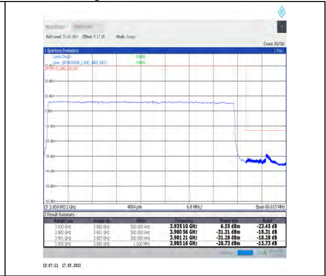
1-N77-3700-3980-30-50-H-3-DFT-PI2BPSK-Outer_Full-128@0-Ant1-PASS-see graph
