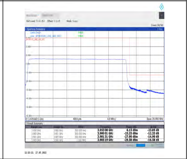
1-N77-3700-3980-30-30-H-6-CP-QPSK-Outer_Full-78@0-Ant1-PASS-see graph
