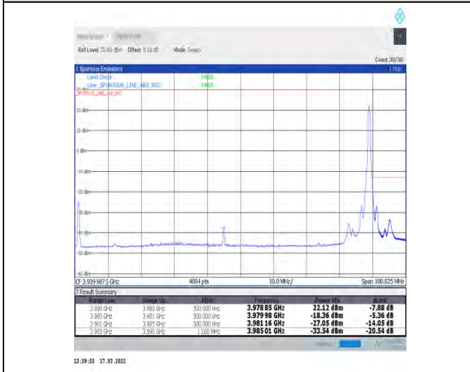
1-N77-3700-3980-30-90-H-5-CP-QPSK-Edge_1RB_Right-1@244-Ant1-PASS-see graph
