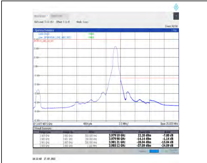
1-N77-3700-3980-30-15-H-2-DFT-PI2BPSK-Edge_1R_B_Right-1@37-Ant1-PASS-see graph
