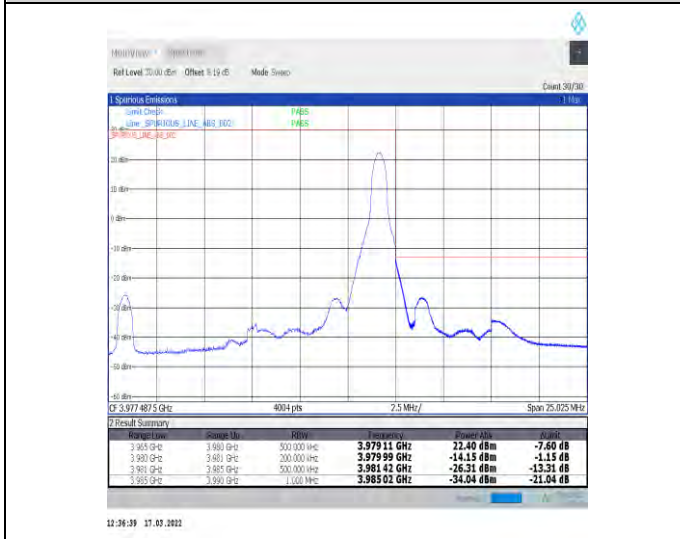
1-N77-3700-3980-30-15-H-5-CP-QPSK-Edge_1RB_Right-1@37-Ant1-PASS-see graph
