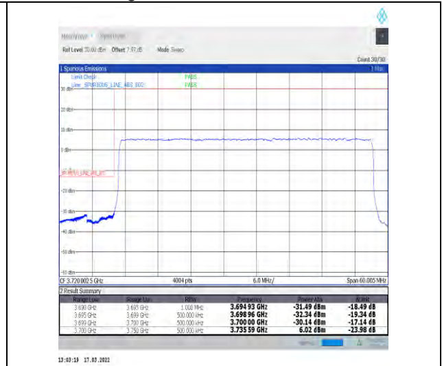
1-N77-3700-3980-30-50-L-3-DFT-PI2BPSK-Outer_Full-128@0-Ant1-PASS-see graph
