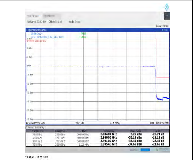
1-N77-3700-3980-30-100-H-6-CP-QPSK-Outer_Full-273@0-Ant1-PASS-see graph
