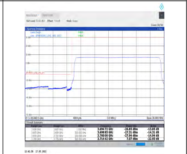
1-N77-3700-3980-30-20-L-6-CP-QPSK-Outer_Full-51@0-Ant1-PASS-see graph
