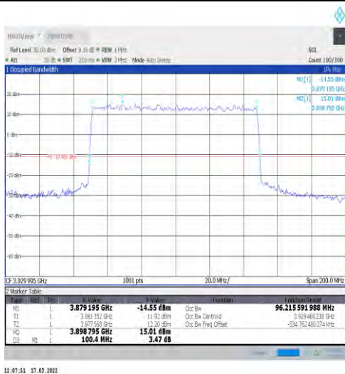
1-N77-3700-3980-30-100-H-3-DFT-16QAM-Outer_Full Full-270@0-Ant1-96.216-100.400-≤100-PASS
