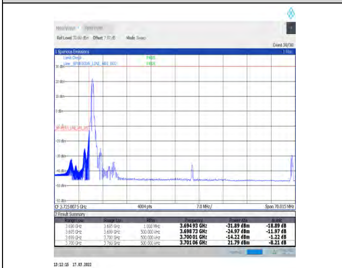
1-N77-3700-3980-30-60-L-4-CP-QPSK-Edge_1RB_Lef t-1@0-Ant1-PASS-see graph
