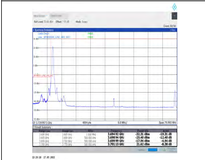
1-N77-3700-3980-30-70-L-4-CP-QPSK-Edge_1RB_Lef-t-1@0-Ant1-PASS-see graph
