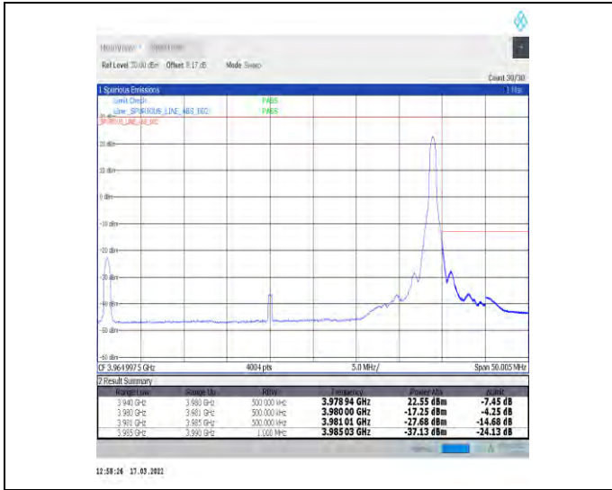
1-N77-3700-3980-30-40-H-2-DFT-PI2BPSK-Edge_1R_B_Right-1@105-Ant1-PASS-see graph
