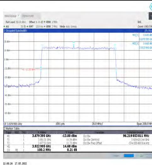
1-N77-3700-3980-30-100-H-4-DFT-64QAM-Outer_Full Full-270@0-Ant1-96.22-100.200-≤100-PASS
