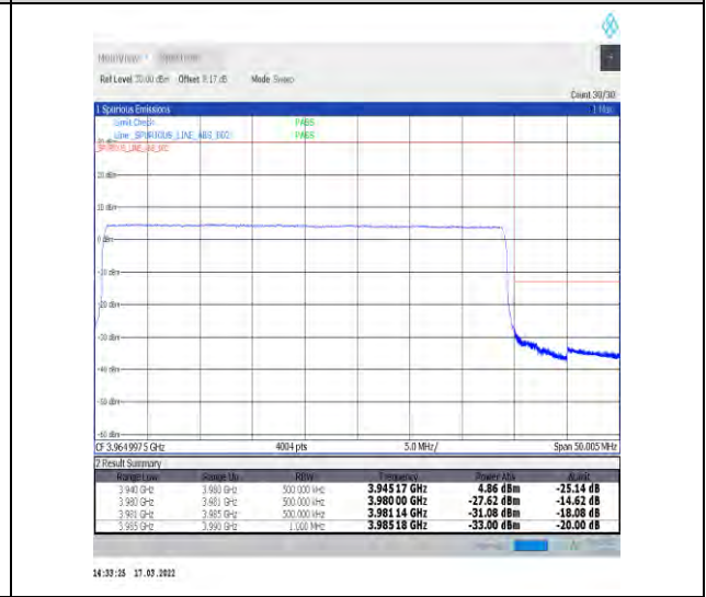
1-N77-3700-3980-30-40-H-6-CP-QPSK-Outer_Full-106@0-Ant1-PASS-see graph
