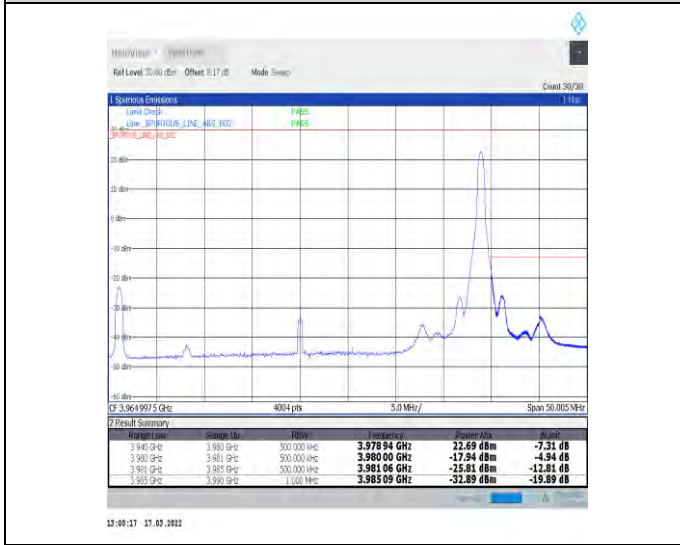
1-N77-3700-3980-30-40-H-5-CP-QPSK-Edge_1RB_Right-1@105-Ant1-PASS-see graph
