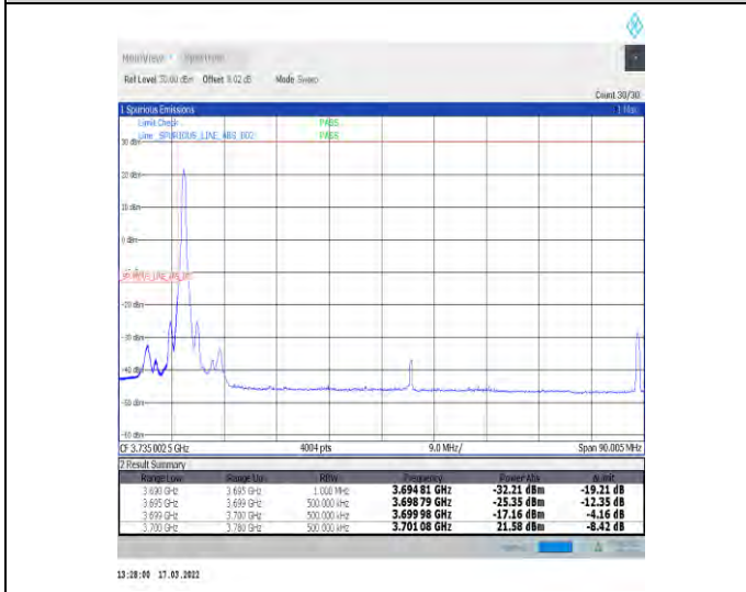
1-N77-3700-3980-30-80-L-4-CP-QPSK-Edge_1RB_Lef-t-1@0-Ant1-PASS-see graph
