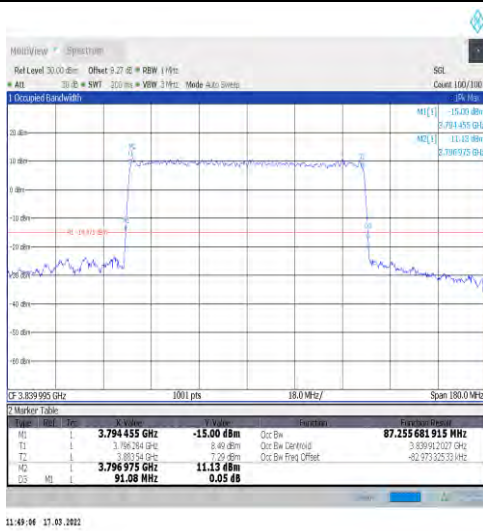
1-N77-3700-3980-30-90-M-9-CP-256QAM-Outer_Full-245@0-Ant1-87.256-91.080-≤90-PASS
