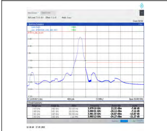
1-N77-3700-3980-30-10-H-5-CP-QPSK-Edge_1RB_Right-1@23-Ant1-PASS-see graph
