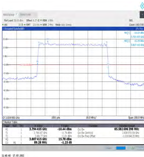
1-N77-3700-3980-30-90-M-3-DFT-16QAM-Outer_Full-240@0-Ant1-85.583-89.280-≤90-PASS
