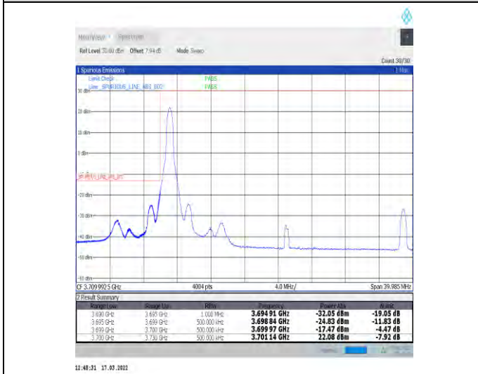
1-N77-3700-3980-30-30-L-4-CP-QPSK-Edge_1RB_Lef t-1@0-Ant1-PASS-see graph
