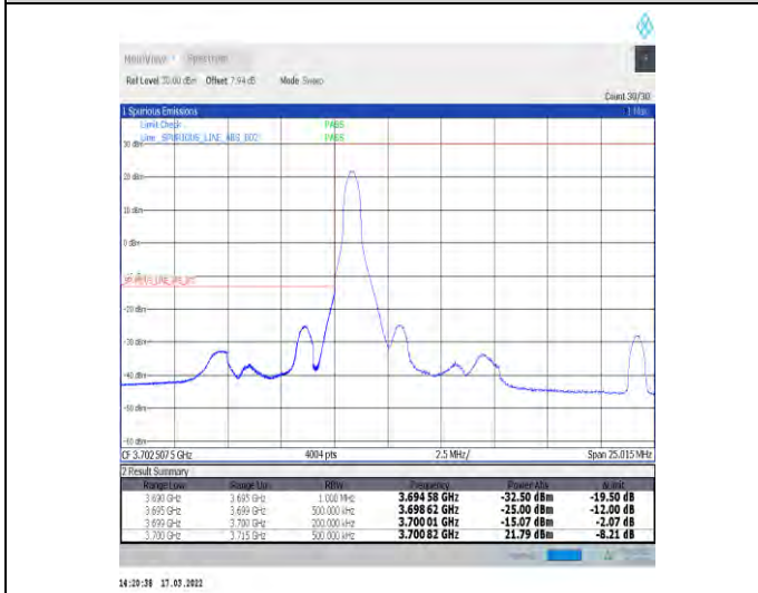
1-N77-3700-3980-30-15-L-4-CP-QPSK-Edge_1RB_Lef t-1@0-Ant1-PASS-see graph
