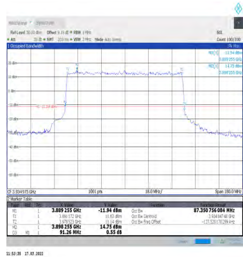
1-N77-3700-3980-30-90-H-7-CP-16QAM-Outer_Full-245@0-Ant1-87.351-91.260-≤90-PASS
