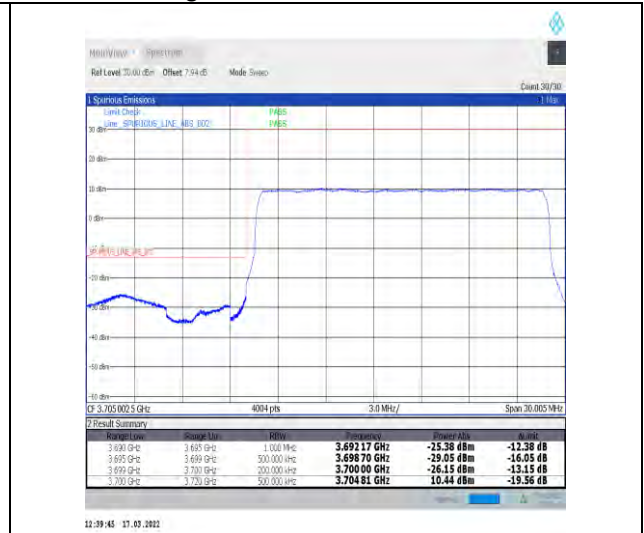
1-N77-3700-3980-30-20-L-3-DFT-PI2BPSK-Outer_Full-50@0-Ant1-PASS-see graph
