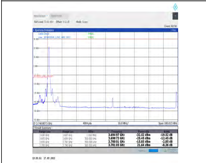
1-N77-3700-3980-30-90-L-4-CP-QPSK-Edge_1RB_Lef-t-1@0-Ant1-PASS-see graph
