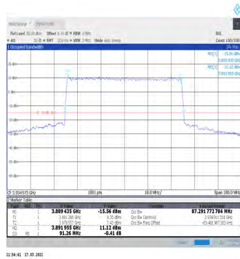
1-N77-3700-3980-30-90-H-9-CP-256QAM-Outer_Ful I-245@0-Ant1-87.292-91.260-≤90-PASS
