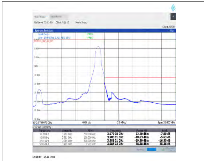
1-N77-3700-3980-30-10-H-2-DFT-PI2BPSK-Edge_1R_B_Right-1@23-Ant1-PASS-see graph
