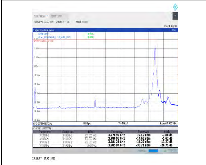
1-N77-3700-3980-30-60-H-5-CP-QPSK-Edge_1RB_Right-1@161-Ant1-PASS-see graph
