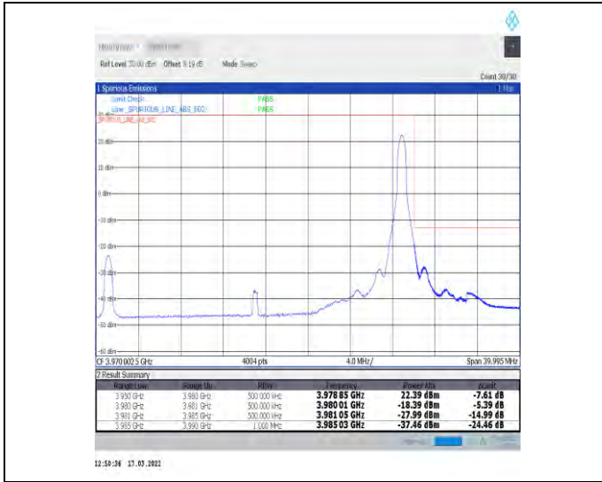
1-N77-3700-3980-30-30-H-2-DFT-PI2BPSK-Edge_1R_B_Right-1@77-Ant1-PASS-see graph
