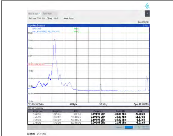
1-N77-3700-3980-30-40-L-1-DFT-PI2BPSK-Edge_1RB _Left-1@0-Ant1-PASS-see graph
