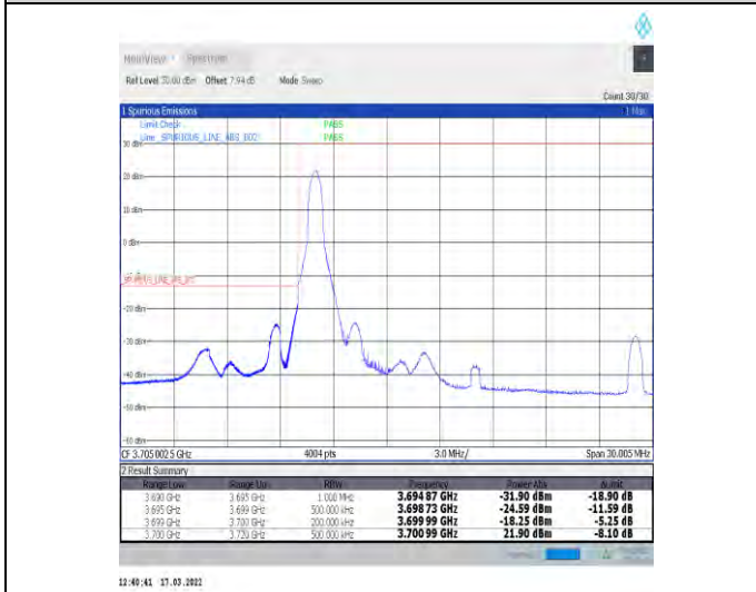
1-N77-3700-3980-30-20-L-4-CP-QPSK-Edge_1RB_Lef-t-1@0-Ant1-PASS-see graph
