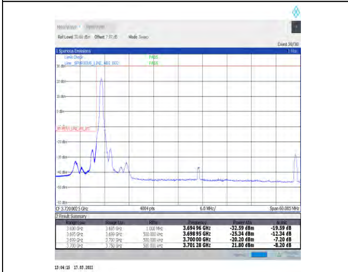
1-N77-3700-3980-30-50-L-4-CP-QPSK-Edge_1RB_Lef-t-1@0-Ant1-PASS-see graph
