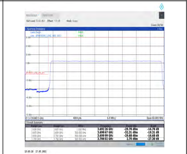
1-N77-3700-3980-30-50-L-6-CP-QPSK-Outer_Full-133@0-Ant1-PASS-see graph
