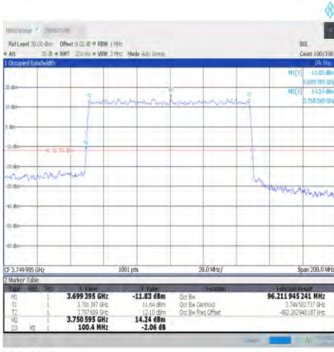
1-N77-3700-3980-30-100-L-3-DFT-16QAM-Outer_Fu ll-270@0-Ant1-96.212-100.400-≤100-PASS
