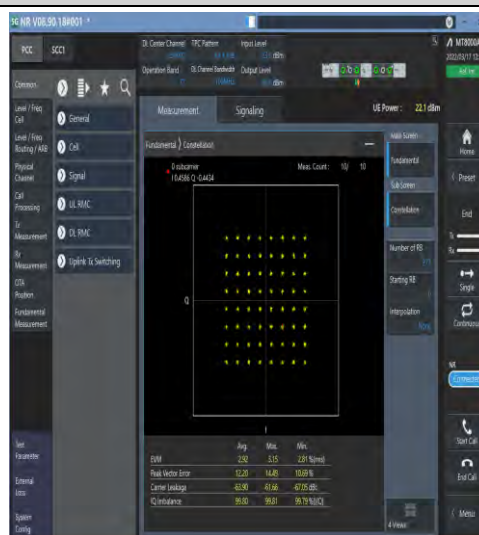
1-N77-3700-3980-30-100-M-8-CP-64QAM-Outer_Full-273@0-Ant1-see graph-PASS
