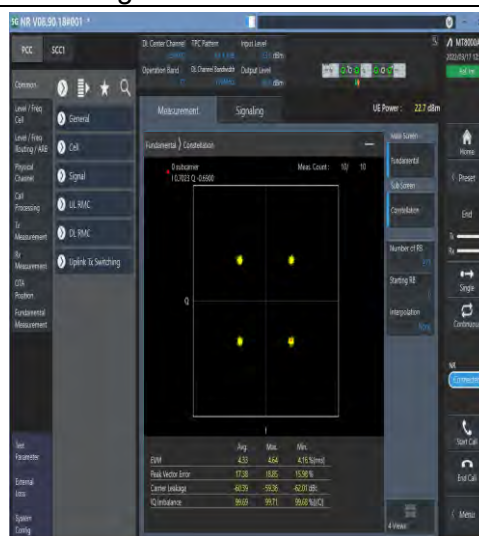
1-N77-3700-3980-30-100-M-6-CP-QPSK-Outer_Full-273@0-Ant1-see graph-PASS
