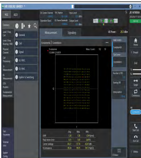
1-N77-3700-3980-30-100-M-5-DFT-256QAM-Outer_Full-270@0-Ant1-see graph-PASS
