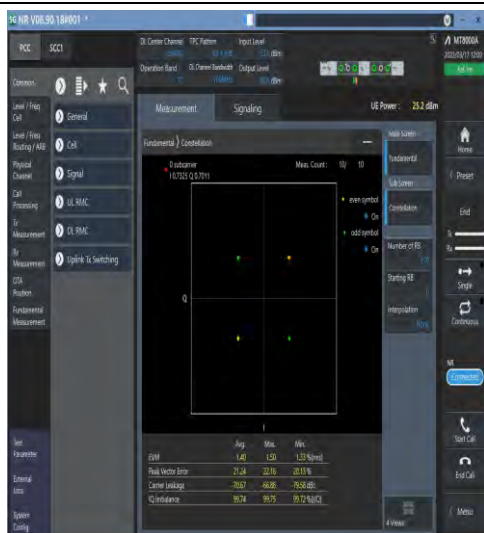
1-N77-3700-3980-30-100-M-1-DFT-PI2BPSK-Out-er_Full-270@0-Ant1-see graph-PASS
