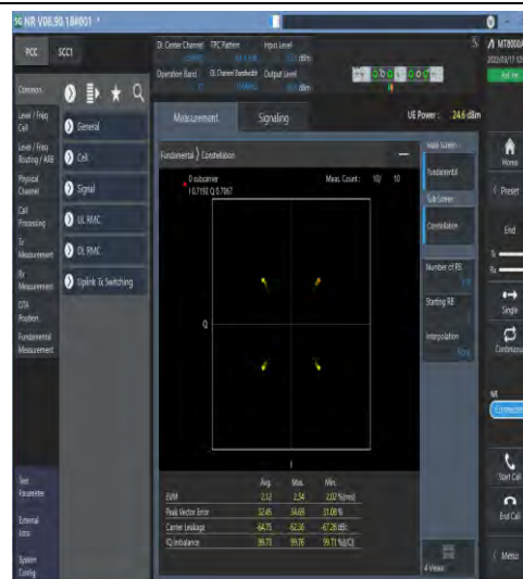
1-N77-3700-3980-30-100-M-2-DFT-QPSK-Out-er_Full-270@0-Ant1-see graph-PASS
