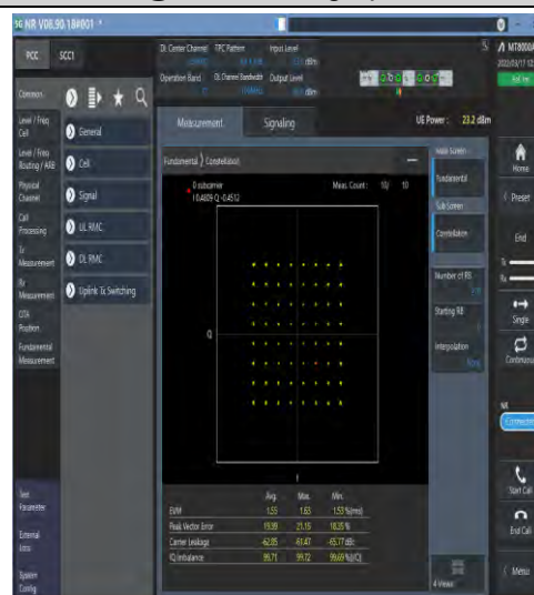
1-N77-3700-3980-30-100-M-4-DFT-64QAM-Out-er_Full-270@0-Ant1-see graph-PASS
