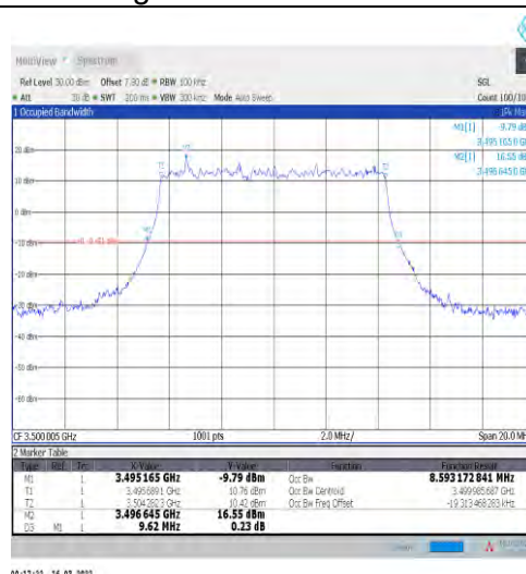
1-N77-3450-3550-30-10-M-1-DFT-QPSK-Outer_Full- 24@0-Ant1-8.593-9.620-≤10-PASS
