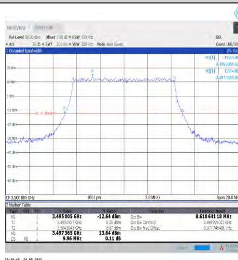
1-N77-3450-3550-30-10-M-3-DFT-16QAM-Outer_Full I-24@0-Ant1-8.611-9.960-≤10-PASS
