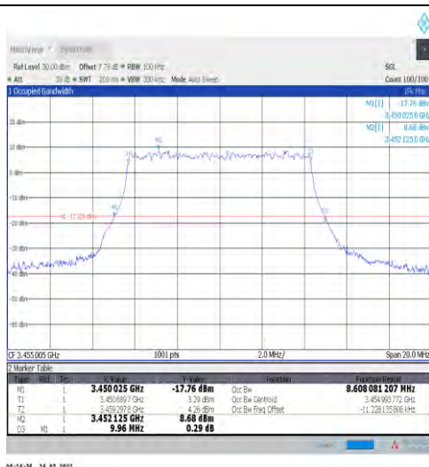
1-N77-3450-3550-30-10-L-9-CP-256QAM-Outer_Full -24@0-Ant1-8.608-9.960-≤10-PASS
