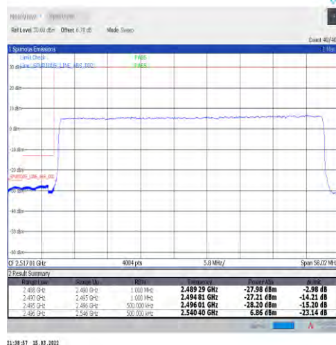
1-N41-30-50-L-3-DFT-PI2BPSK-Outer_Full-128@0-Ant1-PASS-see graph
