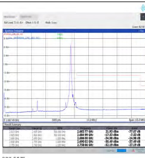
1-N41-30-70-H-2-DFT-PI2BPSK-Edge_1RB_Right-1@188-Ant1-PASS-see graph
