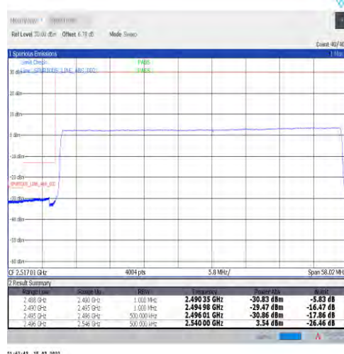
1-N41-30-50-L-6-CP-QPSK-Outer_Full-133@0-Ant1-PASS-see graph
