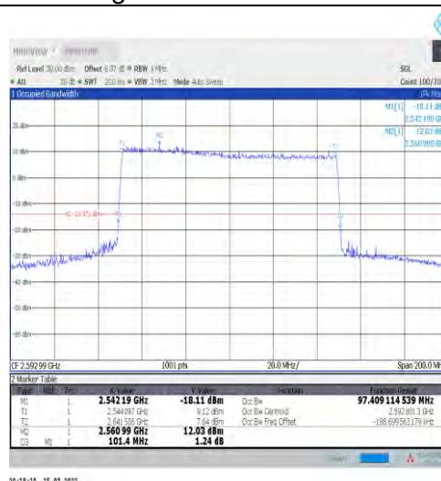
1-N41-30-100-M-9-CP-256QAM-Outer_Full-273@0-A Ant1-97.409-101.400-≤100-PASS
