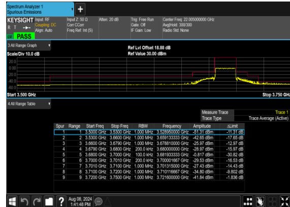
N48(20M)_CP- OFDM_QPSK_Outer_Full_High_CH
