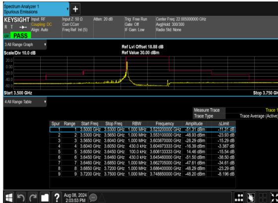
N48(40M)_CP- OFDM_QPSK_Edge_1RB_Left_Mid_CH
