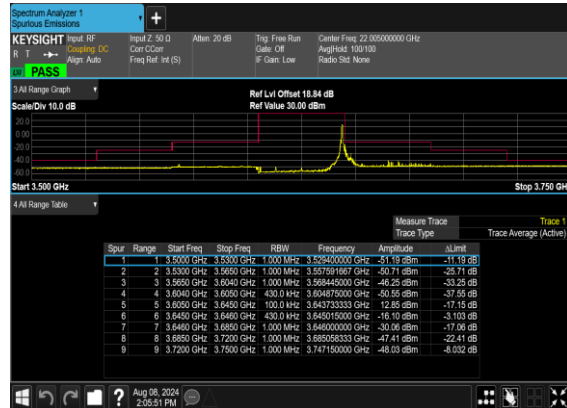
N48(40M)_CP- OFDM_QPSK_Edge_1RB_Right_Mid_CH
