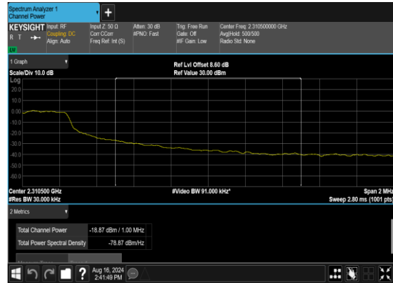
N30(5M)_DFT-s-OFDM_QPSK_Outer_Full_Low_CH_CHP_PASS
