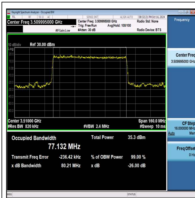
NTNV_N77-3450-3550_PC2_30_80_H_TID1_Ant1#1
