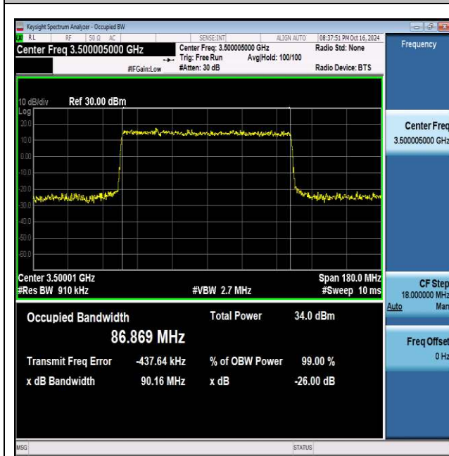
NTNV_N77-3450-3550_PC2_30_90_M_TID1_Ant1#1
