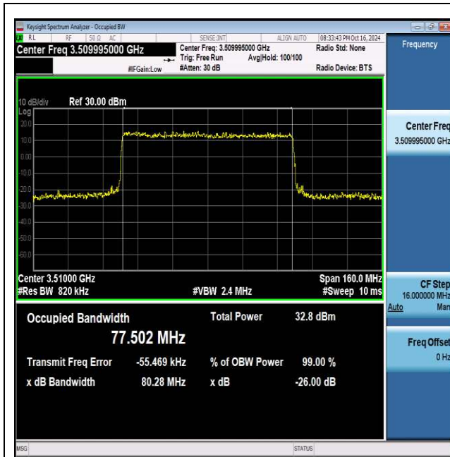
NTNV_N77-3450-3550_PC2_30_80_H_TID5_Ant1#1
