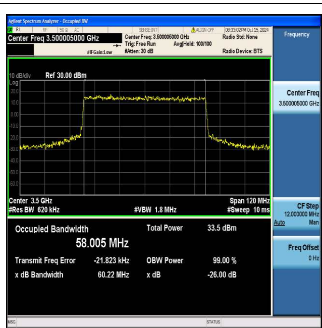
NTNV_N77-3450-3550_PC2_30_60_M_TID2_Ant1#1
