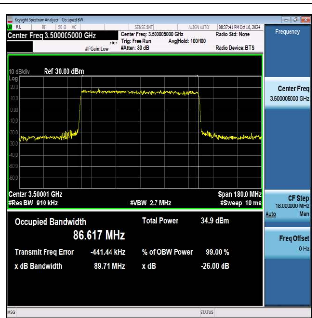
NTNV_N77-3450-3550_PC2_30_90_M_TID2_Ant1#1
