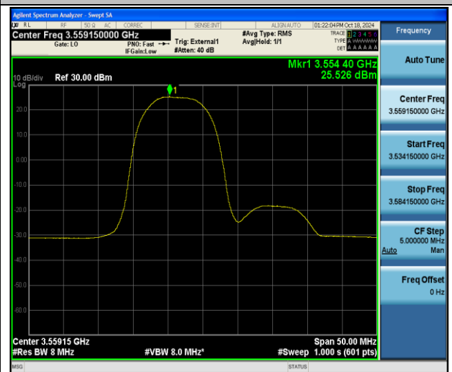
48-48-5MHz-20MHz-QPSK-QPSK-55273-55390-1RB#24-ORB#0- PASS
