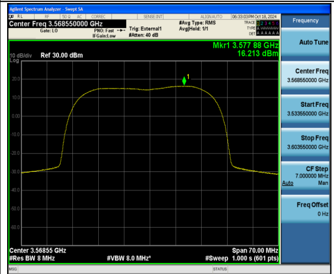
48-48-20MHz-15MHz-QPSK-QPSK-55340-55511-100RB#0- 75RB#0-PASS
