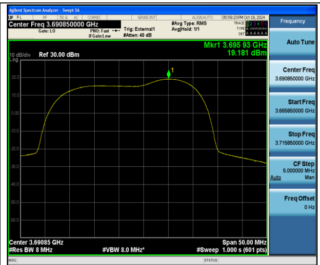
48-48-20MHz-5MHz-QPSK-QPSK-56590-56707-100RB#0- 25RB#0-PASS
