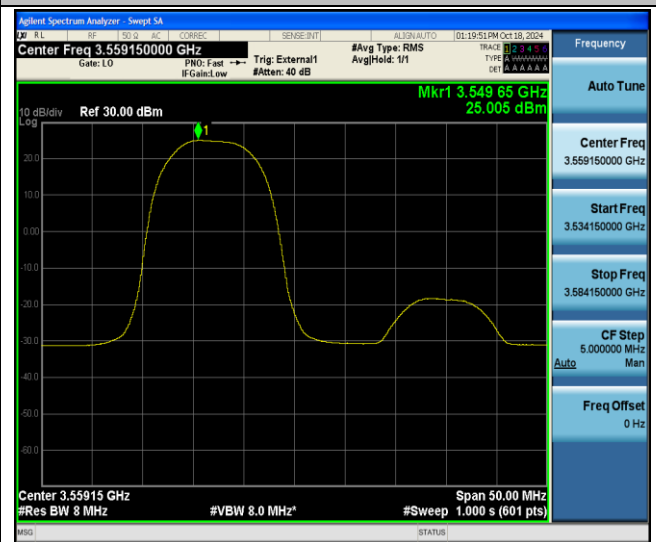
48-48-5MHz-20MHz-QPSK-QPSK-55273-55390-1RB#0-ORB#0- PASS
