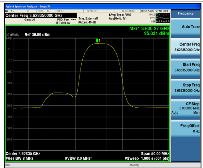
48-48-20MHz-5MHz-QPSK-QPSK-55965-56082-1RB#99-0RB#0- PASS
