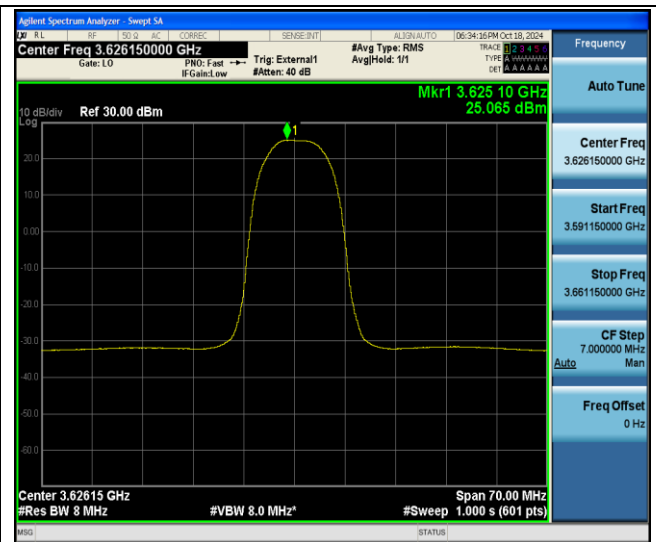
48-48-20MHz-15MHz-QPSK-QPSK-55916-56087-1RB#99- ORB#0-PASS
