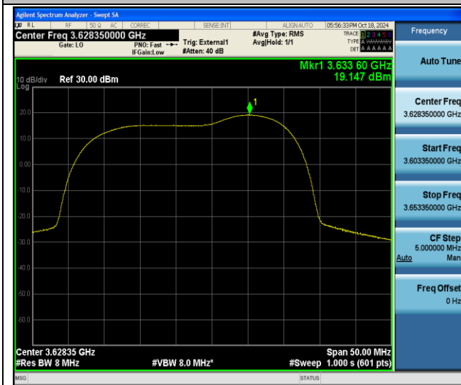
48-48-20MHz-5MHz-QPSK-QPSK-55965-56082-100RB#0- 25RB#0-PASS
