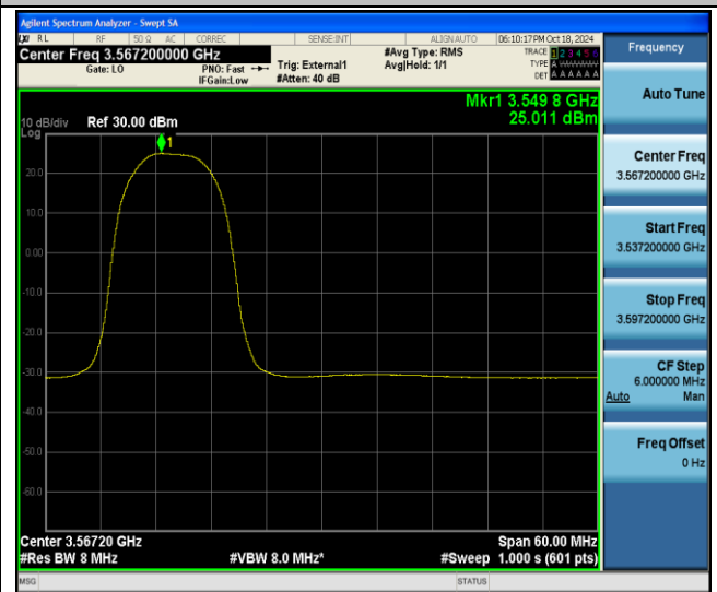
48-48-20MHz-10MHz-QPSK-QPSK-55340-55484-1RB#0-0RB#0- PASS
