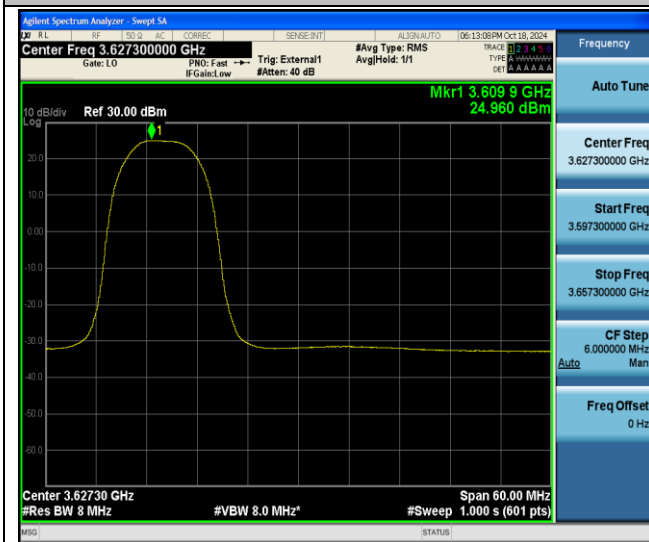
48-48-20MHz-10MHz-QPSK-QPSK-55941-56085-1RB#0-0RB#0- PASS
