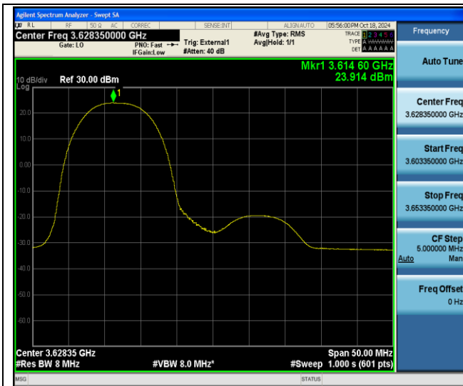
48-48-20MHz-5MHz-QPSK-QPSK-55965-56082-18RB#0-0RB#0- PASS
