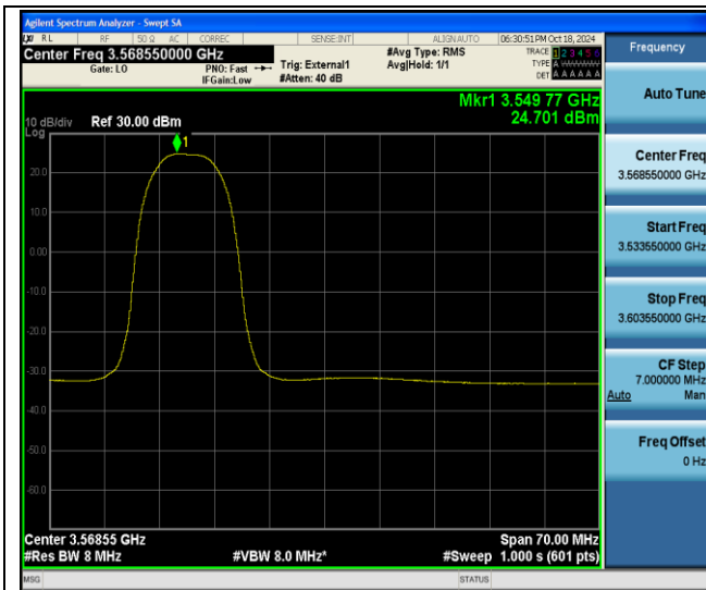
48-48-20MHz-15MHz-QPSK-QPSK-55340-55511-1RB#0-0RB#0- PASS
