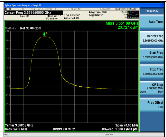
48-48-20MHz-15MHz-QPSK-QPSK-55340-55511-18RB#0- ORB#0-PASS
