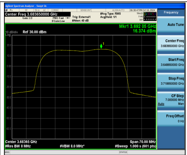
48-48-20MHz-15MHz-QPSK-QPSK-56491-56662-100RB#0- 75RB#0-PASS
