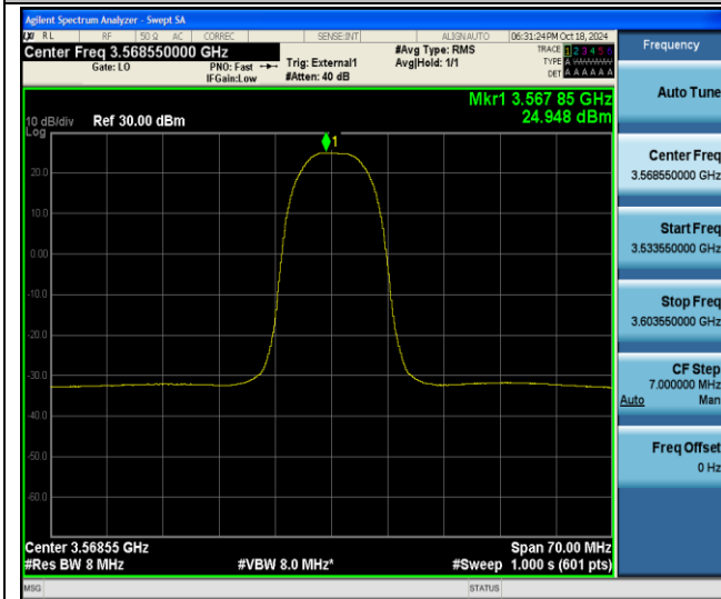
48-48-20MHz-15MHz-QPSK-QPSK-55340-55511-1RB#99- ORB#0-PASS
