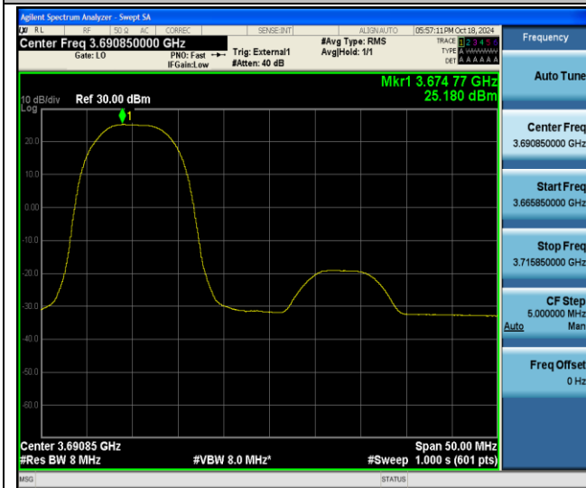
48-48-20MHz-5MHz-QPSK-QPSK-56590-56707-1RB#0-0RB#0- PASS
