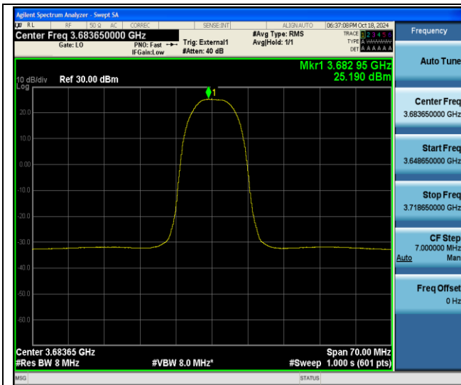
48-48-20MHz-15MHz-QPSK-QPSK-56491-56662-1RB#99- ORB#0-PASS
