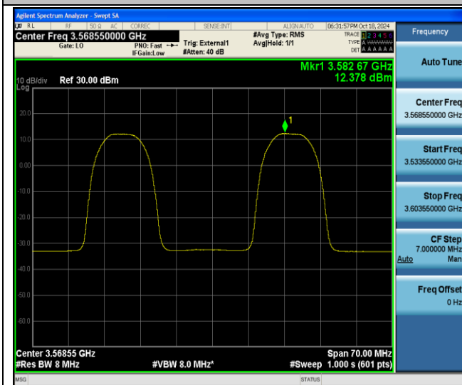
48-48-20MHz-15MHz-QPSK-QPSK-55340-55511-1RB#0- 1RB#74-PASS
