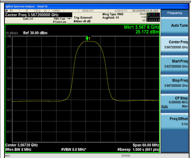
48-48-20MHz-10MHz-QPSK-QPSK-55340-55484-1RB#99- ORB#0-PASS
