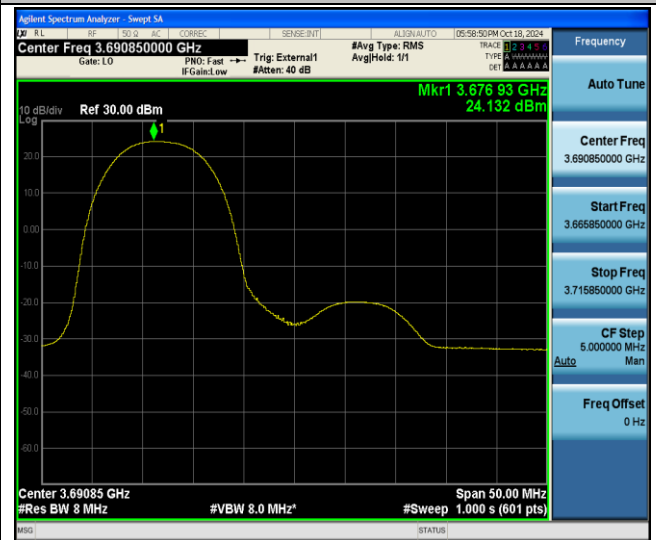
48-48-20MHz-5MHz-QPSK-QPSK-56590-56707-18RB#0-0RB#0- PASS
