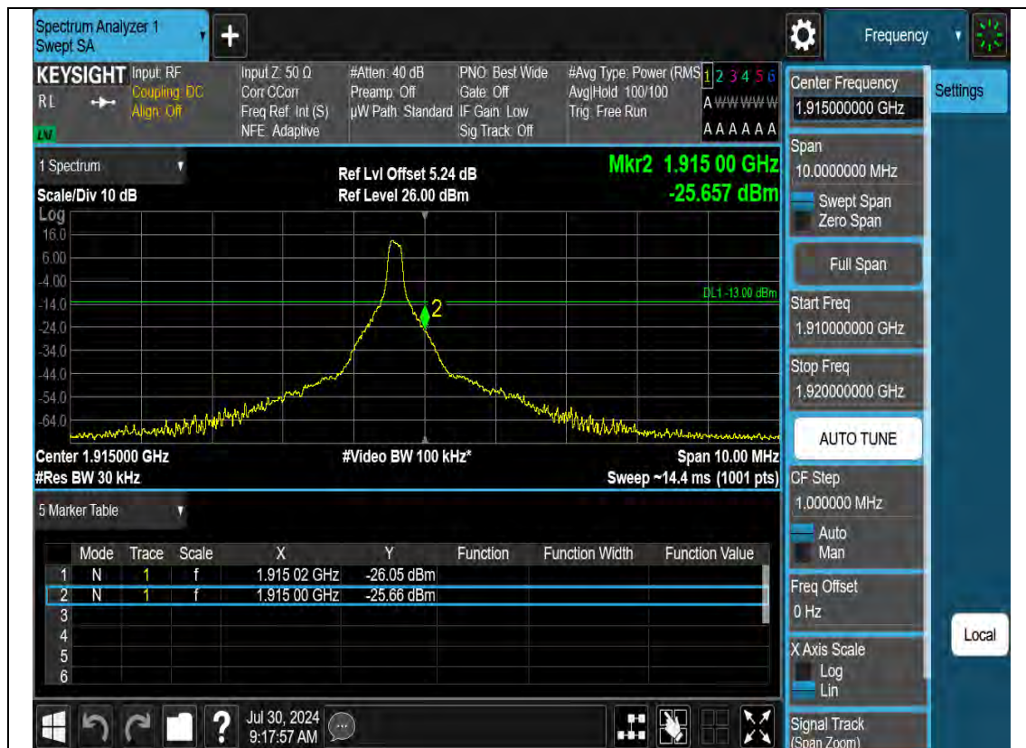
N25-10M-Bandedge-H-CP-OFDM-QPSK-Outer Full
