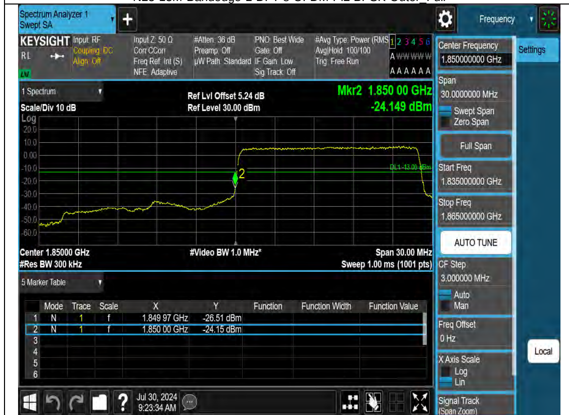
N25-15M-Bandedge-L-DFT-s-OFDM-Pi2 BPSK-1RB0
