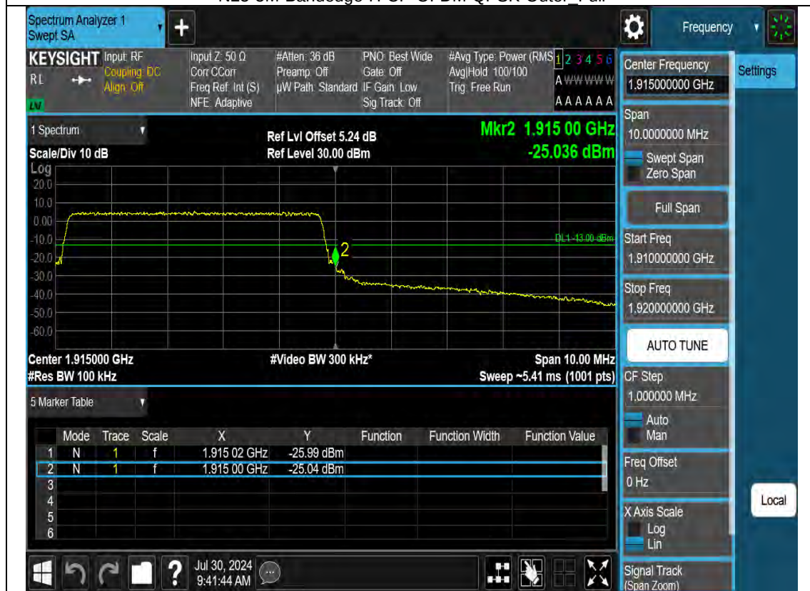
N25-5M-Bandedge-H-CP-OFDM-QPSK-1RB MAX
