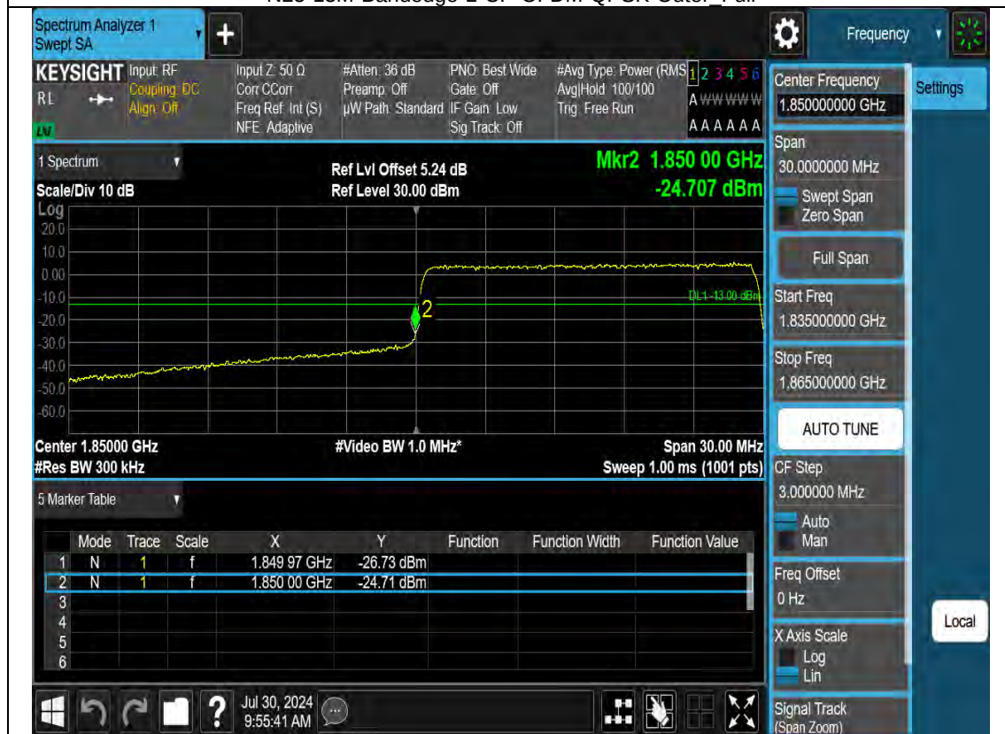
N25-15M-Bandedge-L-CP-OFDM-QPSK-1RB0
