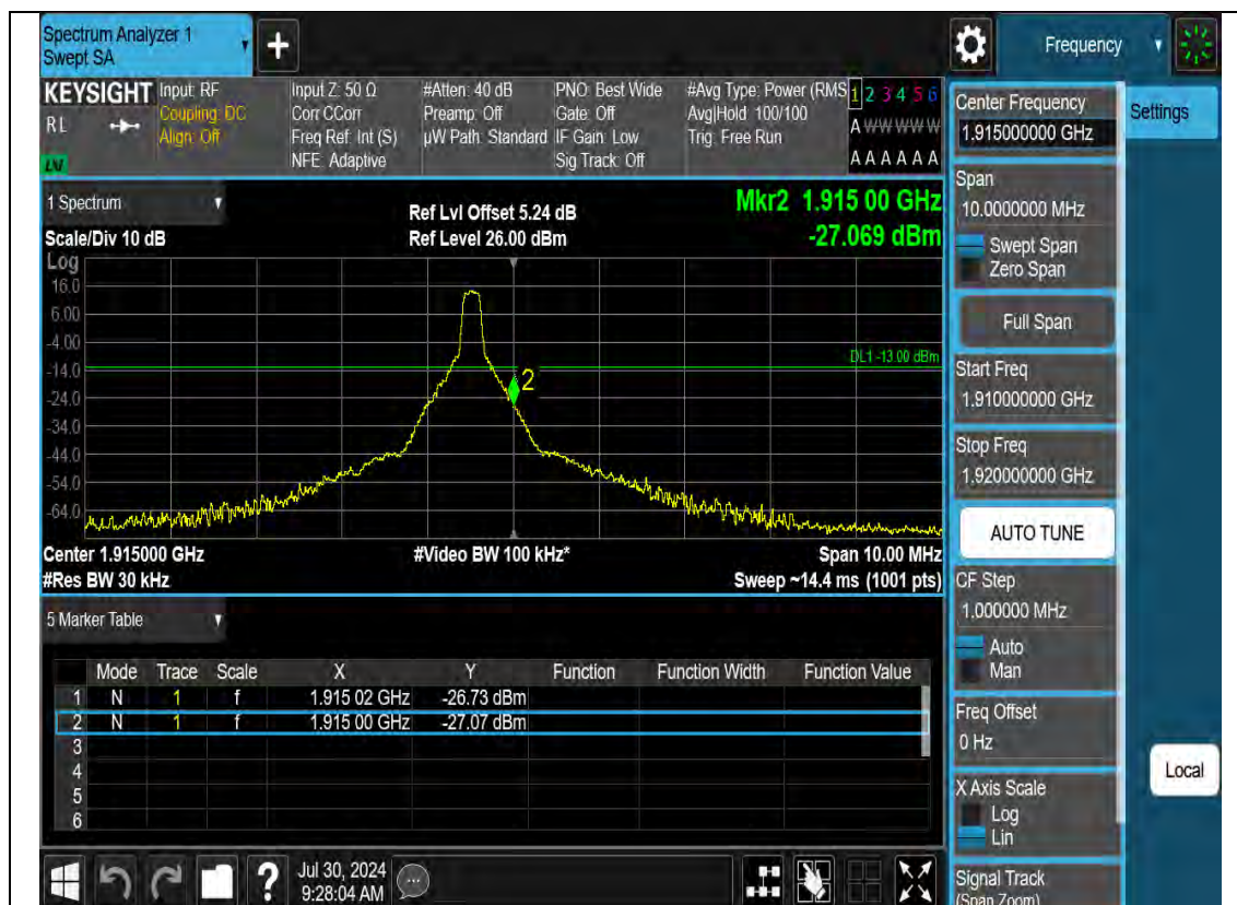
N25-15M-Bandedge-H-CP-OFDM-QPSK-Outer Full
