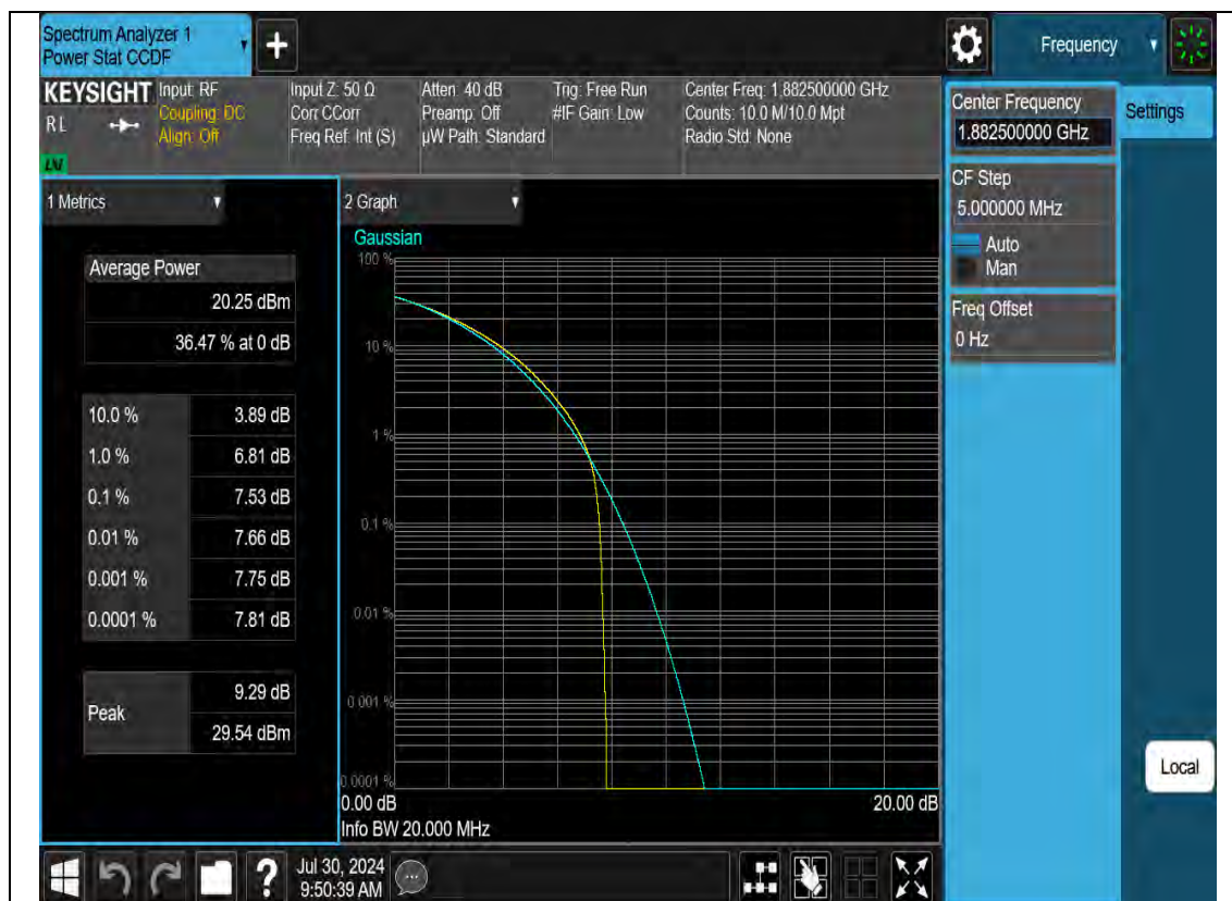
N25-10M-PAPR-H-DFT-s-OFDM-Pi2 BPSK-Outter Full
