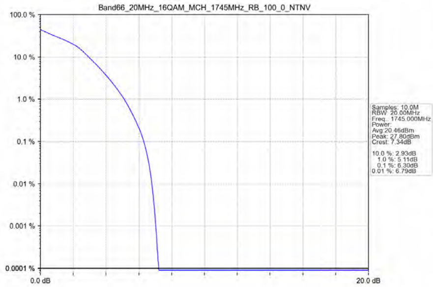
Band66_20MHz_16QAM_MCH_1745MHz_RB_100_0_NTNV
