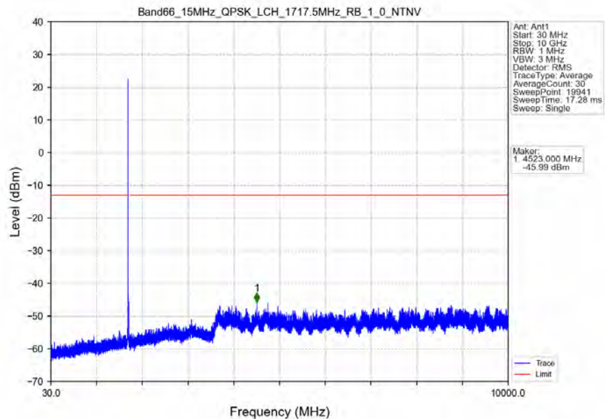
Band66_15MHz_QPSK_LCH_1717.5MHz_RB_1_0_NTNV
