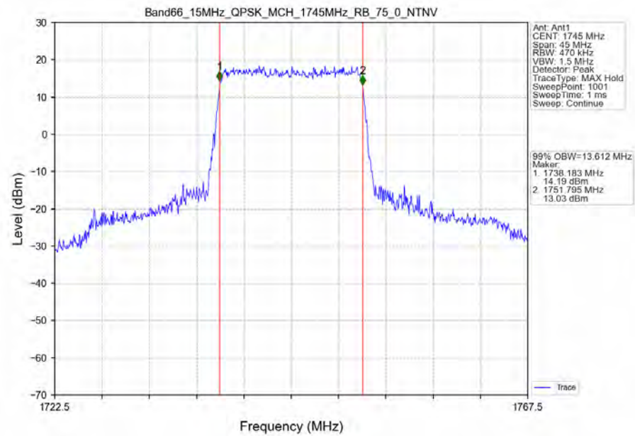
Band66_15MHz_QPSK_MCH_1745MHz_RB_75_0_NTNV
