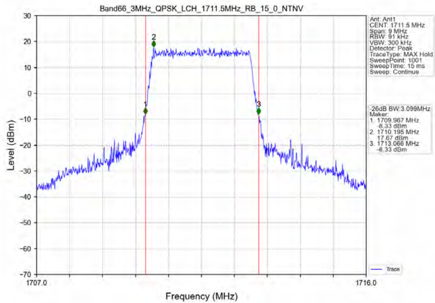
Band66_3MHz_QPSK_LCH_1711.5MHz_RB_15_0_NTNV
