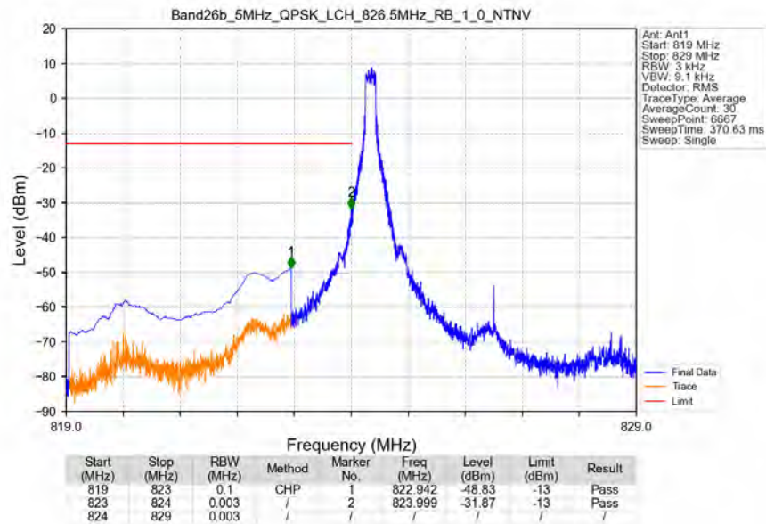
Band26b 5MHz QPSK LCH 826.5MHz RB 1_0 NTN
