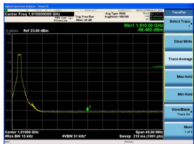
LTE Band 2 1.4MHz 16QAM 1RB CH-High
