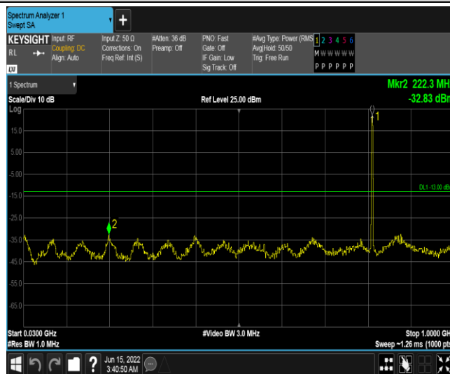
Band26-1.4MHz-QPSK-26697-1RB#0-Range1:30~1000MHz
