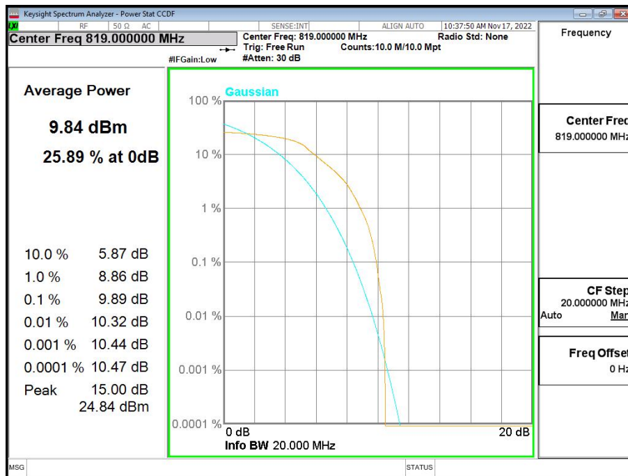
Band26-CH26740-819MHz-3MHz Bandwidth-QPSK
