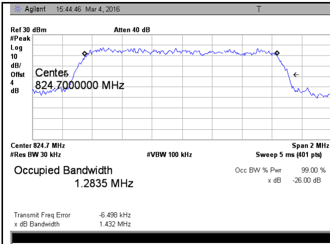
Cellular Band - Low CH
