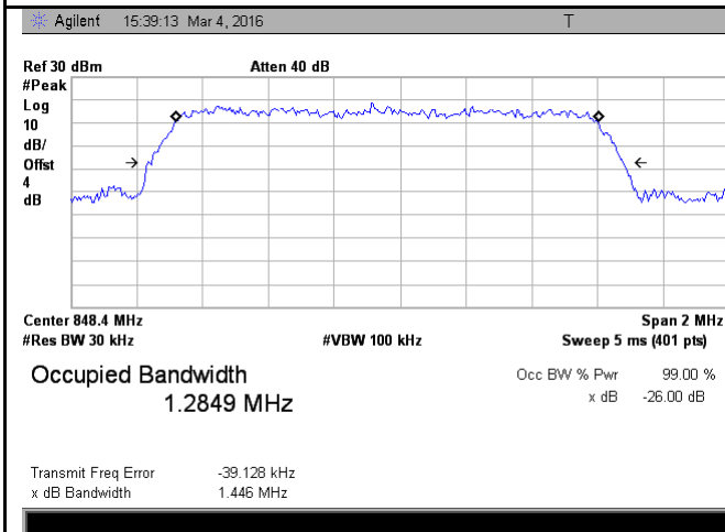
Cellular Band - High CH
