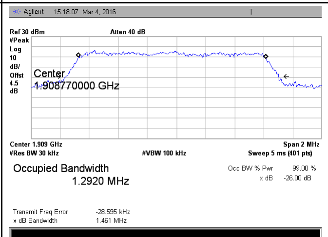
PCS Band - High CH
