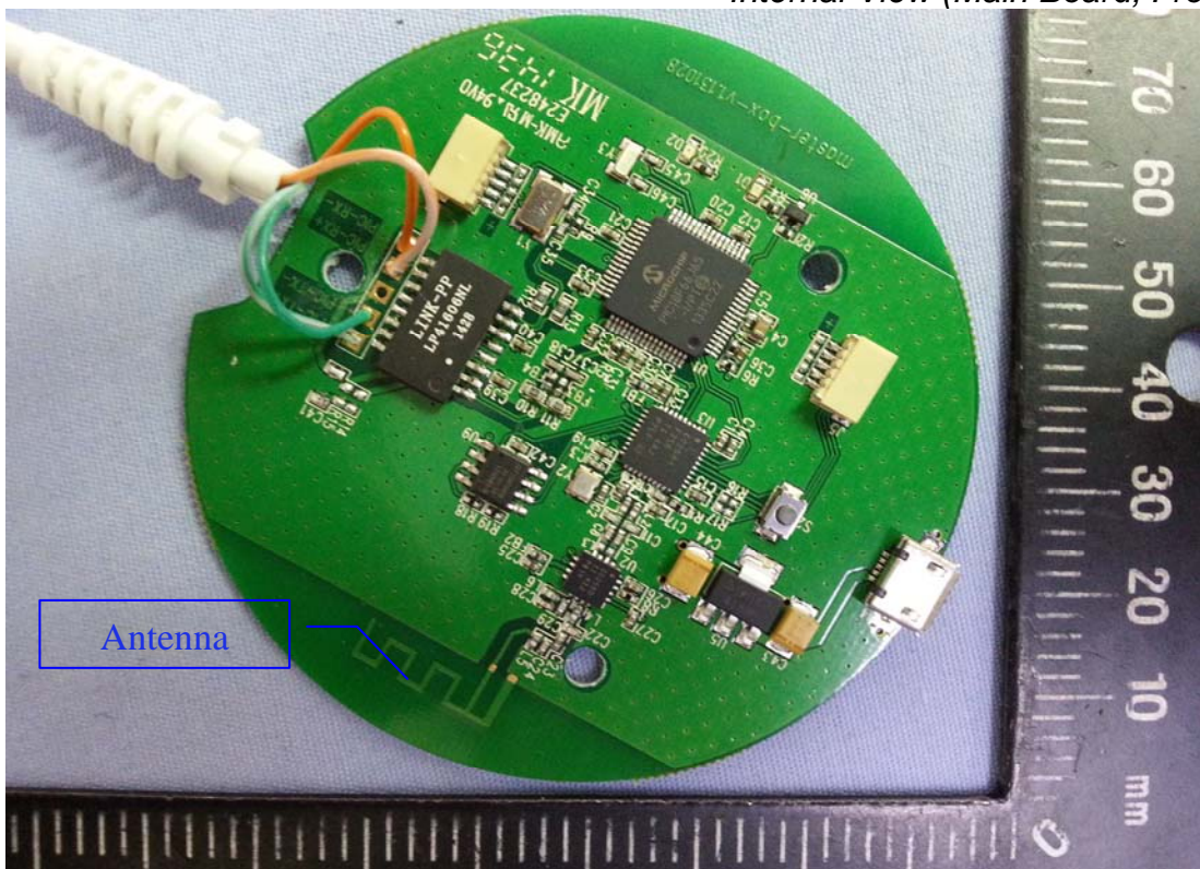
Internal View (Main Board, Front View)
