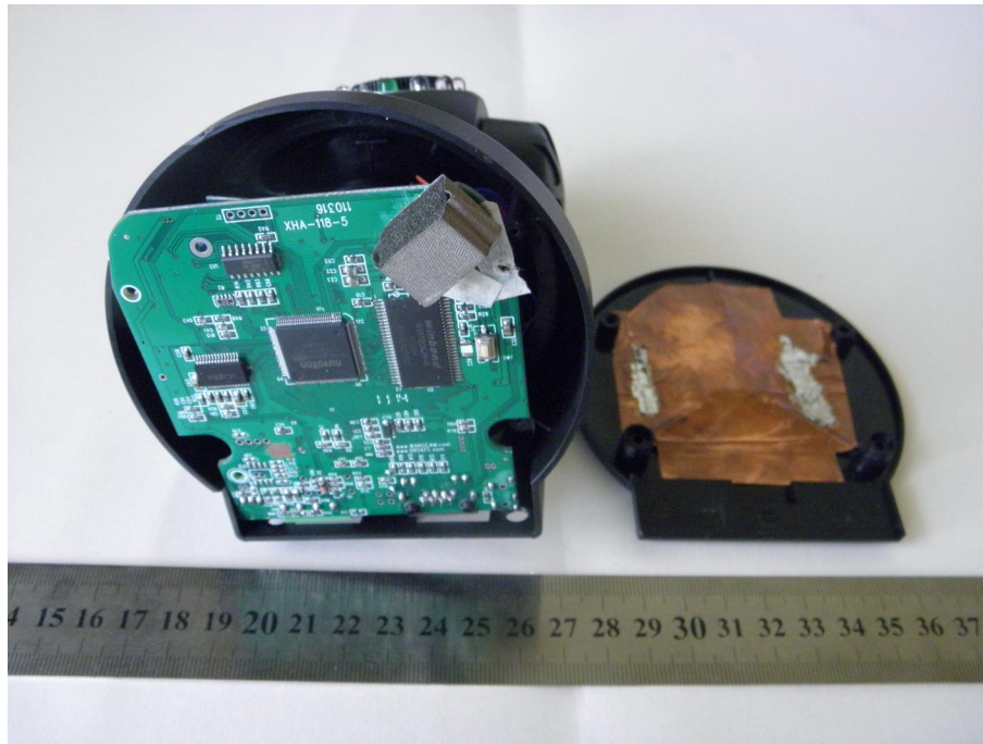
EUT-Internal View 1
