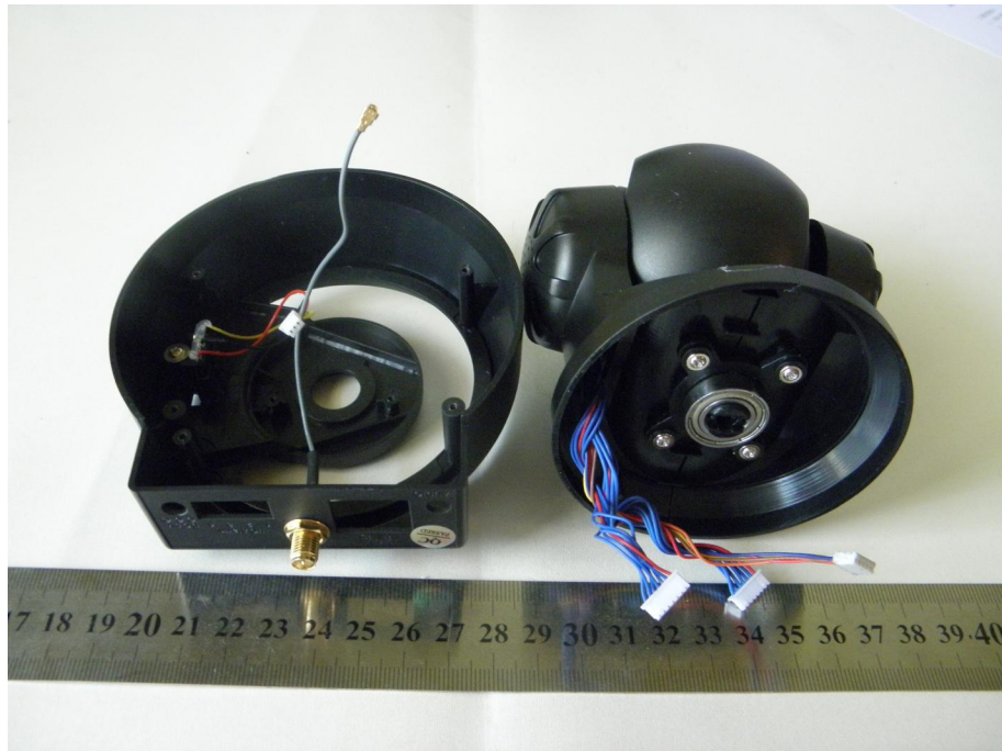
EUT-Internal View 3
