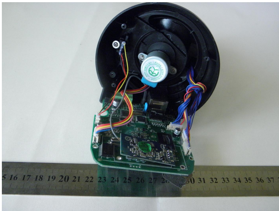
EUT-Internal View 2
