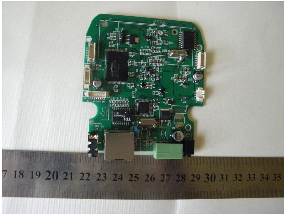
Main Board Top Wifi Module Off View
