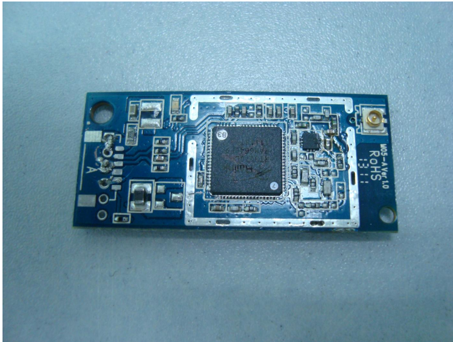
Wifi Module Top Shielding Off View
