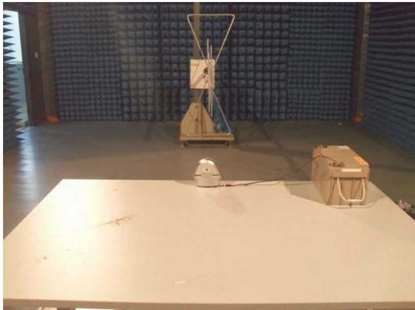
Below 1GHz
