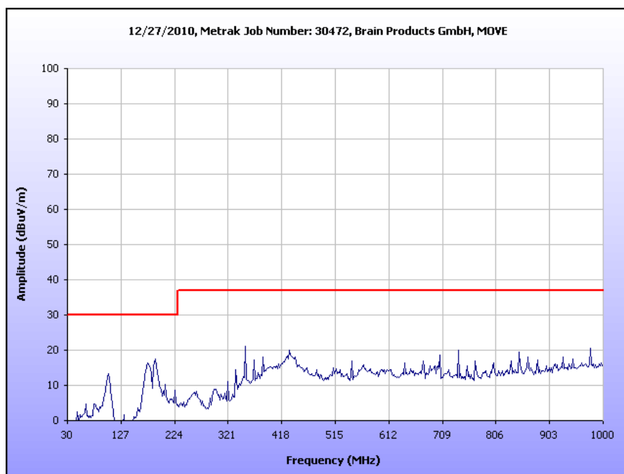
Plot 2. Radiated Emissions, Pre-Scan, 30 MHz – 1 GHz, ICES-003 Limits
