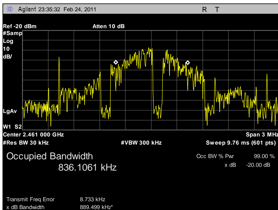
Plot 3. 99% Occupied Bandwidth
