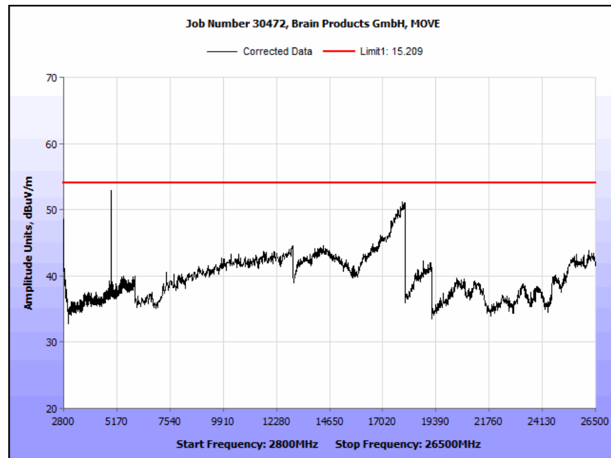
Plot 5. 2.8 – 26.5 GHz Scan
