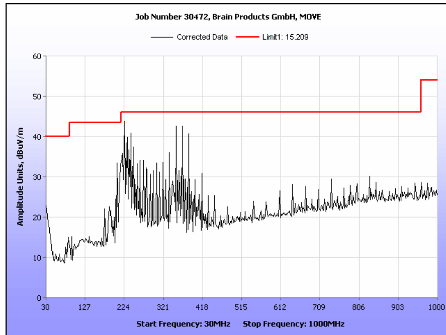
Plot 4. 30 – 1000 MHz Scan
