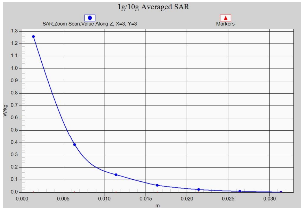
Fig. 1-1 Z-Scan at power reference point (2450 MHz)
