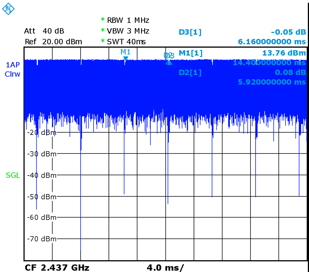
Picture 13.1 Duty factor plot for CH6
