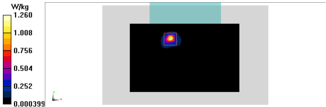
Fig.1 2450 MHz
