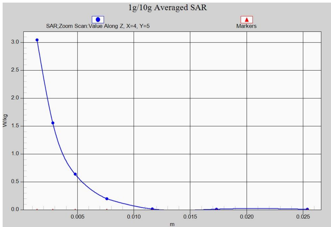
Fig. 26-1 Z-Scan at power reference point (5GHz)
