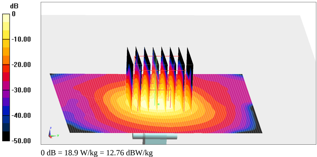
Fig.B.4 validation 5750MHz 100mW
