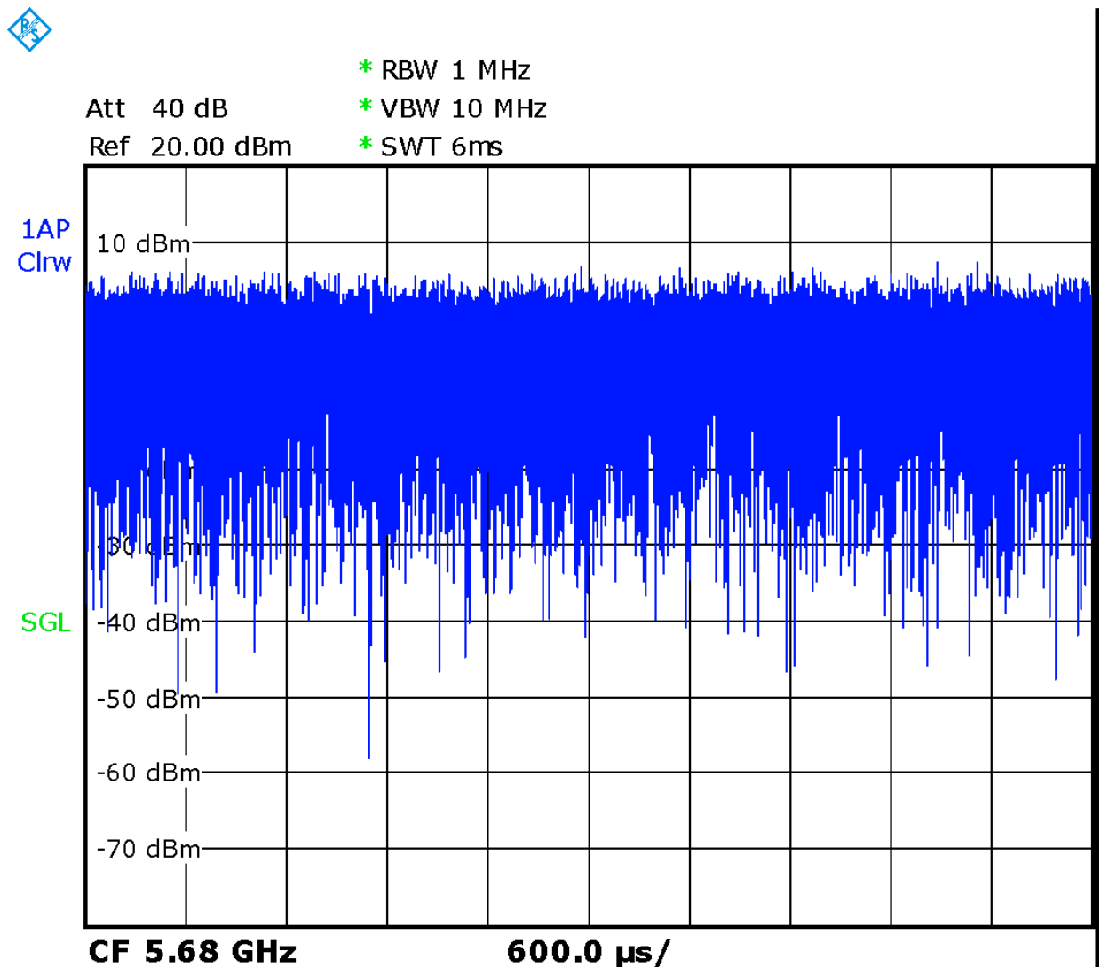
Picture 13.2-1 The plot of duty factor for U-NII-2C (Body)
