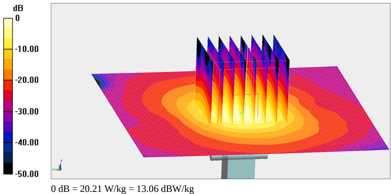
Fig.B.3 validation 5600MHz 100mW
