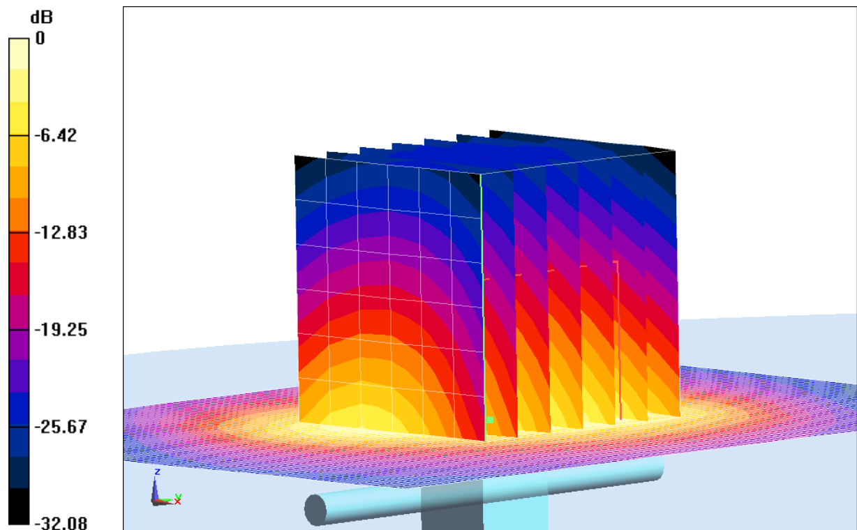
Fig.B.1 validation 2450 MHz 250mW
