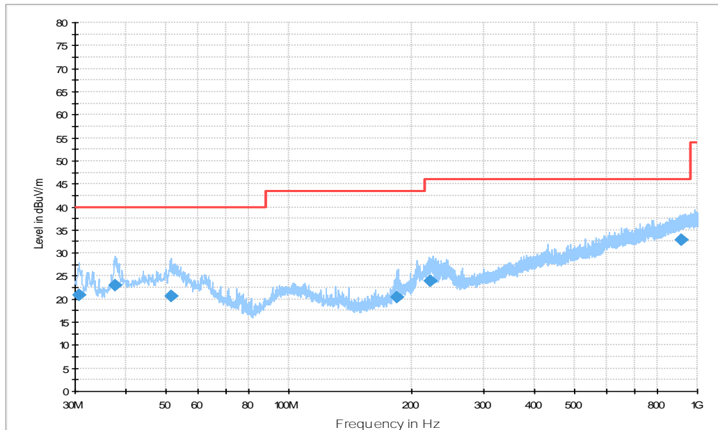
Figure A.4 Radiated Emission from 30MHz to 1GHz (Worst case)
