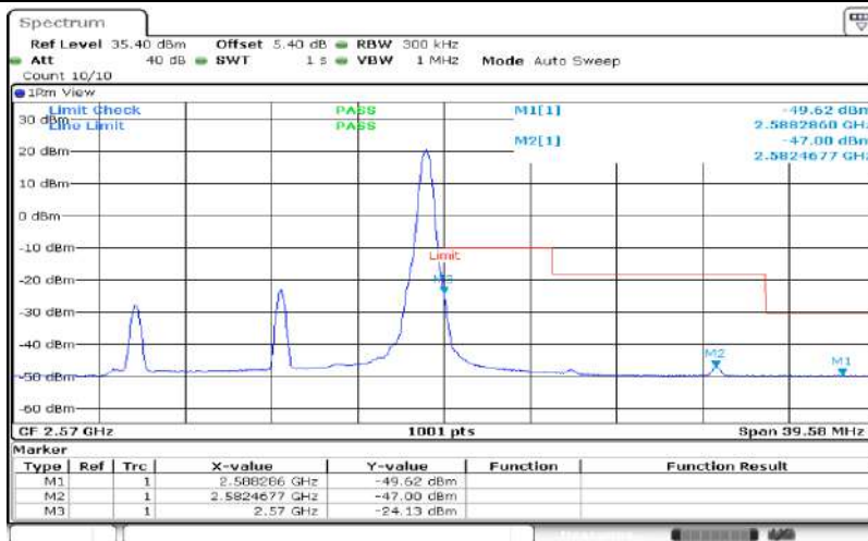
Band7-15MHz-16QAM-21375-1RB#74
