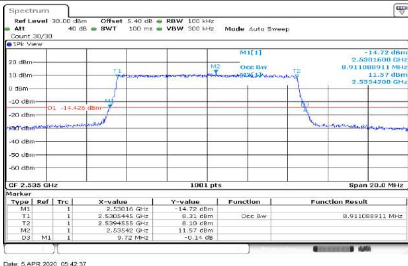
Band7-10MHz-16QAM-21400-50RB#0-8.911
