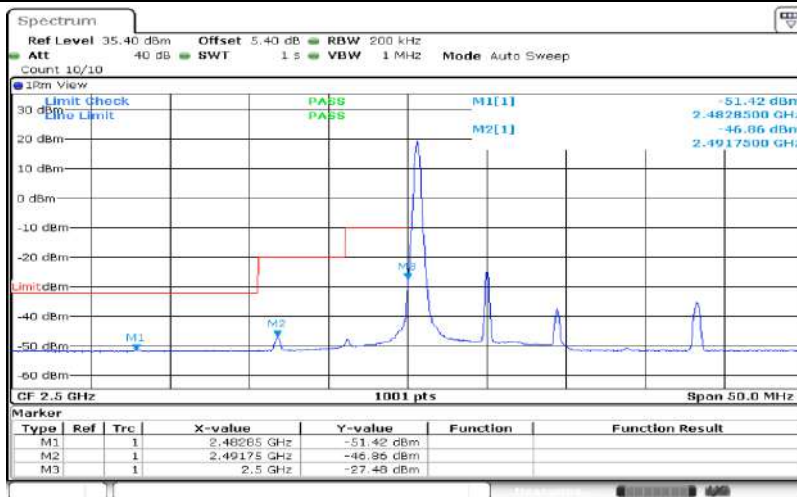
Band7-10MHz-64QAM-20800-1RB#0
