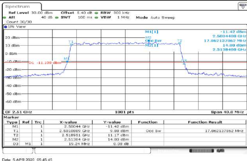
Band7-20MHz-QPSK-21100-100RB#0-17.862
