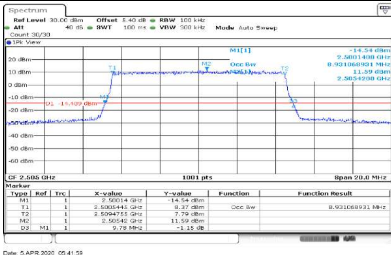
Band7-10MHz-16QAM-21100-50RB#0-8.911
