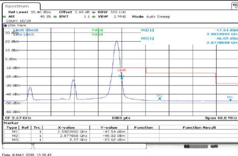
Band7-20MHz-64QAM-21350-100RB#0
