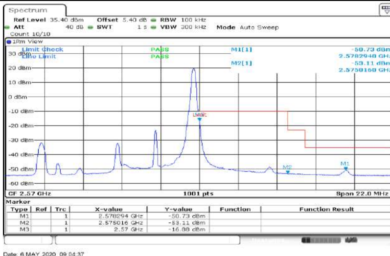
Band7-5MHz-QPSK-21425-25RB#0
