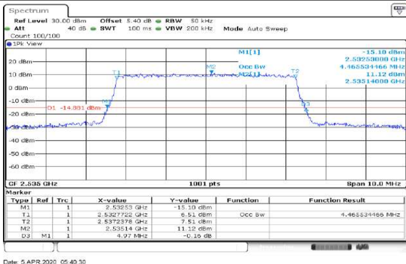
Band7-5MHz-64QAM-21425-25RB#0-4.466
