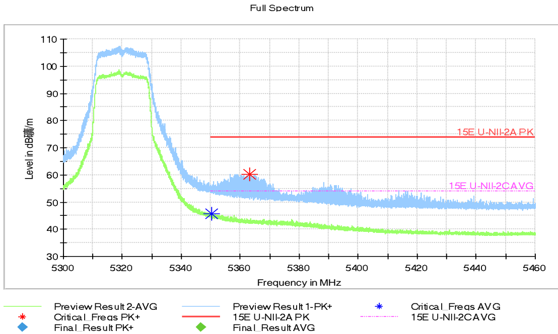
Fig.36 Band Edges (802.11n-HT20 Ch64, 5320MHz)
