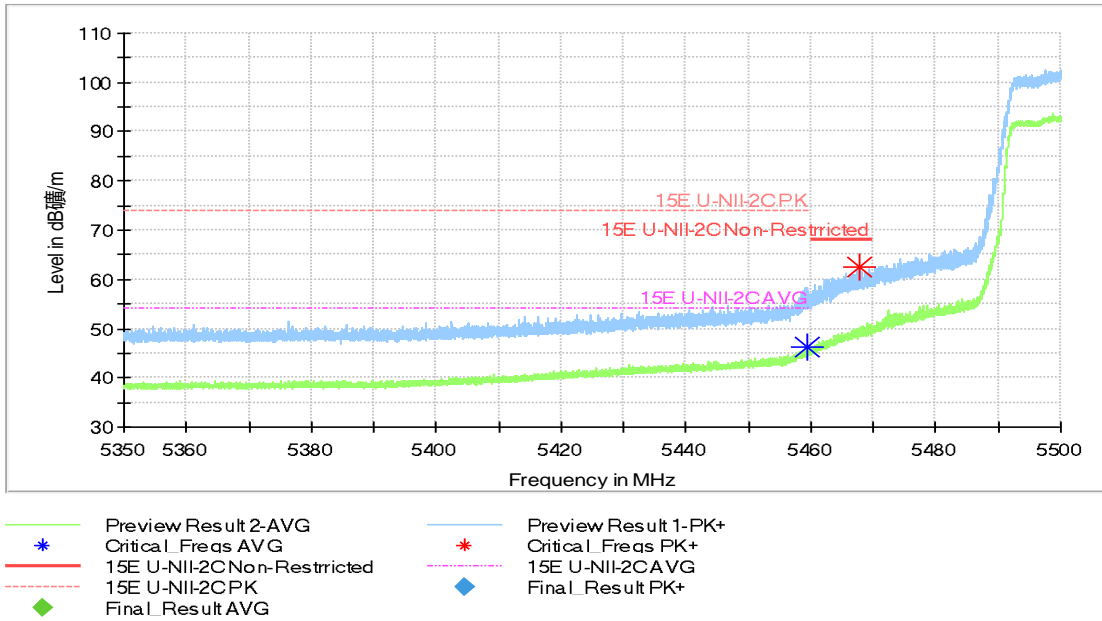
Fig.41 Band Edges (802.11n-HT40 Ch102, 5510MHz)
