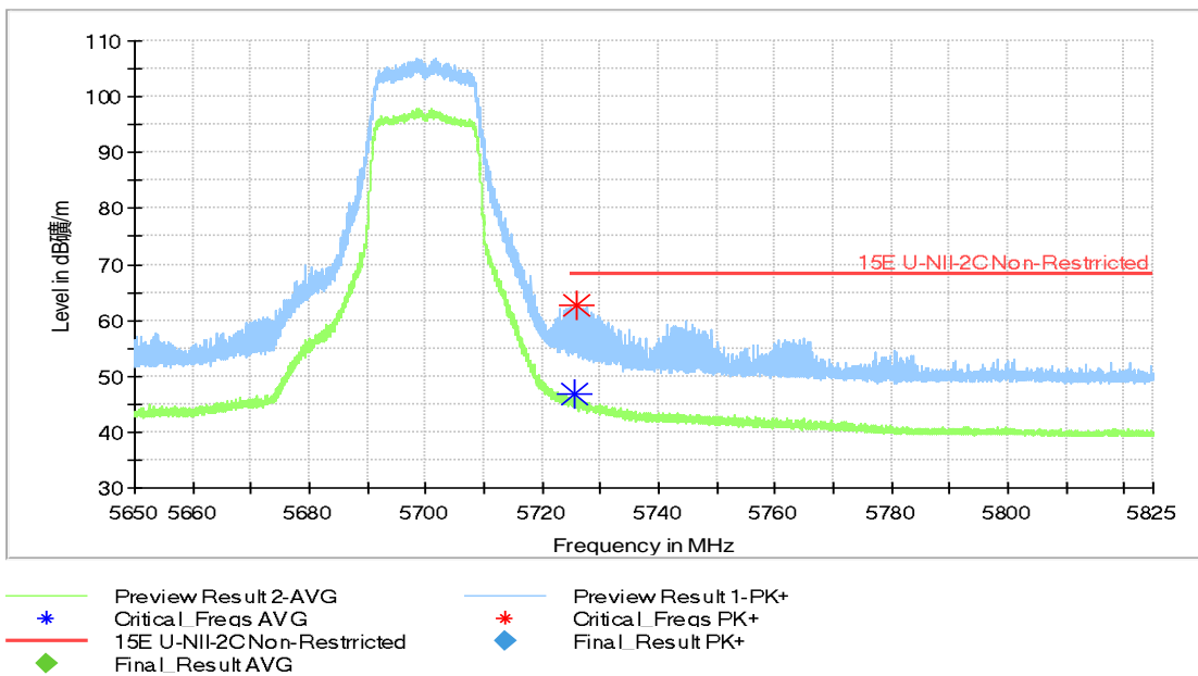
Fig.46 Band Edges (802.11ac-HT20 Ch140, 5700MHz)
