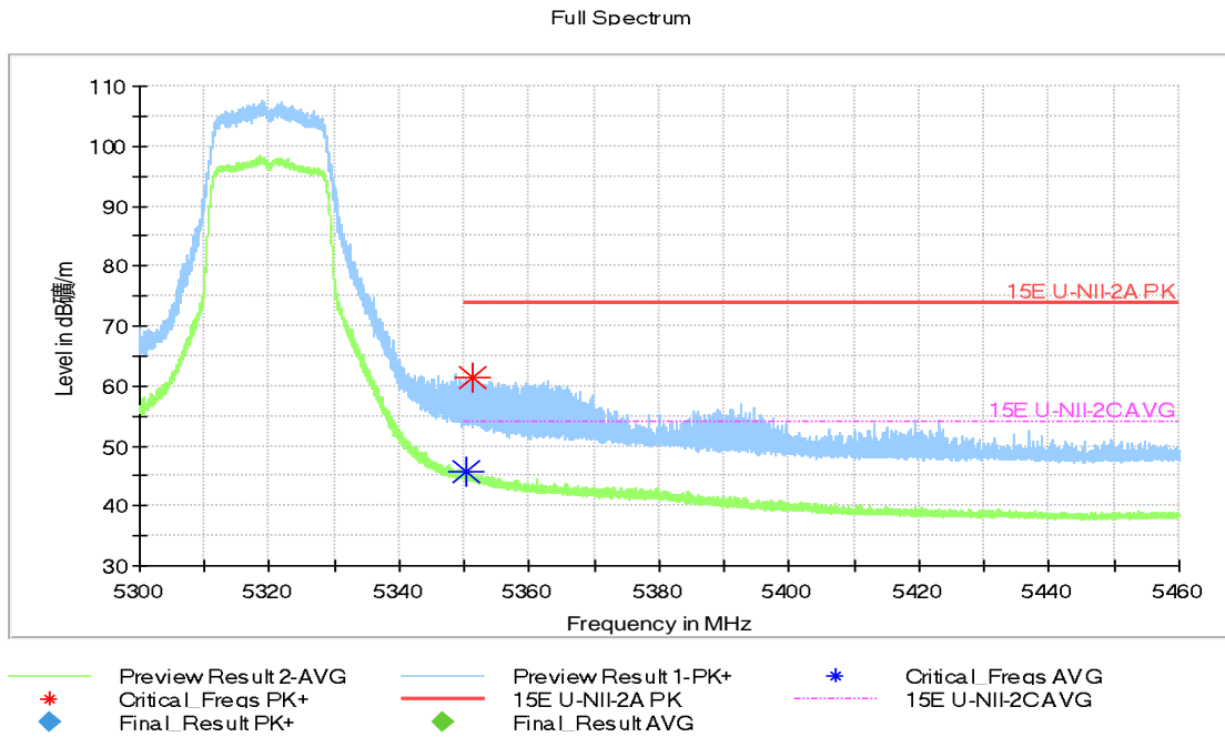
Fig.44 Band Edges (802.11ac-HT20 Ch64, 5320MHz)
