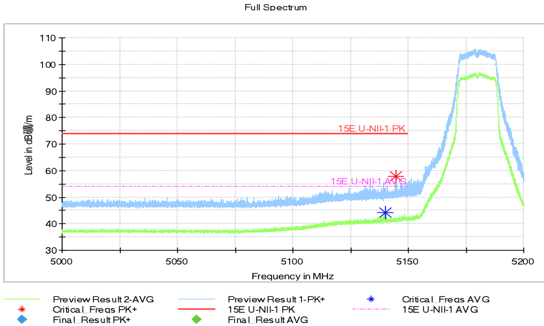
Fig.31 Band Edges (802.11a Ch36, 5180MHz)
