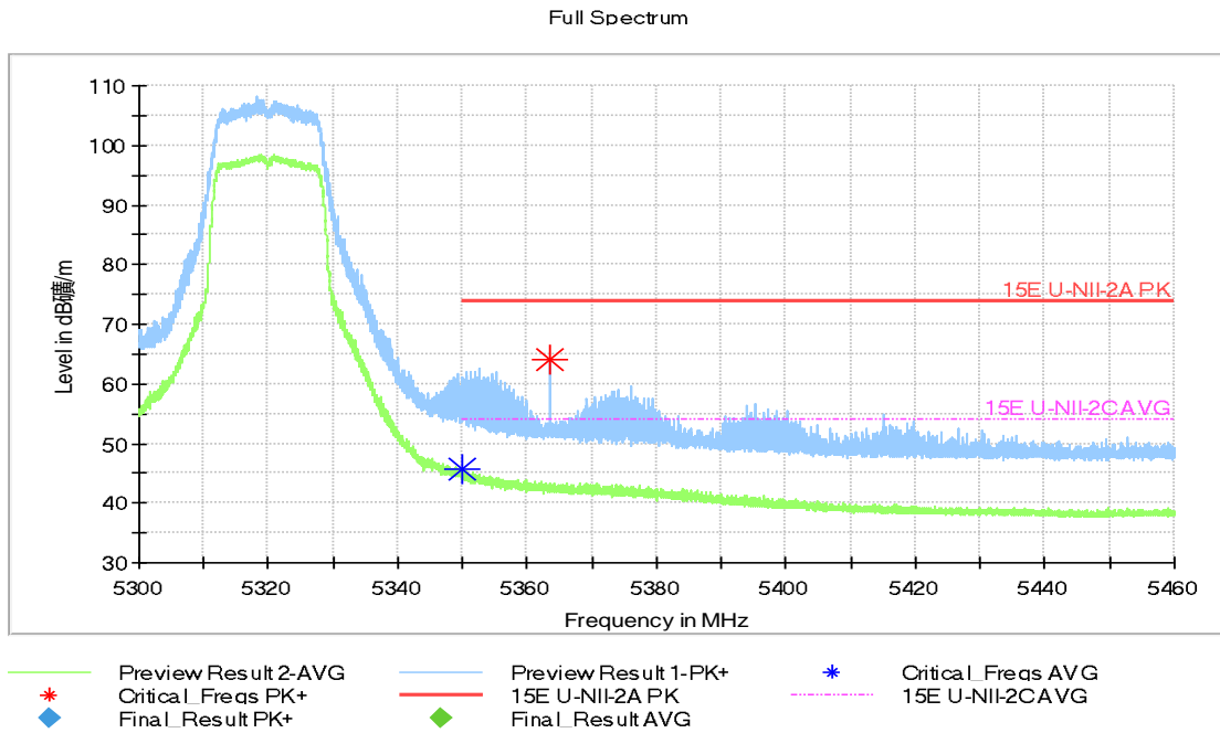
Fig.32 Band Edges (802.11a Ch64, 5320MHz)
