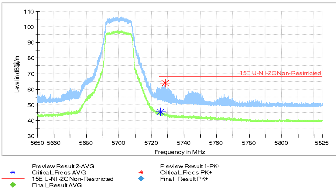
Fig.34 Band Edges (802.11a Ch140, 5700MHz)
