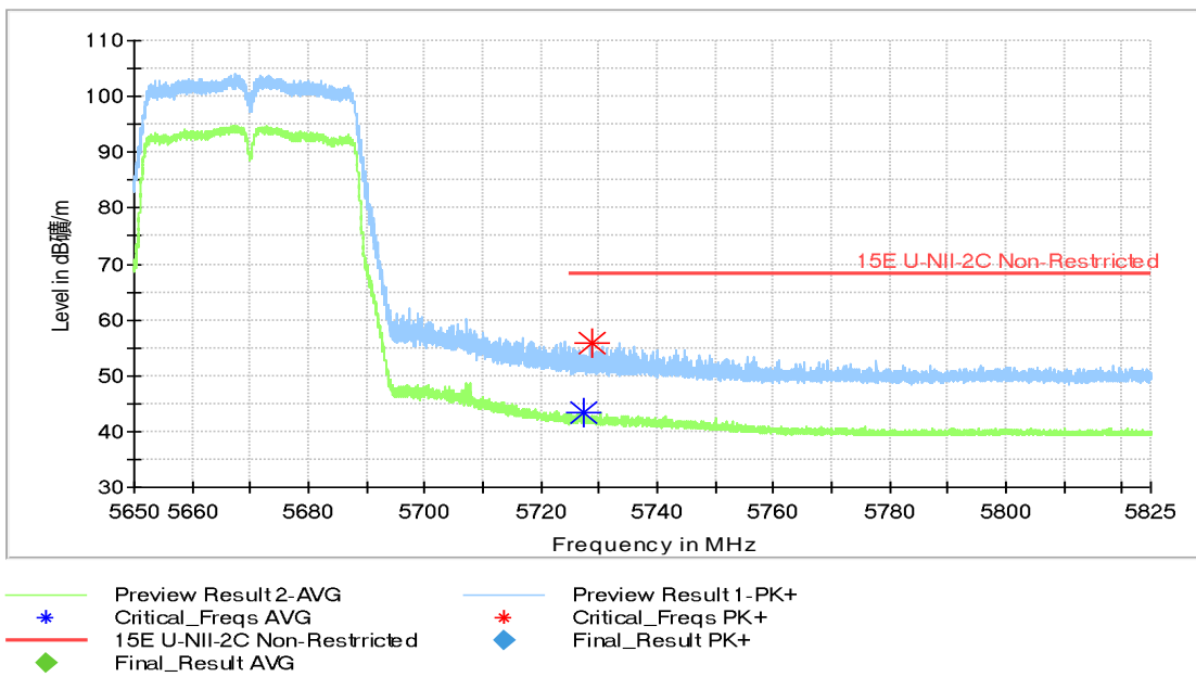
Fig.50 Band Edges (802.11ac-HT40 Ch134, 5670MHz)
