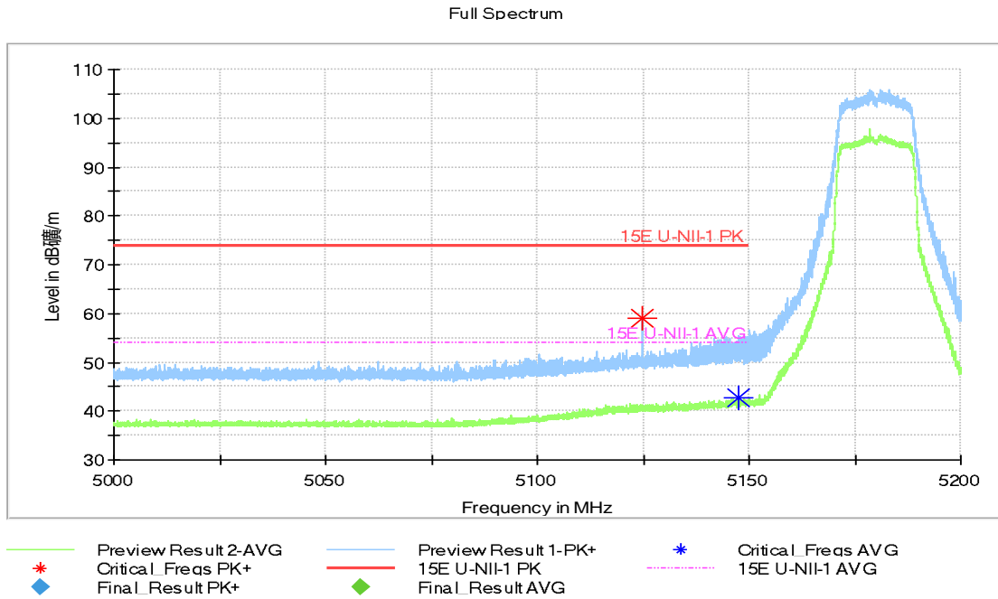
Fig.43 Band Edges (802.11ac-HT20 Ch36, 5180MHz)
