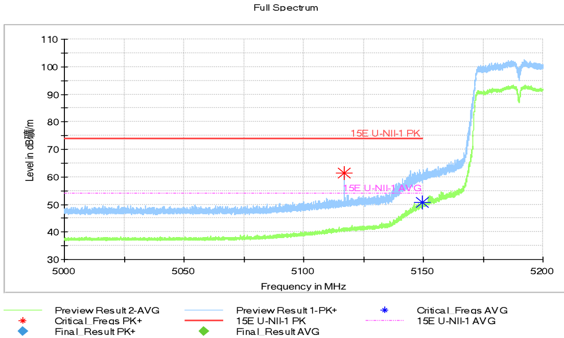
Fig.47 Band Edges (802.11ac-HT40 Ch38, 5190MHz)
