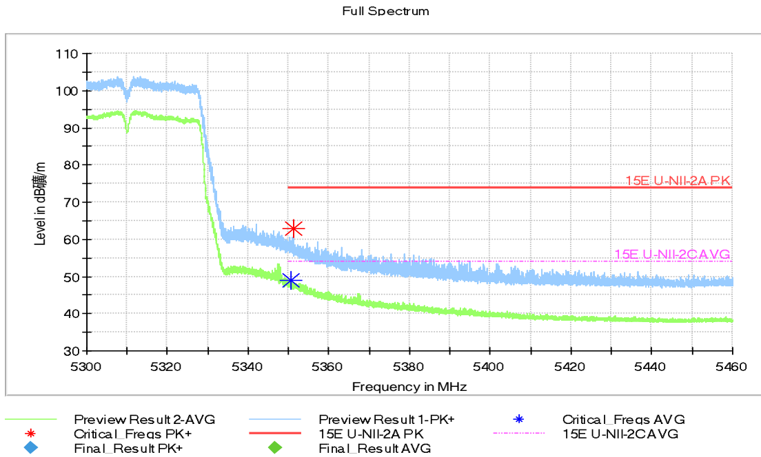
Fig.48 Band Edges (802.11ac-HT40 Ch62, 5310MHz)
