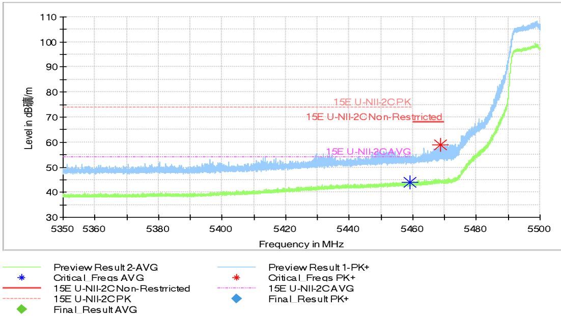
Fig.45 Band Edges (802.11ac-HT20 Ch100, 5500MHz)
