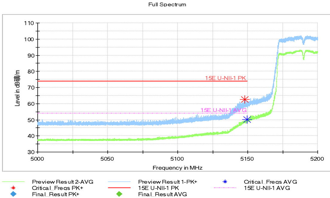
Fig.39 Band Edges (802.11n-HT40 Ch38, 5190MHz)
