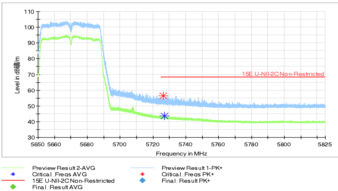
Fig.42 Band Edges (802.11n-HT40 Ch134, 5670MHz)
