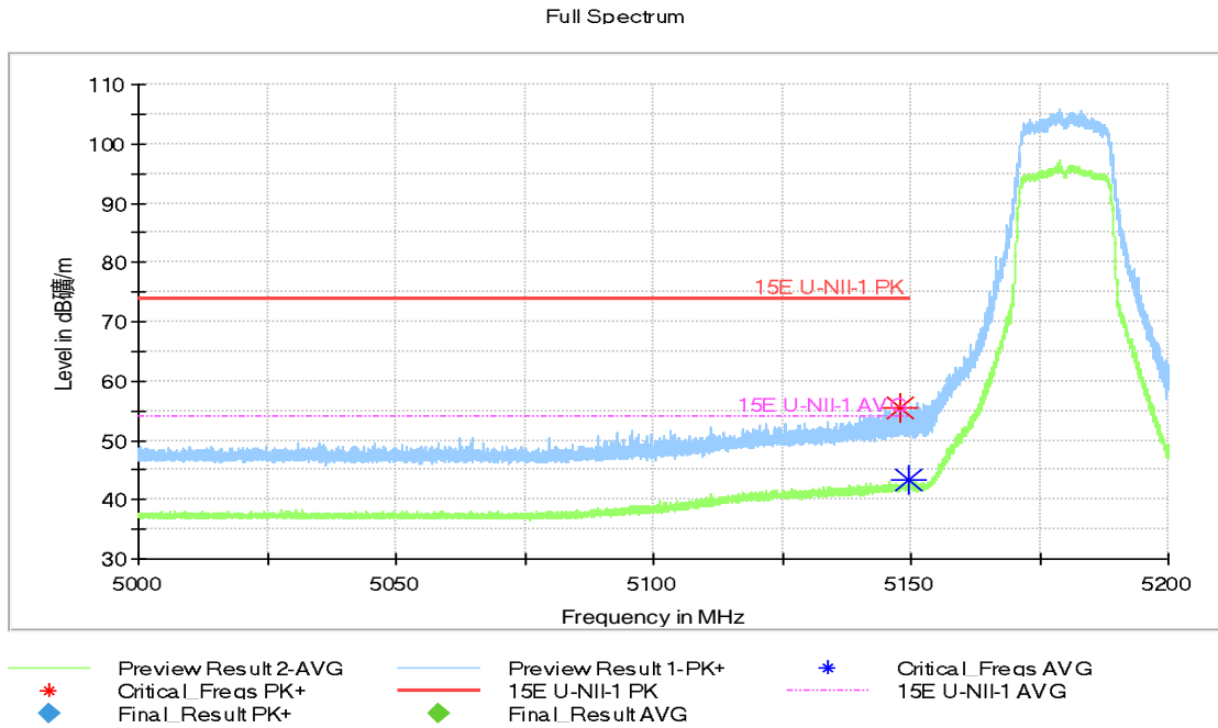
Fig.35 Band Edges (802.11n-HT20 Ch36, 5180MHz)
