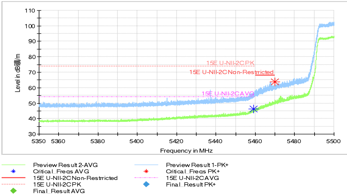
Fig.49 Band Edges (802.11ac-HT40 Ch102, 5510MHz)
