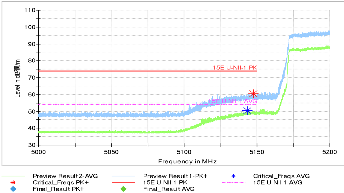
Fig.51 Band Edges (802.11ac-HT80 Ch42 , 5210MHz)
