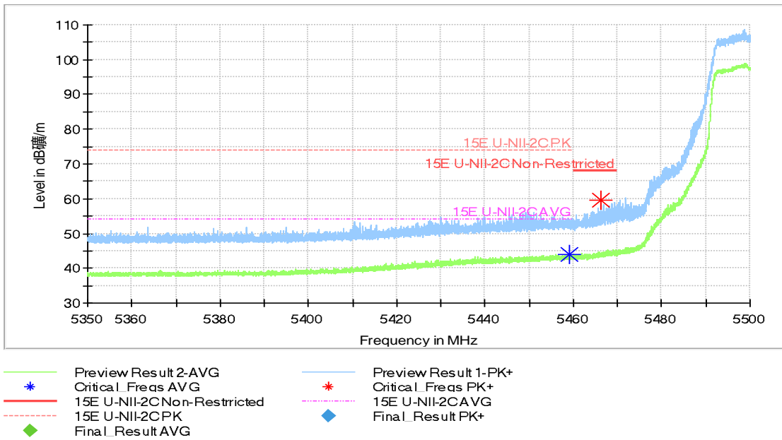
Fig.33 Band Edges (802.11a Ch100, 5500MHz)
