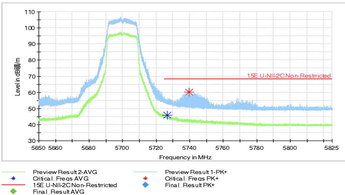
Fig.38 Band Edges (802.11n-HT20 Ch140, 5700MHz)
