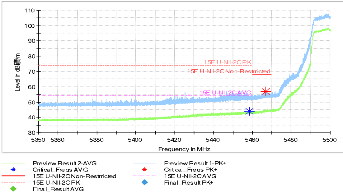
Fig.37 Band Edges (802.11n-HT20 Ch100, 5500MHz)
