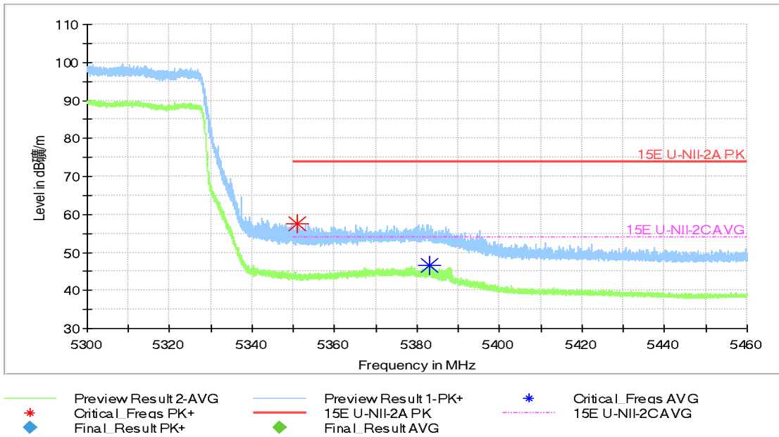
Fig.52 Band Edges (802.11ac-HT80 Ch58, 5290MHz)
