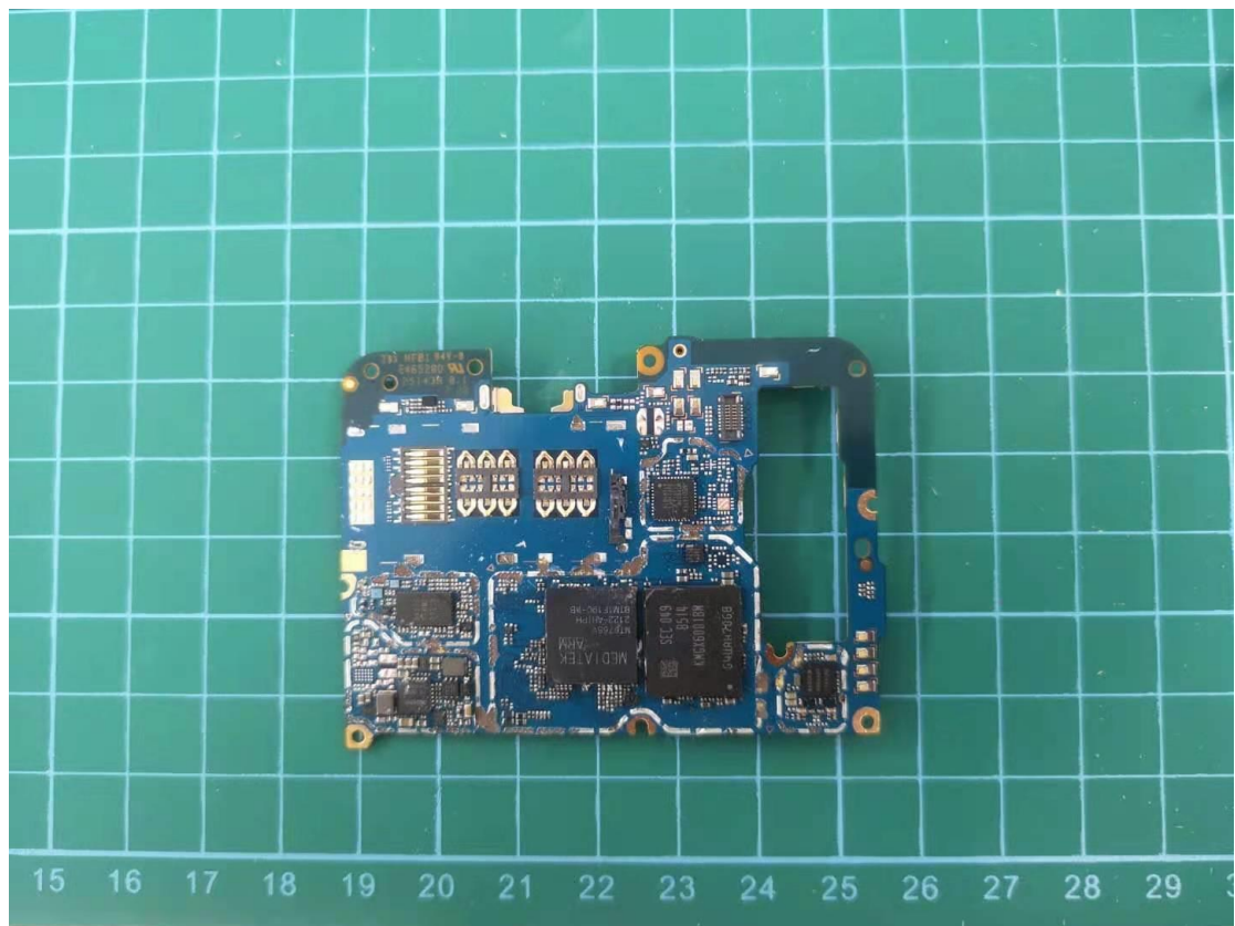
PCB07
