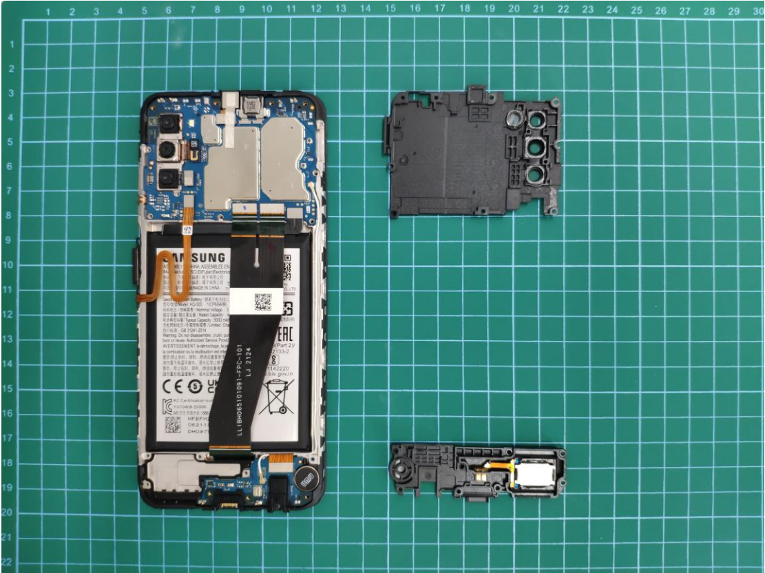
PCB02
