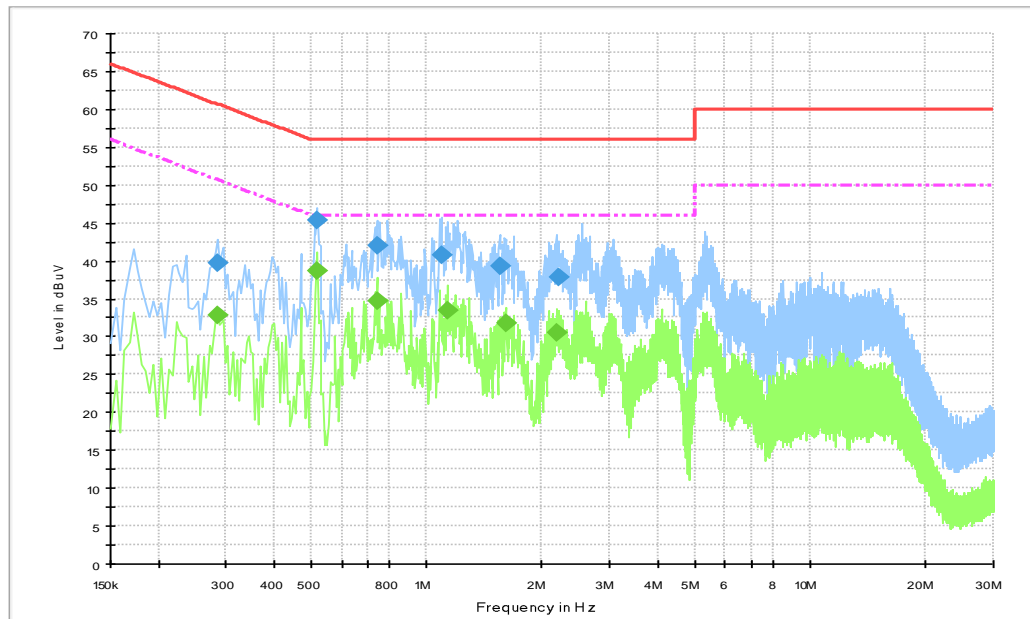
Fig.B.9.2 AC Powerline Conducted Emission-Iidle
